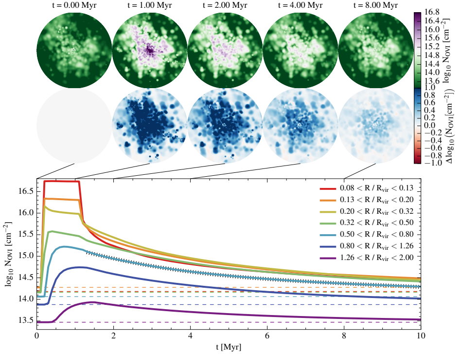
Figure 4.4: The evolution of the OV I column density around the M_* = 1.0 \times 10^{10} M_\odot galaxy at z = 3 , for an L/L_{\text{Edd}} = 1.0 AGN that is on for 1 Myr and off for 9 Myr (i.e. t_{\text{AGN}} = 10^6 yr and f_{\text{duty}} = 10\% ). The maps show the OV I column density (upper row) and difference in \log_{10} N_{\text{OV I}} with respect to t = 0 Myr (equation 4.5; lower row) at t = 0, 1, 2, 4, 8 Myr. The bottom panel shows the evolution of the median N_{\text{OV I}} (solid lines), as well as the equilibrium value at t = 0 Myr (dashed lines), in 7 logarithmic impact parameter intervals between 0.08 R_{\text{vir}} and 2 R_{\text{vir}} . The fit to N_{\text{OV I}}(R) at 0.5 < R/R_{\text{vir}} < 0.8 (black, dotted line) shows that the evolution of N_{\text{OV I}}(R) after the AGN turns off is well approximated by a sum of two exponential functions (equation 4.9).
