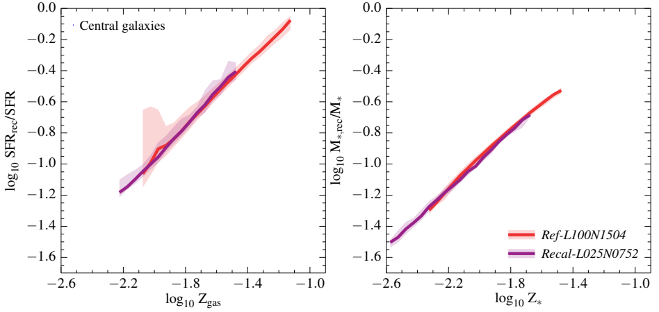
Figure 2.15: Test for numerical convergence of the \text{SFR}_{\text{rec}}/\text{SFR} - Z_{\text{gas}} (left) and M_{*,\text{rec}}/M_* - Z_* (right) relations (presented in Fig. 2.4) for central galaxies at z = 0 , comparing the fiducial EAGLE model ( Ref-L100N1504 ; red) and the high-resolution, recalibrated model ( Recal-L025N0752 ; purple). We only consider galaxies with stellar masses corresponding to at least 100 gas particles, at the respective resolution. In the left-hand panel, we only consider subhaloes with a non-zero SFR. The curves show the median value in each logarithmic metallicity bin of size 0.05 dex, if it contains at least 10 galaxies. The shaded regions mark the 10th to 90th percentile ranges. The \text{SFR}_{\text{rec}}/\text{SFR} - Z_{\text{gas}} and M_{*,\text{rec}}/M_* - Z_* relations are converged at the fiducial resolution over the whole metallicity range.
