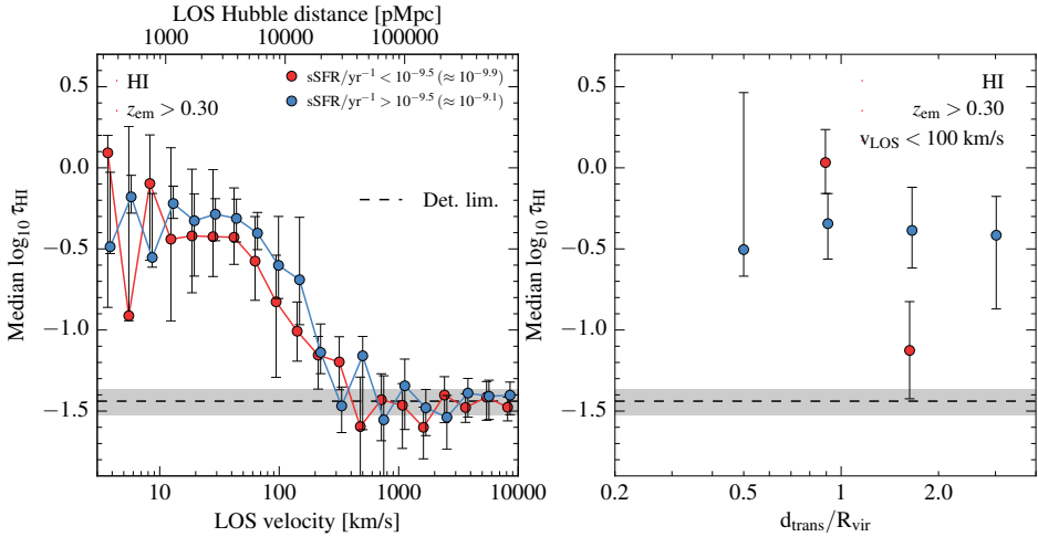
Figure 5.21: As Fig. 5.19, but showing the dependence of the median H I optical depth on the specific SFR of the galaxies. We compare samples of galaxies with \text{SFR}/M_{*} < 10^{-9.5} \text{ yr}^{-1} (red) and \text{SFR}/M_{*} > 10^{-9.5} \text{ yr}^{-1} (blue), with redshifts constrained to z_{\text{em}} > 0.30 . We only consider galaxies for which we could determine their SFR. Except for the significant increase of the H I absorption strength with increasing sSFR shown at 1.2 < d_{\text{trans}}/R_{\text{vir}} < 2.2 , we do not find evidence for a dependence of the absorption signal on sSFR.
