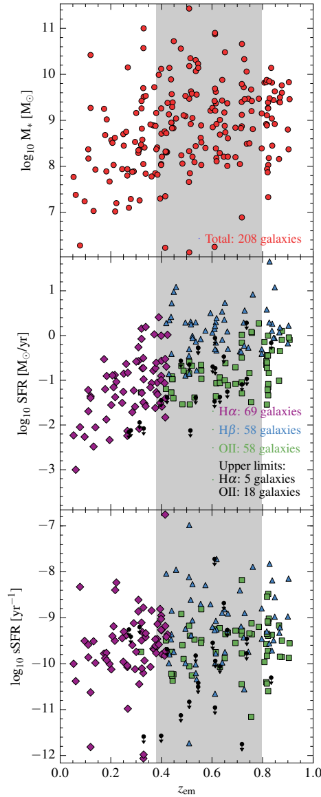
Figure 5.6: Galaxy stellar mass (top panel), SFR (middle panel) and specific SFR ( = \text{SFR}/M_* ; bottom panel) as a function of emission redshift. While the top panel shows the full sample, the middle and bottom panels only show galaxies for which we could obtain an estimate of the SFR, derived from the H \alpha (purple diamonds), H \beta (blue triangles) or OII (green squares) emission-line flux. The black symbols indicate upper limits. The grey shading indicates the redshift range in which we study the dependence of the OVI absorption strength on various galaxy properties, which we select in order to reduce the correlation between the absorption strength and properties other than the one under consideration (see Section 5.4.1 for details).
