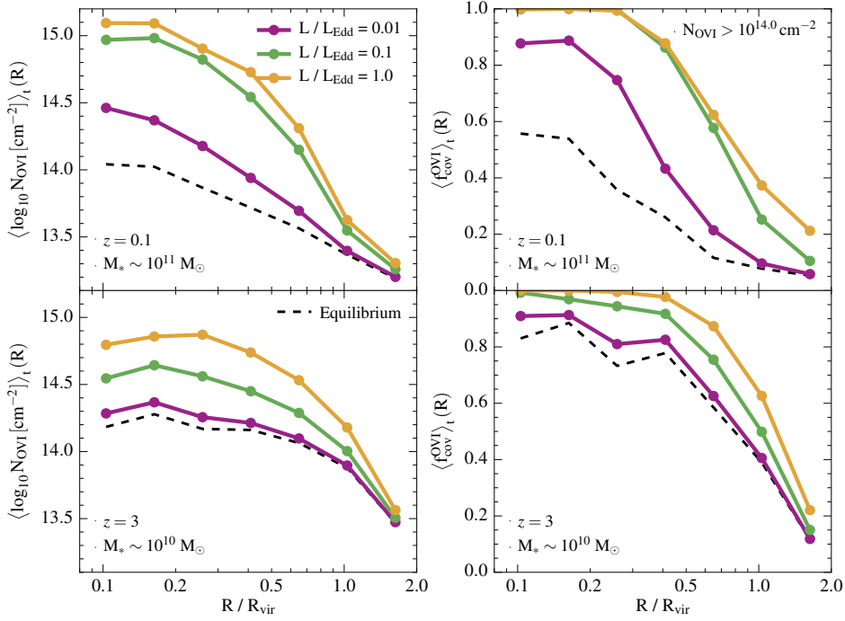
Figure 4.7: The impact of the AGN Eddington ratio on the fossil effect for the M_* \sim 10^{11} M_\odot galaxy at z = 0.1 (upper panels) and the M_* \sim 10^{10} M_\odot galaxy at z = 3 (lower panels). The plotted quantities, including the equilibrium profiles for the respective galaxies (black, dashed lines), are the same as in Fig. 4.6, but now we compare different Eddington ratios: L/L_{\text{Edd}} = 0.01 (purple), L/L_{\text{Edd}} = 0.1 (green) and L/L_{\text{Edd}} = 1.0 (yellow). We still adopt t_{\text{AGN}} = 10^6 yr and f_{\text{duty}} = 10\% . For a sufficiently high AGN luminosity, as in the case of the M_* \sim 10^{11} M_\odot galaxy at z = 0.1 , the increase in \langle \log_{10} N_{\text{OVI}} \rangle_t(R) and \langle f_{\text{OVI}} \rangle_t(R) with respect to equilibrium depends on the adopted luminosity in a non-linear way. This is related to the increase in the photoionization rate from OVI to higher states as well as from OV to OVI.
