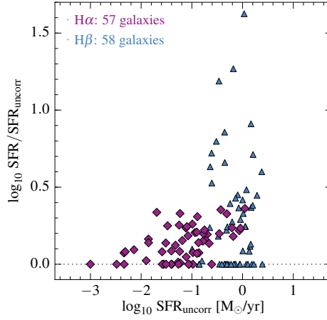
Figure 5.8: The size of the dust correction as a function of the uncorrected SFR for the 115 galaxies for which the H\alpha flux (purple) or the H\beta flux (blue) could be corrected for dust extinction (using the H\alpha/H\beta and H\beta/H\gamma ratios, respectively). The largest dust corrections are generally associated with the galaxies with the highest uncorrected SFRs.
