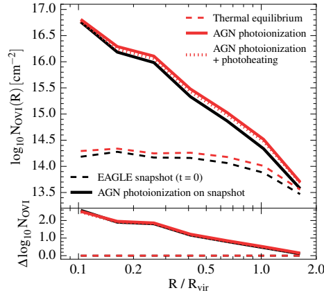
Figure 4.12: The impact of AGN photoheating on the OVI column density profile of the M_* = 1.0 \times 10^{10} M_\odot galaxy at z = 3 , adopting a continuously radiating AGN with L/L_{\text{Edd}} = 0.1 . The red lines correspond to an artificial state with the T < 10^5 K gas in thermal and ionization equilibrium without AGN radiation (dashed) and in a new thermal and ionization equilibrium in the presence of the AGN radiation, where the gas temperature was kept fixed (solid) or allowed to vary (dotted). The temperature of the T > 10^5 K gas was kept fixed to the one in the EAGLE snapshot in both cases. For comparison, the black lines show the profile as calculated directly from the EAGLE snapshot assuming ionization equilibrium (dashed), and the profile corresponding to the new ionization equilibrium due to AGN photoionization using the snapshot temperatures (solid). The bottom panel indicates the difference in \log_{10} N_{\text{OVI}} with respect to the dashed lines of the respective colour. The increase in N_{\text{OVI}} with respect to thermal equilibrium (red, dashed line) due to AGN photoheating and photoionization (red, dotted line) is only \lesssim 0.05 dex lower than the increase due to AGN photoionization (red, solid line), indicating that AGN photoheating does not have a significant impact on N_{\text{OVI}} .
