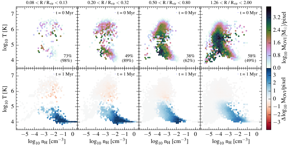
Figure 4.5: The distribution of OVI mass, M_{\text{OVI}} , in T – n_{\text{H}} space for different impact parameter intervals for the M_* \sim 10^{10} M_{\odot} galaxy at z = 3 . The upper row shows the equilibrium distribution at t = 0 Myr, while the lower row shows the difference in \log_{10} M_{\text{OVI}} per pixel between t = 1 Myr (after the AGN has been on for 1 Myr) and t = 0 Myr. In each of the upper panels, the top (bottom) percentage indicates the OVI mass fraction at T > 10^5 K per impact parameter (3D radial distance) bin with boundaries given at the top. The AGN predominantly affects the photoionized gas at T \lesssim 10^5 K: the enhancement of OVI in this temperature regime is what drives the evolution of N_{\text{OVI}} .
