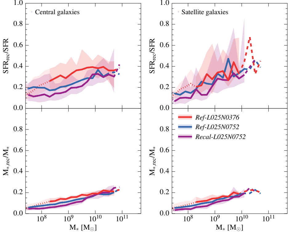
Figure 2.14: Test for numerical convergence of the SFR_{rec}/SFR - M_* (top) and M_{*,rec}/M_* - M_* (bottom) relations (presented in Figs. 2.6 and 2.7) for central (left) and satellite (right) galaxies at z = 0 , comparing an EAGLE simulation with the fiducial resolution ( Ref-L025N376 ; red) to two EAGLE simulations with eight times higher mass resolution, with ( Recal-L025N0752 ; purple) and without ( Ref-L025N0752 ; blue) recalibrated subgrid feedback parameters. All three simulations were run in volumes of size L = 25 cMpc. The curves and shaded regions have the same meaning as in Fig. 2.6, but for clarity we only show the 10th to 90th percentile range for the Ref-L025N376 and Recal-L025N752 simulations. For galaxies with M_* \gtrsim 10^{9.8} M_\odot , SFR_{rec}/SFR and M_{*,rec}/M_* as a function of stellar mass are reasonably well converged. For galaxies with M_* \lesssim 10^{9.8} M_\odot , the fiducial EAGLE simulation likely overpredicts the SFR and stellar mass contributed by recycling, by at most a factor of \sim 2 ( \sim 0.3 dex) at M_* \sim 10^9 M_\odot .
