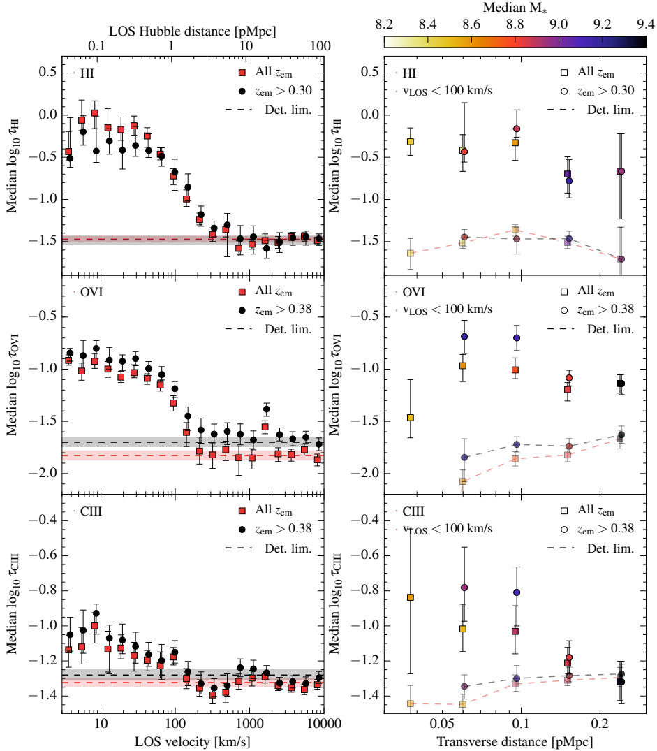
Figure 5.9: The median pixel optical depth of H I (top), O VI (middle) and C III (bottom) as a function of LOS velocity (left) and transverse distance (right). While the squares show the absorption signal for the full sample of galaxies, the circles (which, for clarity, have been offset horizontally by 0.02 dex and 0.006 dex in the left- and right-hand panels, respectively) show the signal for galaxies in a restricted redshift range. Along the LOS direction, the median \log_{10} \tau_Z is calculated in 20 logarithmic bins between v_{\text{LOS}} = 3 km/s and v_{\text{LOS}} = 10,000 km/s, where the corresponding absolute LOS Hubble distance, assuming z = 0.5 and pure Hubble flow, is indicated at the top. The horizontal dashed lines show the detection limit, calculated as the median \log_{10} \tau_Z at 15,000 < v_{\text{LOS}} < 25,000 km/s from the galaxies contributing to the profile of the respective colour. Along the transverse direction, the median \log_{10} \tau_Z is calculated, using only pixels at v_{\text{LOS}} < 100 km/s, in 5 logarithmic bins between d_{\text{trans}} = 30 pkpc and d_{\text{trans}} = 300 pkpc, where we only show bins containing at least three galaxies. The points are colour-coded by the median galaxy stellar mass in each bin. The detection limit is calculated separately for each transverse distance bin, and shown by the light-coloured symbols connected by dashed lines. In all panels, the error bars (and shaded regions) show the 1\sigma confidence interval on the median optical depth.
