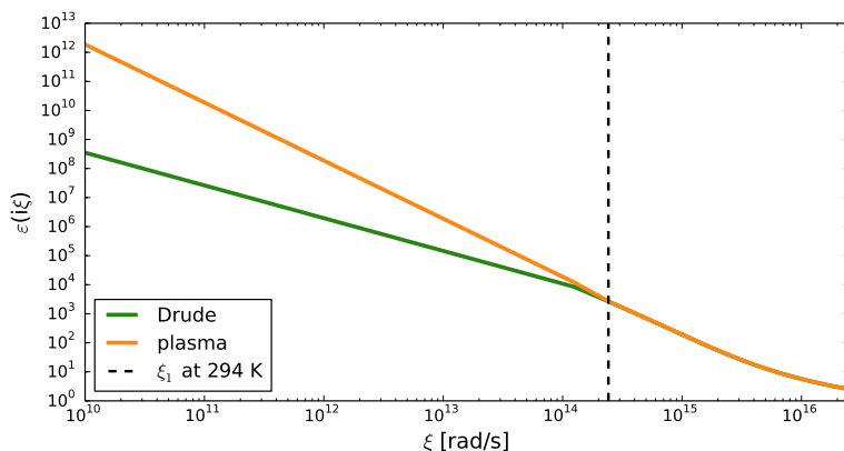
Figure 5.3: Dielectric permittivity of gold at imaginary frequencies i\xi as a function of \xi . For frequencies above 1.9 \times 10^{14} rad/s optical data are available, the extrapolation to lower frequencies was obtained with the values \Omega_p = 9.0 eV and \gamma = 0.035 eV. It is clear that the Drude and plasma models deviate at lower frequencies. The first order Matsubara frequency at room temperature is also indicated.
