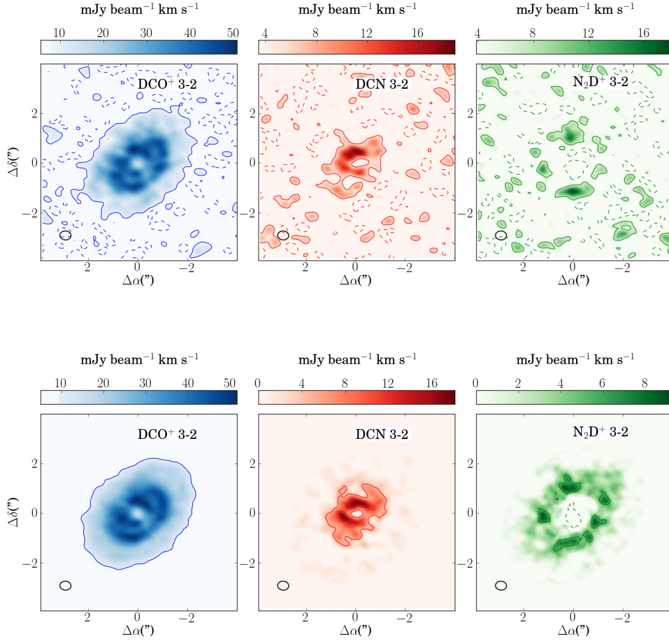
Figure 5.1: Integrated intensity maps of DCO + , N 2 D + , and DCN with (lower panels) and without (upper panels) a Keplerian mask as explained in Appendix 5.A. The resulting synthesized beams of 0 h :53×0 h :42 for DCO + and DCN, and 0 h :50×0 h :39 for N 2 D + , with a beam position angle of 90°, using natural weighting are shown at the lower left of each map. Contours are 1 \sigma levels, where \sigma is estimated as the rms of an emission free region in the sky.
