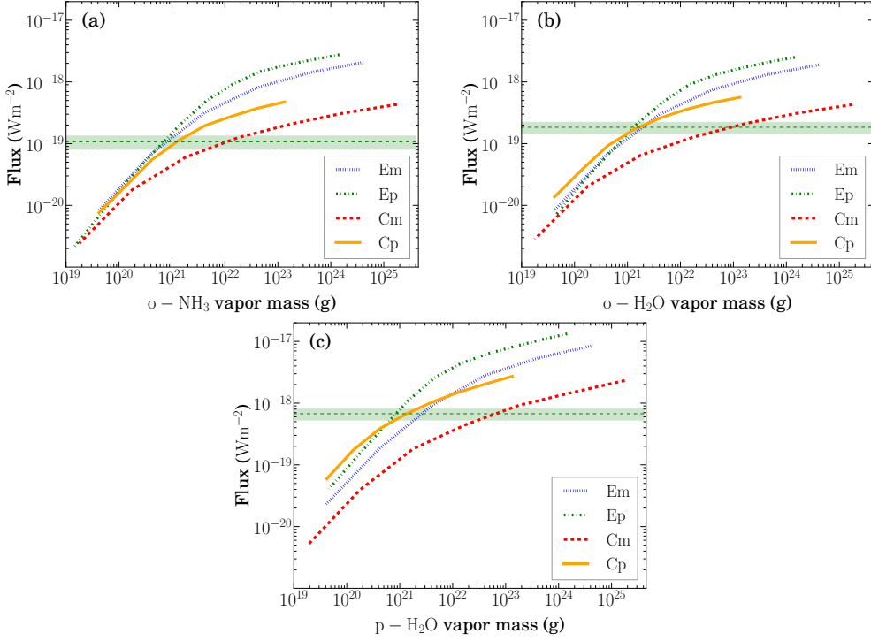
Figure 3.4: Panels (a), (b) and (c) show the LIME (Brinch & Hogerheijde 2010) output of the total line fluxes of ortho- \text{NH}_3 , ortho- \text{H}_2\text{O} , and para- \text{H}_2\text{O} , respectively, as a function of the total water vapor mass. The blue, green, red, and yellow curves correspond to the Em, Ep, Cm, and Cp models, respectively. The dashed lines and horizontal green bar show the observed line fluxes and their 3\sigma ranges, with sigma having two sources of noise added in quadrature; the systematic error of the observations, estimated to be about 20% of the total flux, and the rms of the spectra.
