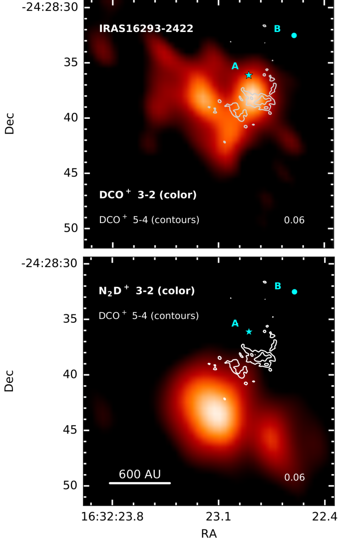
Figure 3: Intensity integrated maps of DCO + 3-2 (top) and N 2 D + 3-2 (bottom) observed with the SMA, overlaid with DCO + 5-4 (contours) observed with ALMA. Contours are the same as in Fig. 2. The positions of IRAS 16293-2422 A and B are indicated with a star and circle, respectively. Both DCO + transitions match spatially, and N 2 D + is located beyond the extent of the DCO + emission. Note the different center of this figure compared to Fig. 2.
