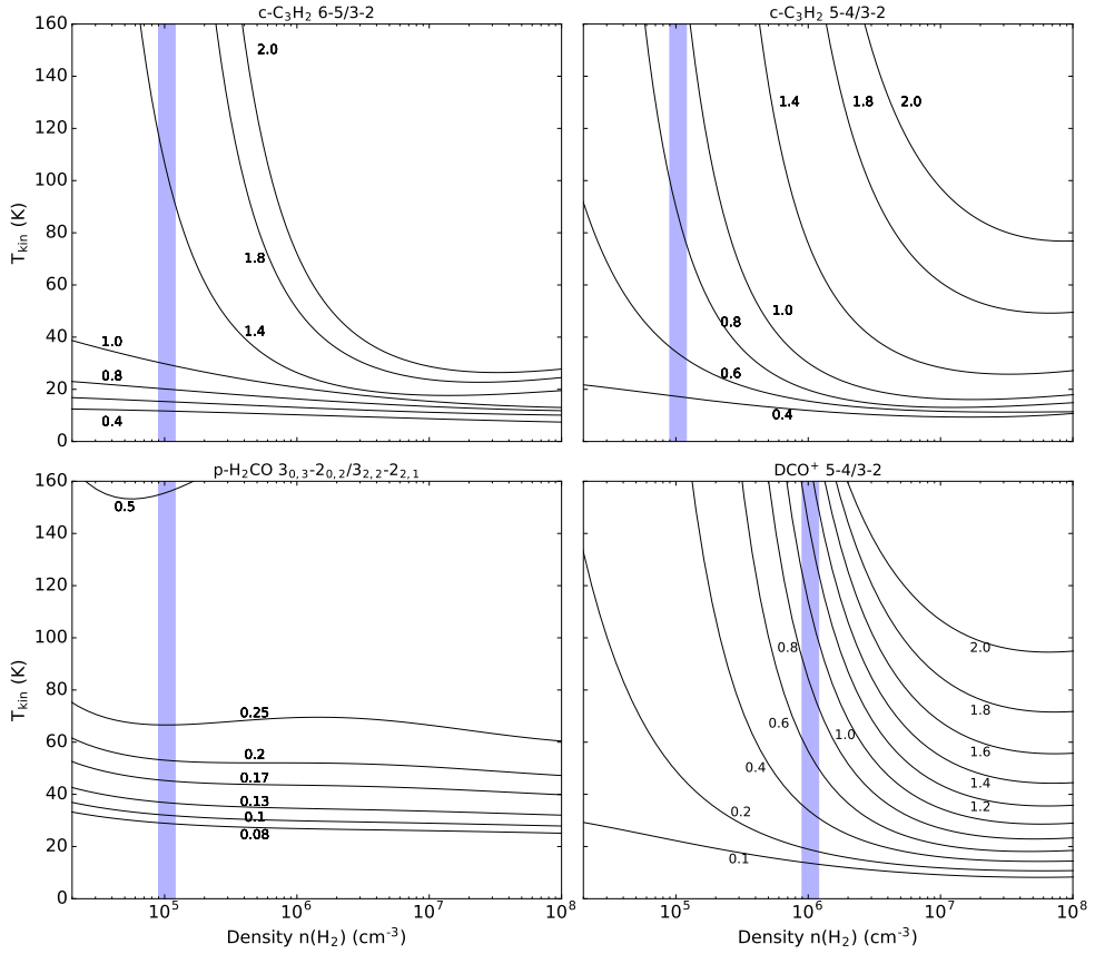
Figure 7: Calculated line ratios for c\text{-C}_3\text{H}_2 6\text{-}5 / 3_{0,3}\text{-}2_{2,1} (left) and 5_{1,4}\text{-}4_{2,3} / 3_{3,0}\text{-}2_{2,1} (center), and \text{H}_2\text{CO} 3_{0,3}\text{-}2_{0,2} / 3_{2,2}\text{-}2_{2,1} . The black lines show the modelled ratios assuming a column density of 10^{12} \text{ cm}^{-2} . Lines between the 0.4 and 1.0 ratios of c\text{-C}_3\text{H}_2 , are spaced evenly in steps of 0.2. The shaded area indicates the adopted \text{H}_2 density for the temperature calculations.
