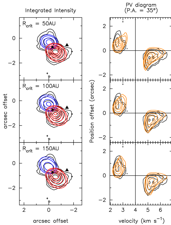
Figure 8: Infall plus Keplerian case for three different R_{\text{crit}} . The best fit model (color) to the data (black) is obtained as R_{\text{crit}} approaches R_{\text{out}} . Right panels show PV diagrams along the disk's major axis (P.A. = 35°). All contours and the model at R_{\text{crit}} = 150\text{ AU} are the same as in Fig. 6.
