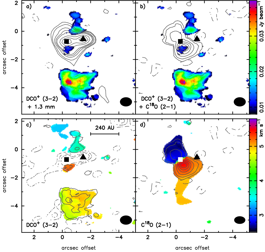
Figure 1: DCO + compared with continuum and C 18 O toward VLA1623A & B, marked with a square and triangle, respectively. The black ellipse shows the synthesized beam. Intensity integrated DCO + (color-scale) with (a) 1.3mm continuum and (b) C 18 O. DCO + peaks at 0.0433 Jy beam -1 km s -1 . Contours are in steps of 3, 5, 10, 15, 20, 40, 60 and 78σ with σ = 1 mJy beam -1 for 1.3 mm continuum, and -5, -3, 3, 5, 10, 15, 20 and 25σ with σ = 13 mJy beam -1 km s -1 for C 18 O. Velocity map (moment 1, color-scale) for (c) DCO + and (d) C 18 O overlaid with the corresponding intensity integrated map (contours). Contours are in steps of -10, -7, -4, 4, 7, 10 and 11σ with σ = 3 mJy beam -1 km s -1 for DCO + , and the same as in (b) for C 18 O.
