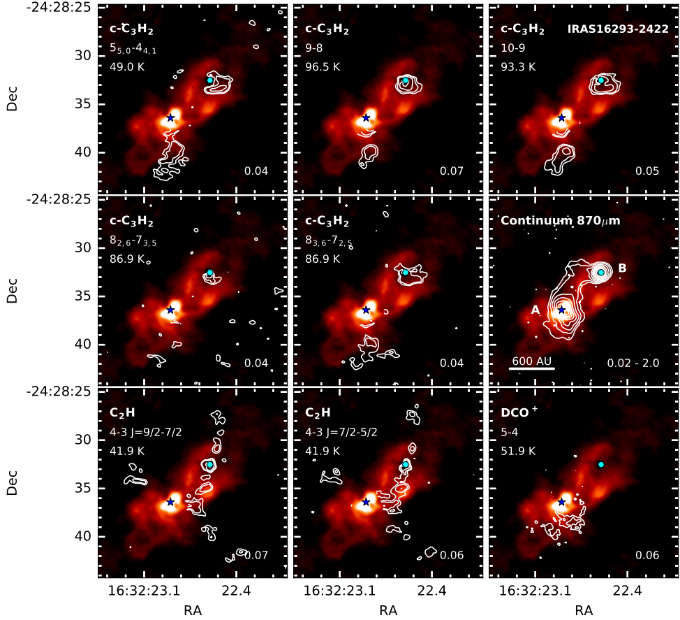
Figure 2: Intensity integrated maps (contours) of c\text{-C}_3\text{H}_2 , \text{C}_2\text{H} , \text{DCO}^+ and continuum towards IRAS 16293-2422. \text{H}_2\text{CO} 5-4 is shown in color-scale. Contours show the respective lines in steps of 2, 3, 5, 20 and 60\sigma , with \sigma ( \text{Jy beam}^{-1} \text{ km s}^{-1} ) indicated in the lower right of each panel. For continuum, the levels are logarithmically spaced between 0.02 and 2 \text{Jy beam}^{-1} , and highlight the ridge that spans between sources A and B. The positions of IRAS 16293-2422 A and B are indicated with a star and circle, respectively. For the c\text{-C}_3\text{H}_2 and \text{C}_2\text{H} panels, the emission centered on A is contamination from other molecule(s) and is masked out in a radius of 2'' from the position of A.
