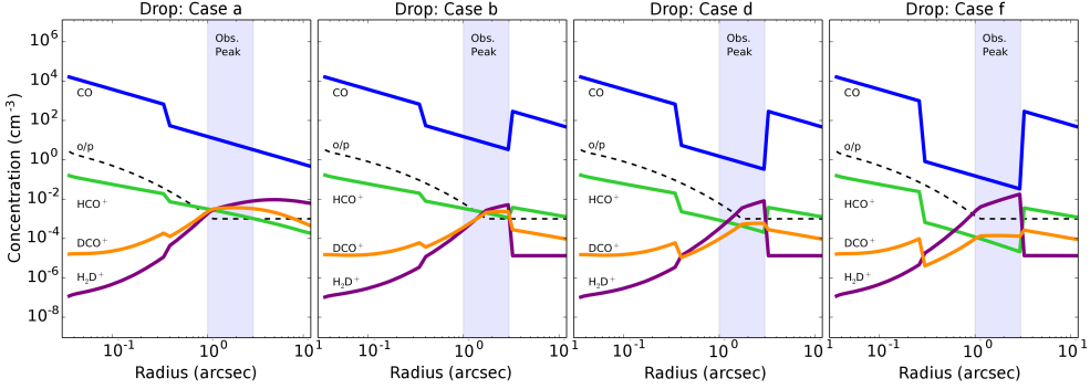
Figure 13: Chemical network results for Drop CO abundance with the decreased-temperature (Test 4) source profile for four cases (Table 2). Case d is the same as in the bottom row center panel of Fig. 6.
