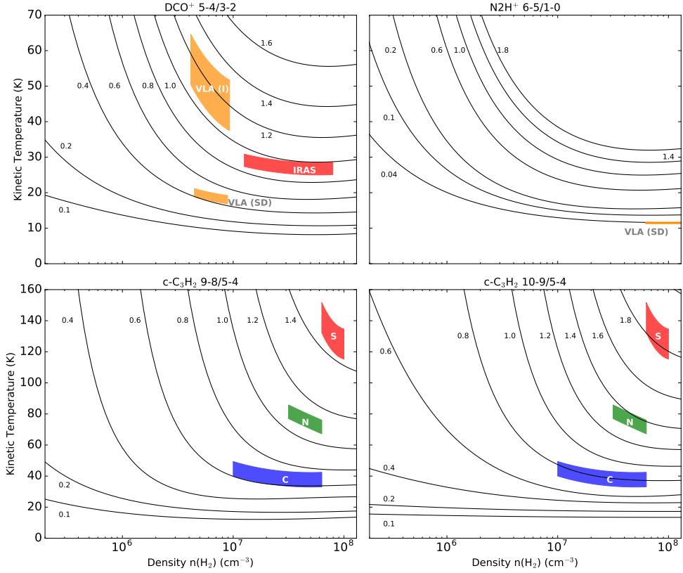
Figure 9: Calculated line ratios for \text{DCO}^+ 5-4/3-2, \text{N}_2\text{H}^+ 6-5/1-0 and \text{c-C}_3\text{H}_2 10-9/5-4 and 9-8/5-4. Black lines show the modelled ratios assuming column densities of 2.5 \times 10^{12} and 1.3 \times 10^{13} \text{cm}^{-2} for \text{DCO}^+ and \text{N}_2\text{H}^+ , respectively, and 2.5 \times 10^{13} for both \text{c-C}_3\text{H}_2 ratios. Color areas indicate the observed line ratios drawn over the range of densities and temperatures that characterize the observed emission, for IRAS 16293-2422 with ALMA (red, blue and green) and VLA 1623-2417 (orange) with single-dish (SD) and interferometric (I) observations.
