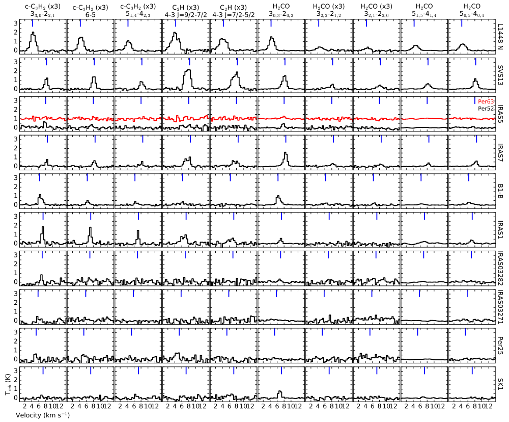
Figure 3: Same as Fig. 2 but for c-C 3 H 2 , C 2 H and H 2 CO.
