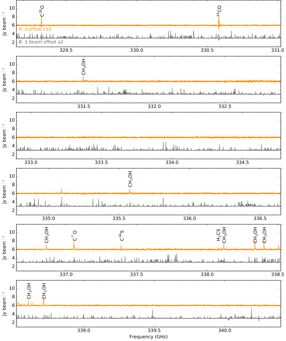
Figure 13: Full spectra obtained in the PILS survey for IRAS 16293-2422. Here the frequency range 329.15 to 340.4 GHz is shown. The rest of the spectra is shown in Fig. 14 and 15. The spectra for the IRAS 16293-2422 B is one beam away from the source position, note that it is multiplied by a factor of 2. The spectra for IRAS 16293-2422 A's outflow is centered at the observed peak of c\text{-C}_3\text{H}_2 , note that it is multiplied by a factor of 10 and shows very little emission other than c\text{-C}_3\text{H}_2 , \text{CH}_3\text{OH} , \text{H}_2\text{CS} , \text{H}_2\text{CO} and \text{HCO}^+ .
