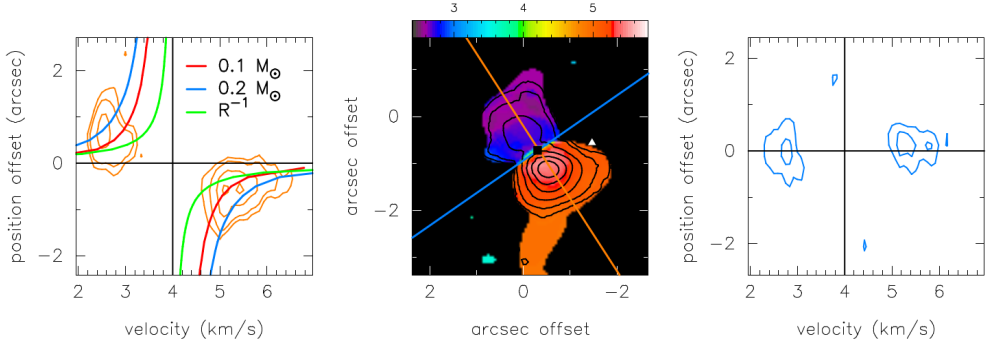
Figure 2: Observed C 18 O (2-1): Left: Pure Keplerian rotation curves ( v \propto R^{-0.5} , red and blue) and infall ( v \propto R^{-1} , green) are overlaid on the PV diagram. This suggests that the emission may be rotationally supported with M_* \sim 0.1\text{--}0.2 M_{\odot} . Center: C 18 O velocity map (Moment 1, half-tone) and intensity integrated (Moment 0, contours) maps. Contours are in steps of 3\sigma , 5\sigma , 10\sigma , 15\sigma , 20\sigma and 25\sigma with \sigma = 13 \text{ mJy beam}^{-1} . VLA1623A and B’s positions are marked with a square and triangle, respectively. Orange and blue lines indicate the image-space PV diagram cuts at PA = 35° (left) and 125° (right), respectively. Right: Lack of velocity gradient suggests no outflow contamination on the C 18 O emission. In both PV diagrams contours are in steps of 3\sigma , 5\sigma , 10\sigma and 15\sigma where \sigma = 19 \text{ mJy beam}^{-1} and the black lines indicate the systemic velocity and position of VLA1623A.
