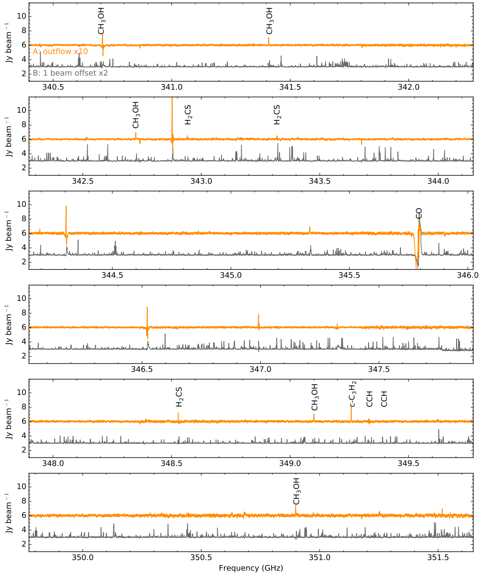
Figure 14: Same as in Fig. 13 but for the frequency range 340.4 to 351.65 GHz. \text{C}_2\text{H} is marked for reference.
