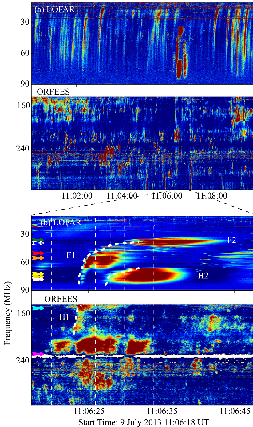
Fig. 1. Panel a: composite dynamic spectrum at frequencies of 10–240 MHz (top panel) showing multiple Type III radio bursts observed by LOFAR (top) and a Type I noise storm observed by ORFEES (bottom) on 9 July 2013 starting from 11:00 to 11:10 UT. Panel b: zoom in of the dynamic spectrum in (a) focussing on the bright J -burst observed by LOFAR (top) and ORFEES (bottom). The J -burst is denoted by white dashed lines and its components are labelled F1, F2, H1, and, H2. The vertical lines and colour-coded arrows denote the time and frequency, respectively, of the bursts shown in Fig. 2.
