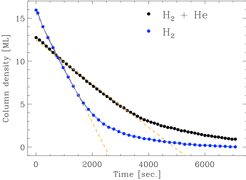
Figure 3.11: CO photodesorption of ices irradiated with either Pure \text{H}_2 at 0.41 mbar (blue) or \text{H}_2\text{:He} 1:3 (black) at 2.13 mbar.
