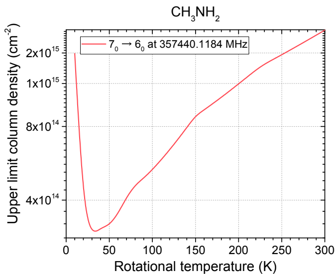
Figure 9.7: Upper limit column density for the strongest CH 3 NH 2 transition. A 3\sigma value of 23 mJy km s -1 is used.
