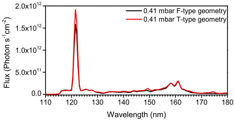
Figure 3.7: VUV spectra in the 110 – 180 nm range of different geometry MDHLs (F- and T-types) at a molecular hydrogen pressure of 0.41 mbar.
