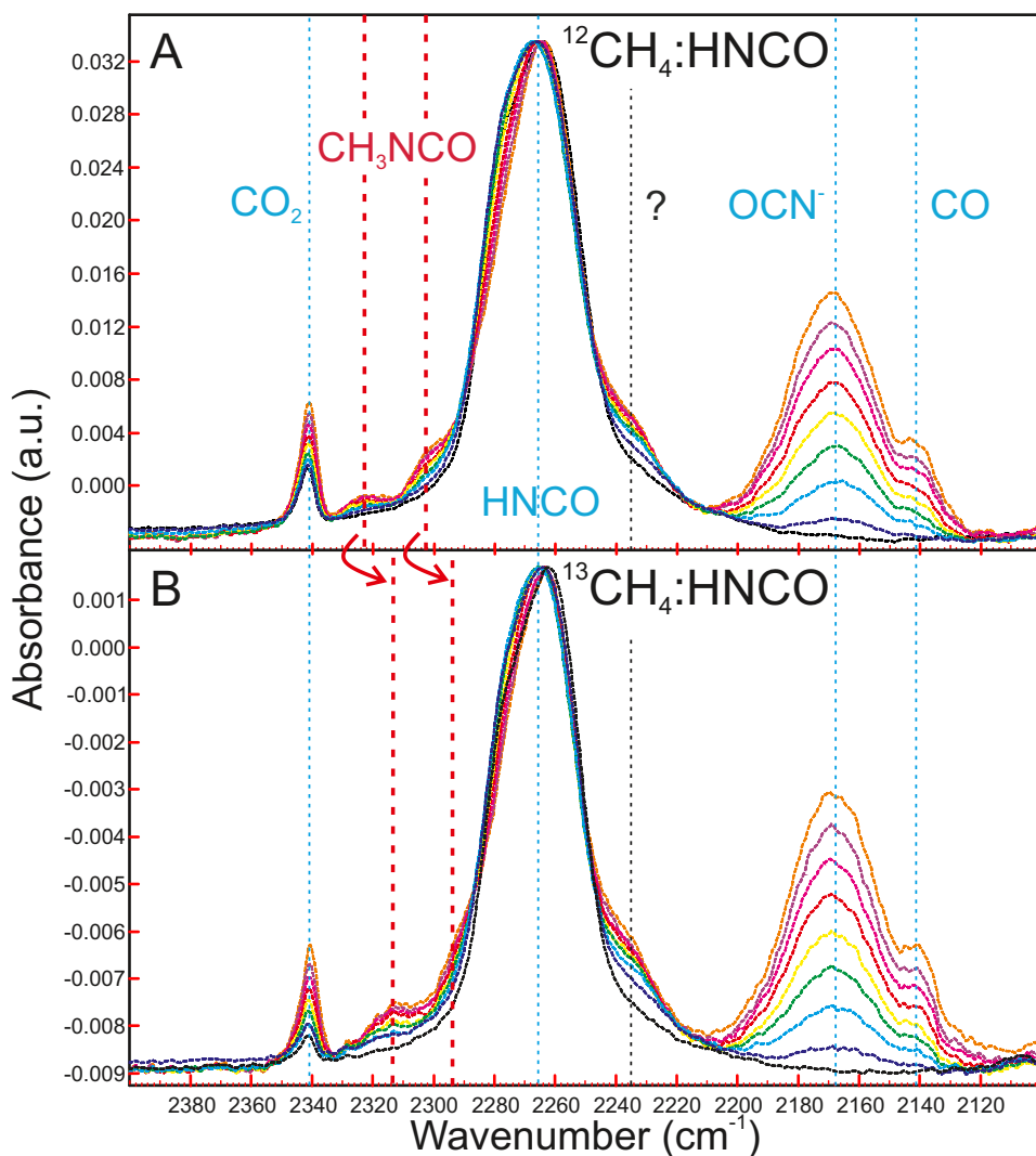
Figure 6.5: IR spectra taken over time for the ^{12}\text{CH}_4:\text{HNCO} (A) and ^{13}\text{CH}_4:\text{HNCO} (B) mixture. \text{HNCO} and the products \text{CO}_2 , \text{OCN}^- and \text{CO} are listed (blue). Spectroscopic features that coincide with \text{CH}_3\text{NCO} are found at the red lines and show a clear shift with the ^{13}\text{CH}_4 isotopologue. One unidentified peak is found in the right wing of the \text{HNCO} peak, indicated by a question mark.
