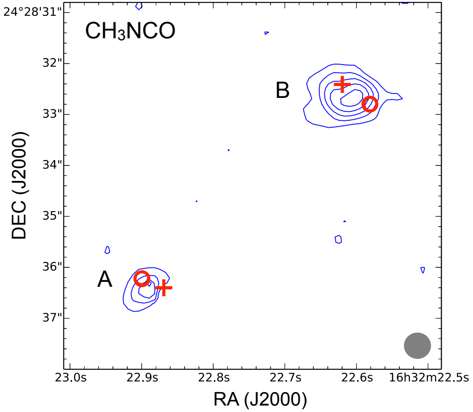
Figure 6.2: Integrated intensity map of the \text{CH}_3\text{NCO} 39_{0,39,0} – 38_{0,38,0} transition at 336339.9 MHz and E_{\text{up}} = 323.7 K between 1.7 and 3.7 \text{km s}^{-1} . The positions of the continuum of source A (South East source) and source B (North West source) are indicated with red crosses, while the positions studied in this chapter are indicated with red circles. The contour levels start at 5\sigma with additional steps of 5\sigma . The circular restoring beam of 0.5 arcsec size is indicated in grey in the right hand lower corner.
