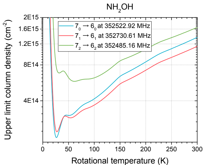
Figure 9.8: Upper limit column densities for the three strongest NH 2 OH transitions. 3\sigma values of 27, 21 and 27 mJy km s -1 are used for the respective lines.
