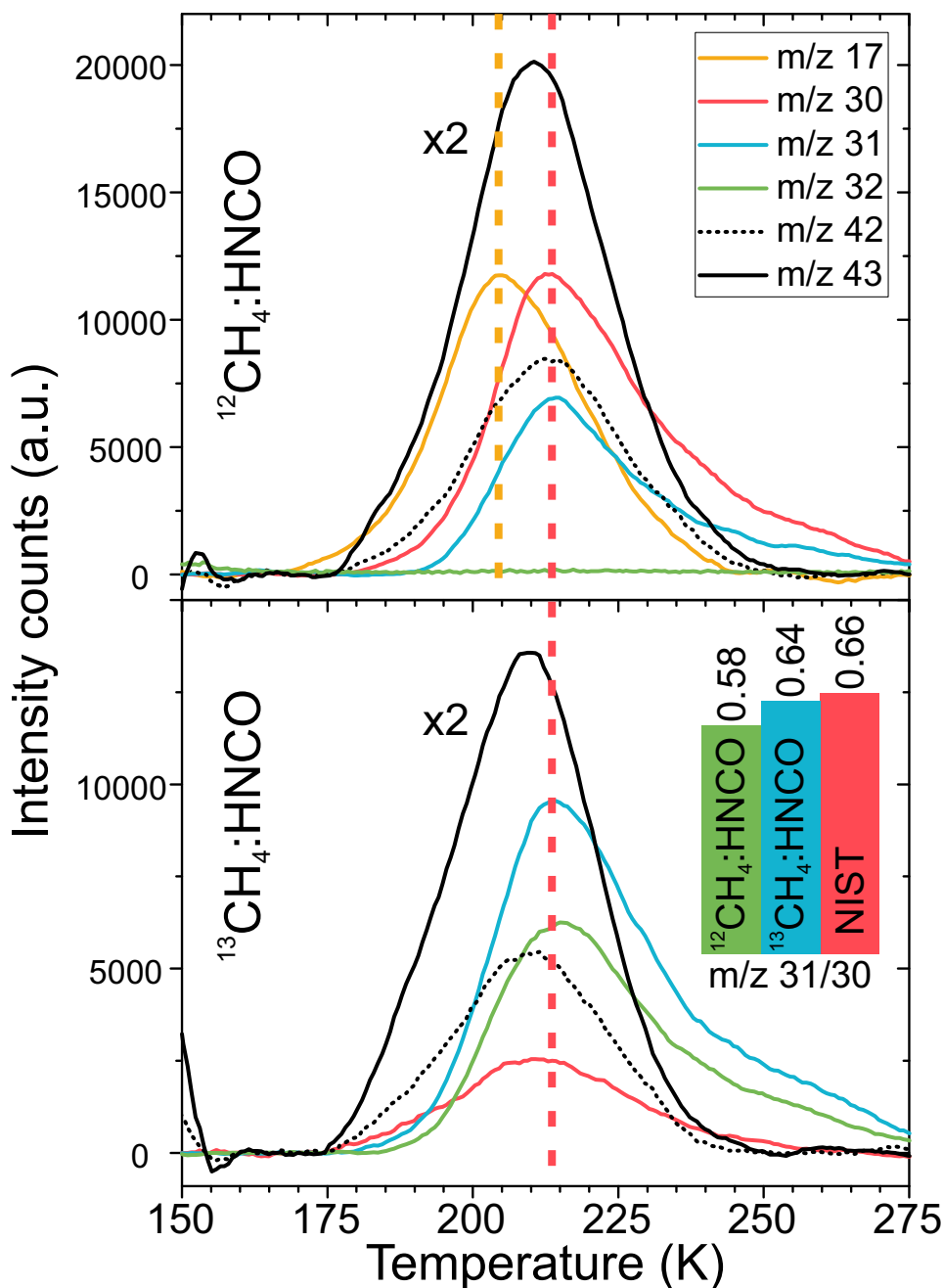
Figure 7.7: TPD trace of m/z 17 (yellow), 30 (red), 31 (blue), 32 (green), 42 (black dashed) and 43 (black, scaled by factor 1/2) of HNC0: 12 CH 4 (experiment 1, top) and HNC0: 13 CH 4 (experiment 3, bottom) ice. The dashed yellow line indicates the peak desorption temperature of m/z 17 and the red dashed line indicates the peak desorption temperature of m/z 30, 31 and 32. The inset gives the m/z 31/30 ratio for the two experiments and as given in the NIST database.
