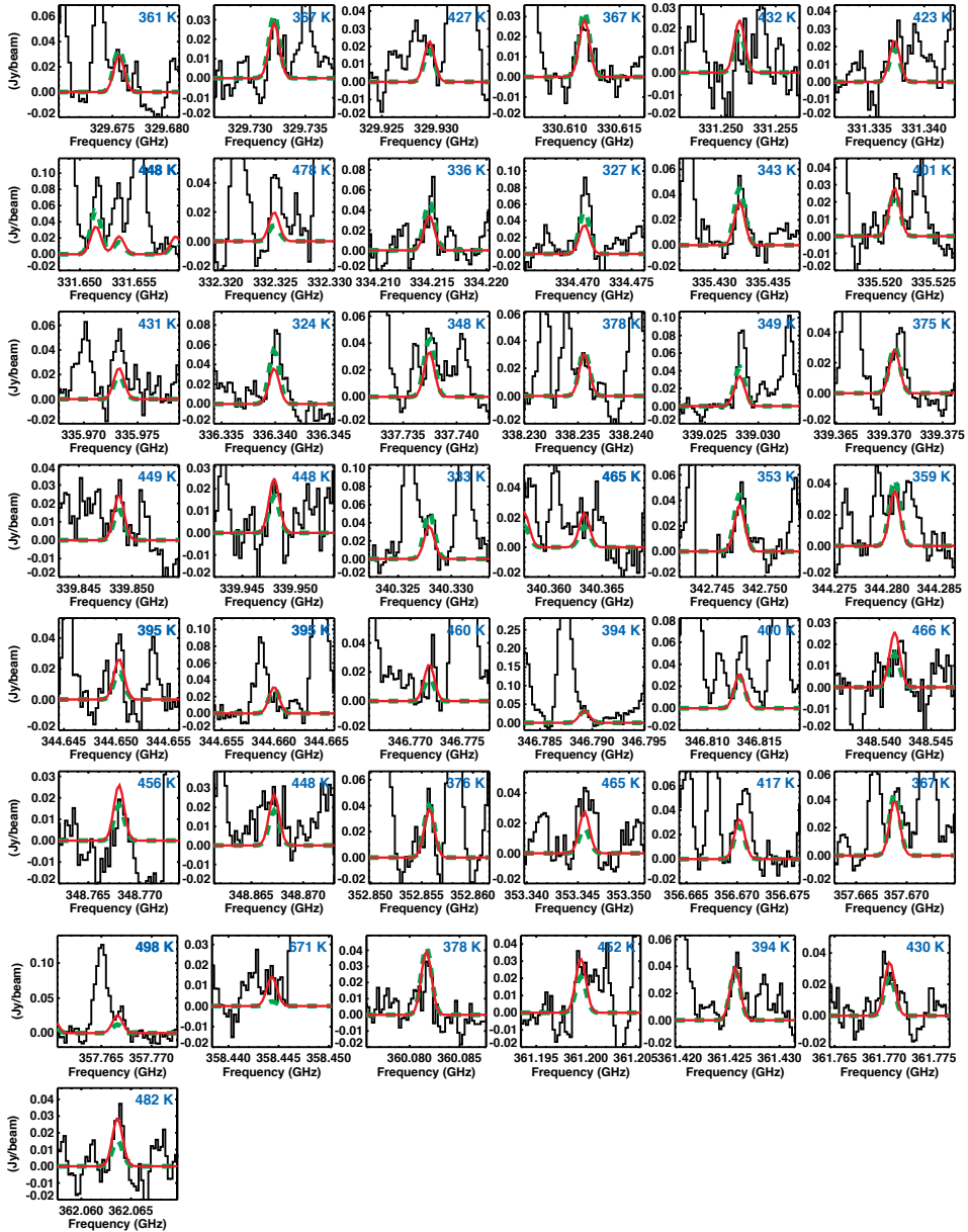
Figure 6.3: Black: detected unblended lines of \text{CH}_3\text{NCO} toward source B. Red solid: best-fit model for T_{\text{ex}} = 300 K. Green dashed: best-fit model for T_{\text{ex}} = 100 K. The E_{\text{up}} values of the lines are indicated in blue in the right upper part of each panel.
