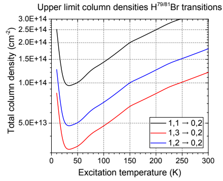
Figure 10.6: Upper limit column densities for the \text{H}^{79/81}\text{Br} (e.g. ^{79}\text{Br} and ^{81}\text{Br} are used interchangeably here) J = 1_x \rightarrow 0_2 transitions plotted versus rotational temperature based on the 3\sigma values ( 216 \text{ mK km s}^{-1} ) found for the Orion KL Hot Core and beam-dilution corrected ( \eta = 0.049 )
