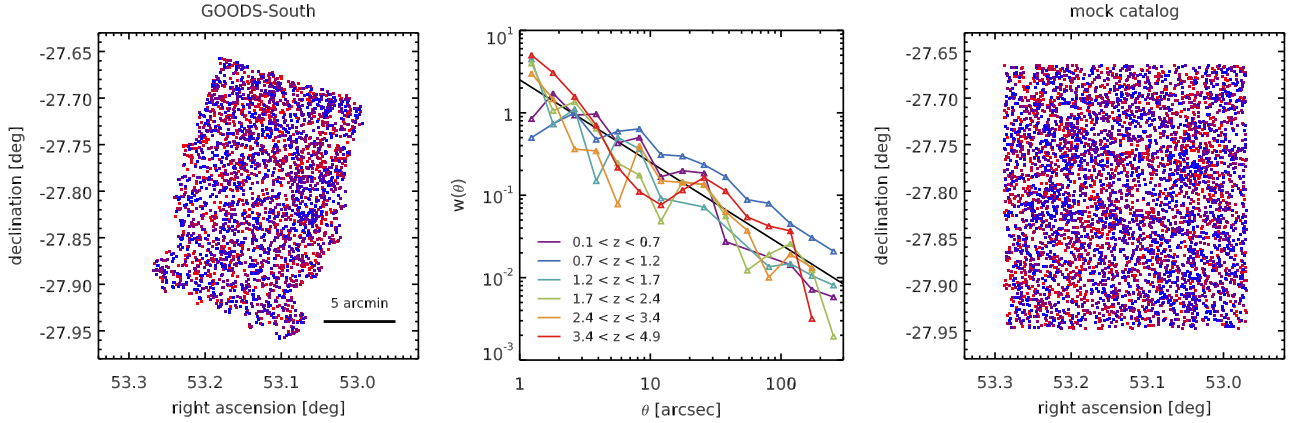
Fig. 5. Left: sky positions of the galaxies in the GOODS-South field with H < 23 . The colors indicate the redshift: blue points are z < 0.3 , red points are z > 1.5 , and galaxies in between are shown in shades of purple. Middle: angular two-point correlation function for GOODS-South galaxies with 9 < \log_{10}(M_*/M_\odot) < 10.3 , in various redshift slices as indicated in the legend. The straight black line is a power law of index -1 . Error bars are not shown for clarity. Right: same as left, but for the mock catalog produced by EGG.
