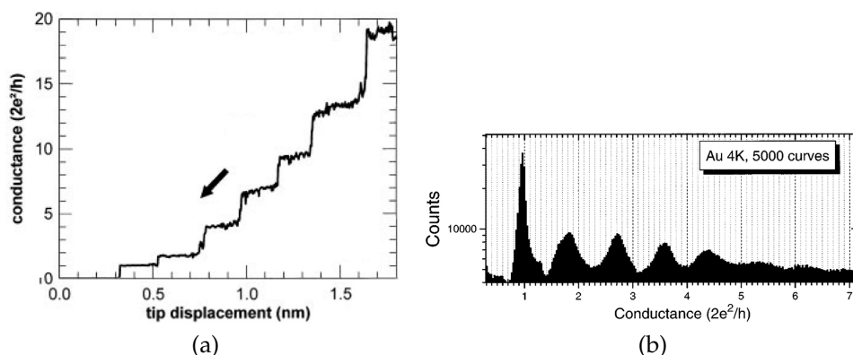
Figure 1.2: (a) Conductance steps associated quantization measured in a gold (Au) point contact (b) A typical conductance histogram of Au atomic point contacts. Above Figures are taken from Rubio et al. [24] and Costa-Krämer et al. [25]
