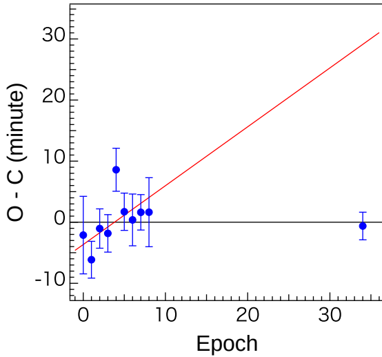
Fig. 7. Residuals of the observed mid-transit times from the current best-fit transit ephemeris. The red line represents the best-fit transit ephemeris for the transits from K2 only. We note that the transit ephemeris from K2 has an uncertainty of \sim 17 minutes at the epoch of 34. Thus the discrepancy is still within the 2\sigma level.
