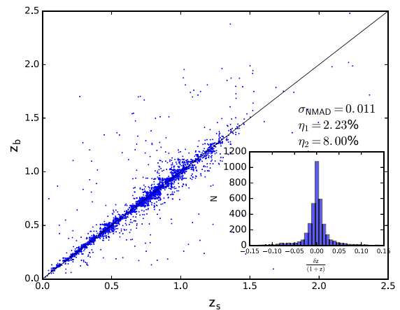
Figure 10. ALHAMBRA K_s photometric redshift z_b versus spectroscopic redshift z_s for 3736 sources. The inset shows the distribution of the deviations \delta z / (1 + z) . The measured scatter is \sigma_{\text{NMAD}} = 0.011 , with catastrophic error rates \eta_1 \sim 2.3 per cent, \eta_2 \sim 8.0 per cent.
