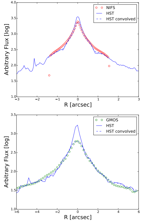
Fig. B.1. Determination of the NIFS ( top ) and GMOS ( bottom ) PSF by comparing the light profiles of the NIFS/GMOS and HST images along the major axis. In both panels the open circles denote the IFU profiles and blue solid lines the HST profiles. The HST profiles were convolved with the PSFs of Table 2 to fit the IFU data and are shown as dashed blue lines.
