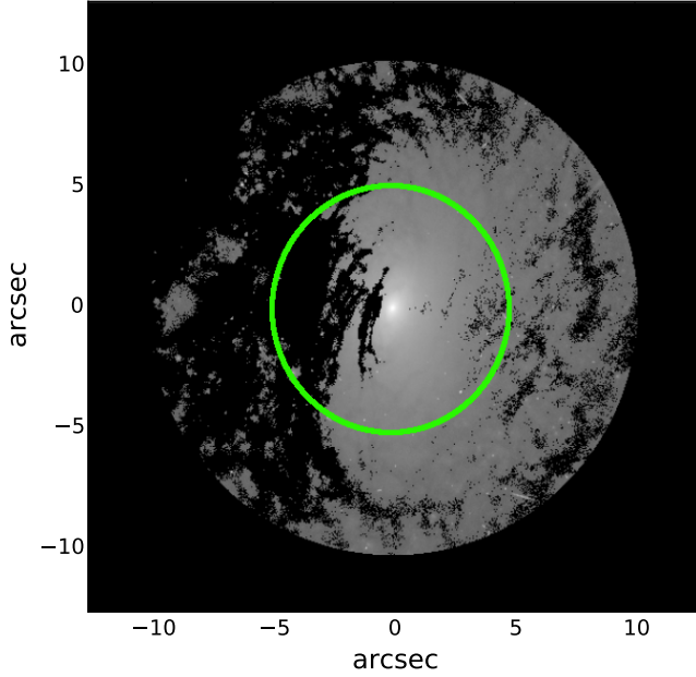
Fig. A.4. Dust masked region of the HST/ F606W image. The black parts of the image are the regions which were masked to account for dust attenuation. The green circle marks the region which was used in the MGE modeling ( r < 5'' ).
