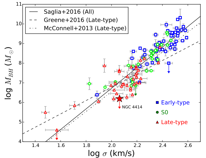
Fig. 12. Location of the upper limit mass measurement of NGC 4414 in the M_{\text{BH}} - \sigma_e relation. The data points were taken from the BH compilation of Saglia et al. (2016) in addition to measurements by Verdoes Kleijn et al. (2002), Greene et al. (2010), Coccato et al. (2006), De Lorenzi et al. (2013), den Brok et al. (2015), Walsh et al. (2015, 2016), Greene et al. (2016), Thomas et al. (2016), Bentz et al. (2016) and divided into early-type galaxies (blue), S0 type (green) and late-type galaxies (red). Our upper-limit measurement is indicated by a red star. We have also added the scaling relations by Saglia et al. (2016) for all types of galaxies (solid) and Greene et al. (2016), McConnell & Ma (2013) for late-type galaxies (dashed, dashed-dotted).
