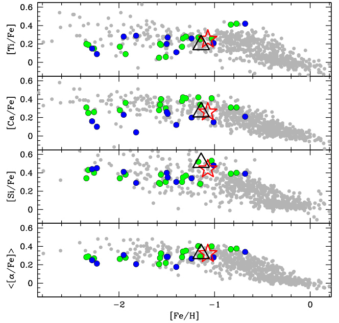
Figure 4. Upper three panels: [Si/Fe], [Ca/Fe], [Ti/Fe] versus [Fe/H] trends for NGC 6362, field stars (same symbols of Fig. 3) and Galactic GCs (green circles are taken from Carretta et al. 2009, blue circles are taken from Mészáros et al. 2015). Lower panel: same comparison on the \langle[\alpha/\text{Fe}]\rangle versus [Fe/H] trend. NGC 6362 is in very good agreement with what observed for the other GCs.
