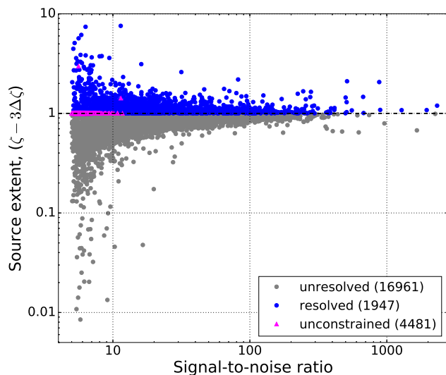
Figure 3. S-PASS source extents ( \zeta - 3\Delta\zeta ) as a function of signal-to-noise ratio. Magenta triangles represent sources with unconstrained source size errors (i.e. \Delta a = -1 \text{ arcsec} or \Delta b = -1 \text{ arcsec} in Table 3). Resolved sources are depicted as blue circles and unresolved sources are shown as grey circles. The catalogue consists of 8% resolved sources and 73% unresolved sources, with the remaining 19% having unconstrained source size errors.
