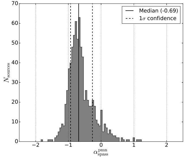
Figure 5. Spectral index distribution between 2.3 GHz and 4.8 GHz for all S-PASS sources with S_{\text{peak}} > 500 \text{ mJy beam}^{-1} and a counterpart in PMN. The solid black line identifies the median spectral index ( \alpha_{\text{spass}}^{\text{pmn}} = -0.69 \pm 0.02 ) and the black dashed lines represent the 1\sigma confidence interval ( -0.93 to -0.26 ). Note the extended tail of flat and inverted spectral indices.
