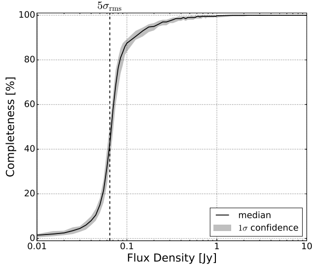
Figure 8. The S-PASS catalogue median completeness (solid black line) and the 67% confidence interval (shaded grey). The 5\sigma_{\text{rms}} cut-off is indicated by the vertical dashed line.
