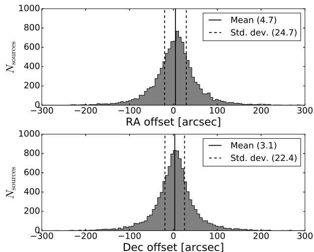
Figure 6. Astrometric offset distributions from cross-matching S-PASS with SUMSS. The mean offset in RA is 4.7 arcsec and 3.1 arcsec in Dec. The solid black line represents the distribution mean and the dashed lines identify the standard deviation.
