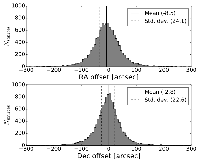
Figure 7. Astrometric offset distributions from cross-matching S-PASS with NVSS. The mean offset in RA is -8.5 arcsec and -2.8 arcsec in Dec. The solid black line represents the distribution mean and the dashed lines identify the standard deviation.
