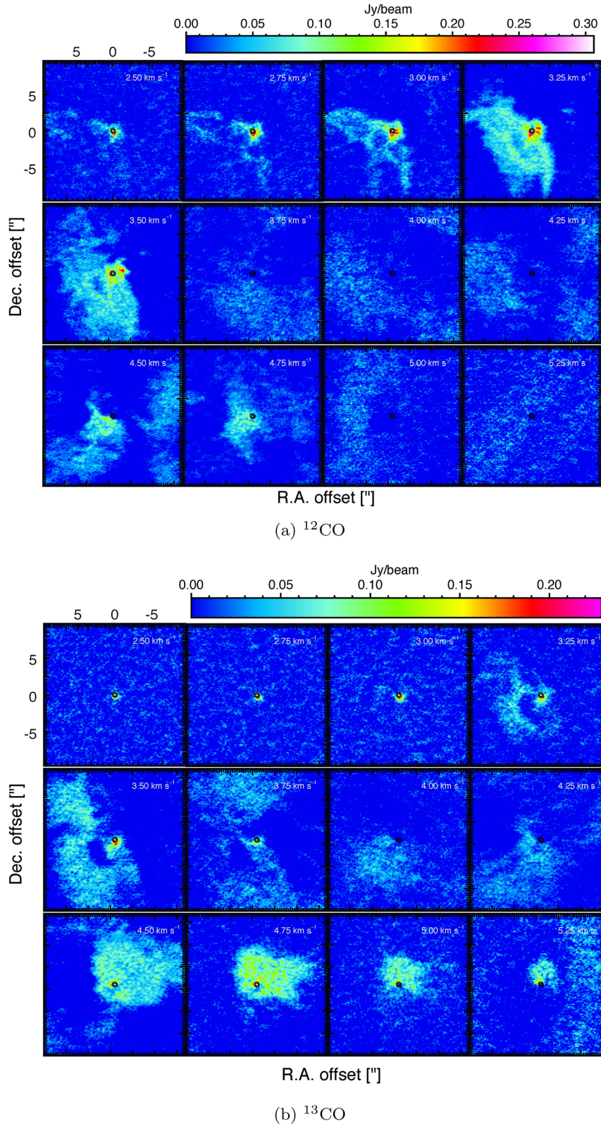
Figure 4. Channel maps of the ^{12}\text{CO} and ^{13}\text{CO} . LSR velocities are shown at the top-right corner of each panel with a systemic velocity of \sim 4.3 \text{ km s}^{-1} . Black contours represent the continuum emission around V883 Ori as shown in Fig. 2(a).
