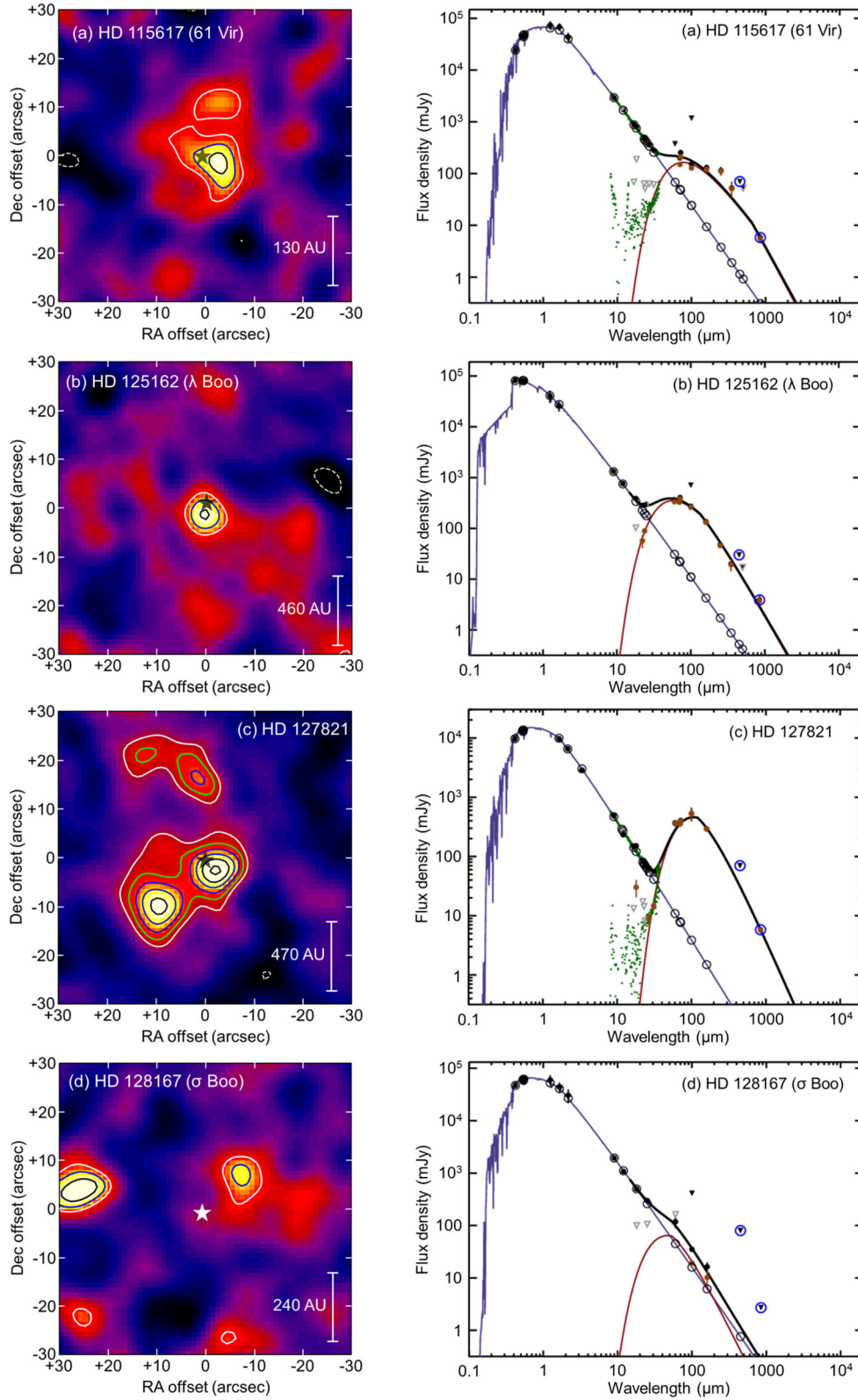
Figure A9. As for Fig. A1 for the targets (a) HD 115617 (61 Vir), (b) HD 125162 (λ Boo), (c) HD 127821 and (d) HD 128167 (σ Boo).
