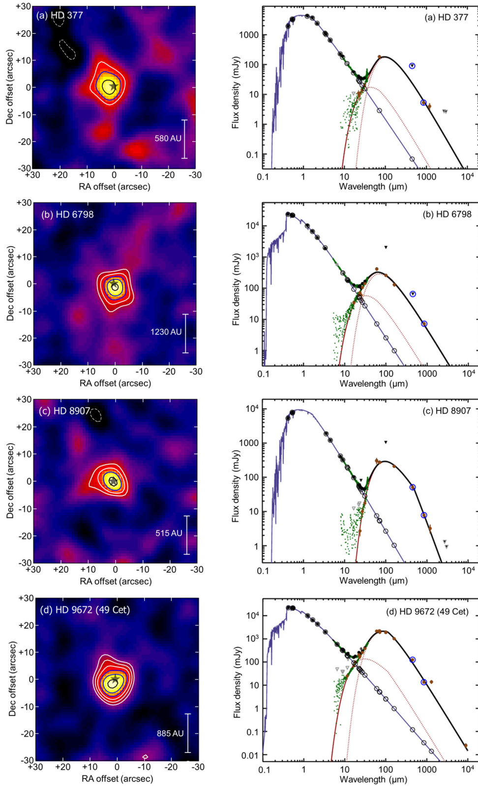
Figure A1. 850 μm S/N images and SEDs for the targets (a) HD 377, (b) HD 6798, (c) HD 8907 and (d) HD 9672 (49 Cet).
