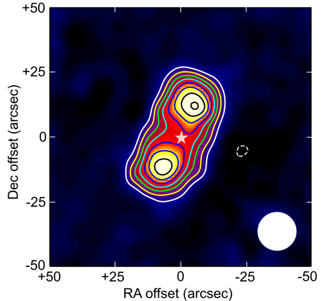
Figure 4. The Fomalhaut debris disc imaged by SCUBA-2 at 850\ \mu\text{m} . This S/N image is colour scaled from -5\sigma (black) to the maximum S/N in the image at 26\sigma (white). The dashed contour is at -5\sigma and the solid contours start at 5\sigma and increase in 3\sigma steps. The star symbol shows the position of Fomalhaut with respect to the disc (after proper motion corrections). The white circle represents the approximate FWHM beam size at 850\ \mu\text{m} after smoothing.
