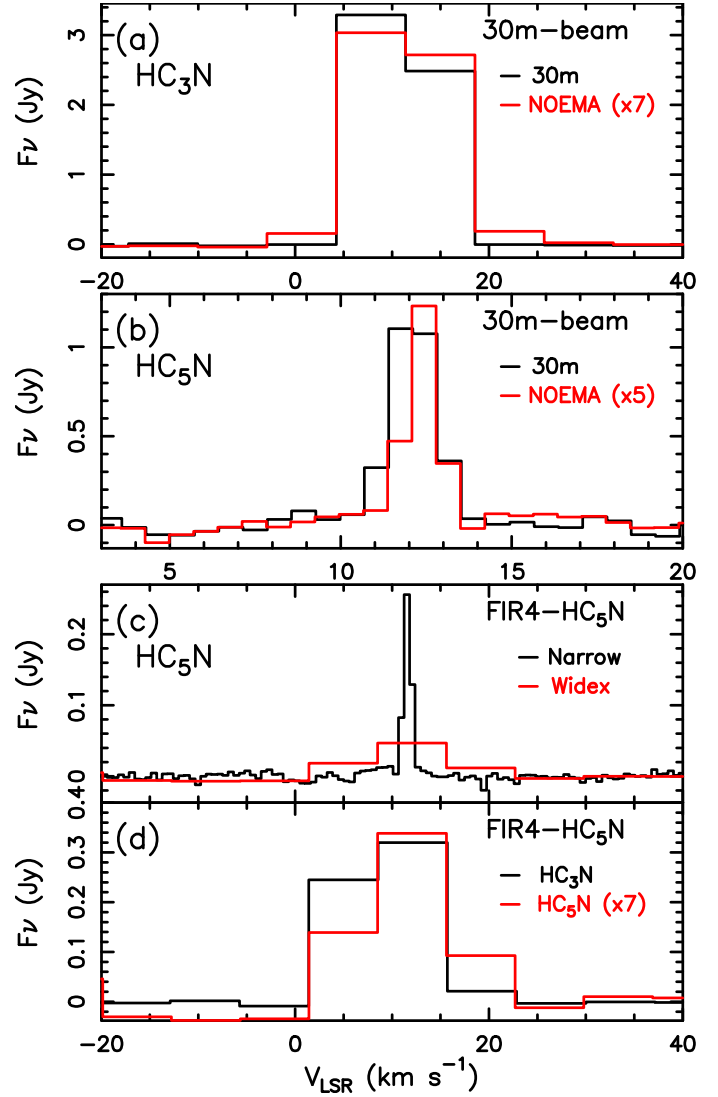
Fig. A.1. a ) Spectrum of \text{HC}_3\text{N} (9–8) obtained with the IRAM-30 m Telescope (black histogram) in the framework of the ASAI large program, and SOLIS-NOEMA spectrum (red histogram) extracted from a circular region equal to the IRAM-30 m HPBW ( \sim 30'' ). We note that the flux resulting from the convolved NOEMA observations have been multiplied by a factor 7 to match those of the 30 m Telescope: we thus recover about the 15% of the total flux. b ) Same as panel a for \text{HC}_5\text{N} (31–30). In this case, the NOEMA spectrum has been multiplied by a factor 5. From the plot, it is apparent that we recover slightly less than the 20% of the total flux. c ) Comparison between the Narrow (black) and Widex (red) spectrum of \text{HC}_5\text{N} (31–30), both integrated on the region FIR4- \text{HC}_5\text{N} (red contour in Fig. 1). The integral under the channel with signal is different by \sim 7\% (see Sect. 2). d ) Widex spectra of \text{HC}_3\text{N} (black) and \text{HC}_5\text{N} (red) integrated over the same region as in panel c . The \text{HC}_5\text{N} spectrum has been multiplied by 7 for clarity of the figure.
