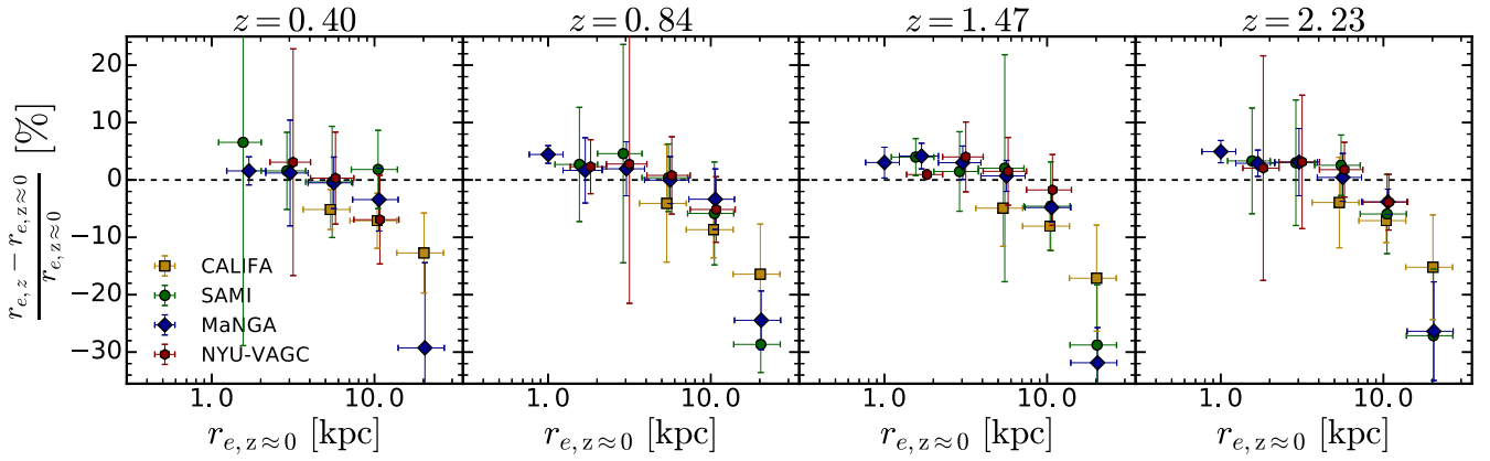
Figure 4. The fraction difference between the recovered and input effective radius ( r_{e,z} - r_{e,z \approx 0} )/ r_{e,z \approx 0} , for each of the local subsamples and each redshift (one per column). Each symbol represents the median values in bins (with a minimum of 10 galaxies) of width of the horizontal error bar. The vertical error bar shows the error on the median value. The black dashed line pinpoints a fractional difference of 0, i.e. when the recovered effective radius is the same as input. We find the difference to be very small (<10 per cent) up to 10 kpc. Above that value, the size of galaxies is more severely underestimated ( \sim 10 –30 per cent). Small horizontal offsets were applied to improve the readability of the plot.
