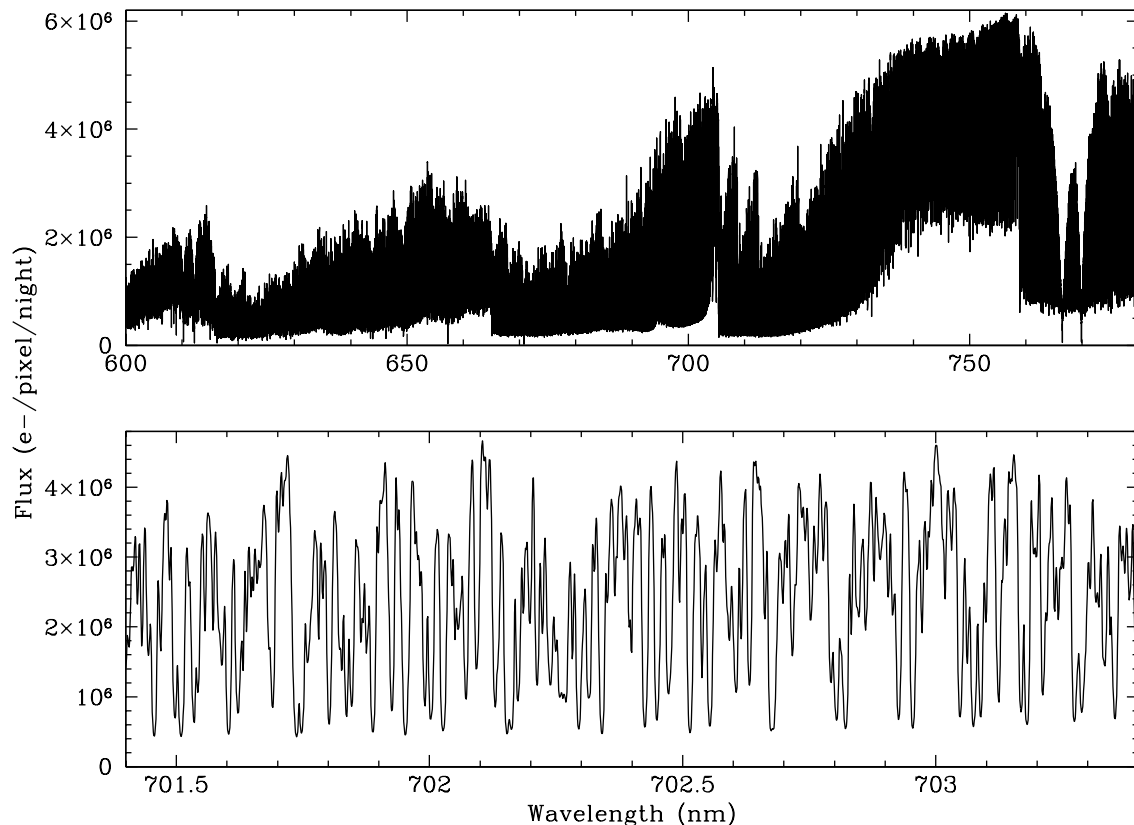
Fig. 4. PHOENIX high-resolution spectrum simulating an observation of Proxima with SPHERE+ESPRESSO. The total integration time is eight hours. Top: the 600–780 nm region, which would be used for SPHERE+ESPRESSO observations. Bottom: close-up view showing the very high density of spectral lines in this star.
