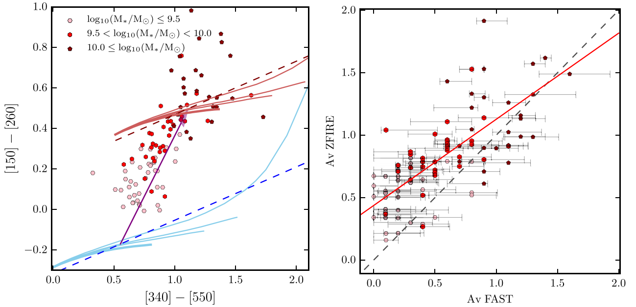
Figure 10. Dust parametrizations to investigate IMF dependences of dust extinction values. Galaxies are divided into three mass bins. Left: the dust content of the galaxies are parametrized using UV/optical colours. The cyan solid lines are PEGASE models for \Gamma = -1.35 IMF with varying SFHs. The dashed blue line is the best-fitting line for these models. The pink lines are similar to the cyan lines, but with an extinction of 1 mag. The magenta dashed line is the best-fitting line for these models with A_V = 1 . The purple arrow denotes the direction of the dust vector and connects the two best-fitting lines at time t . Right: comparison between the extinction derived by equation (6) with the extinction values derived by FAST. The error bars are the upper and lower 68th percentile of the A_V values compiled by FAST and the diagonal red line is the error-weighted least-squares fit to the data. The diagonal dashed line is the A_V(\text{SED}) = A_V(\text{ZF}) line.
