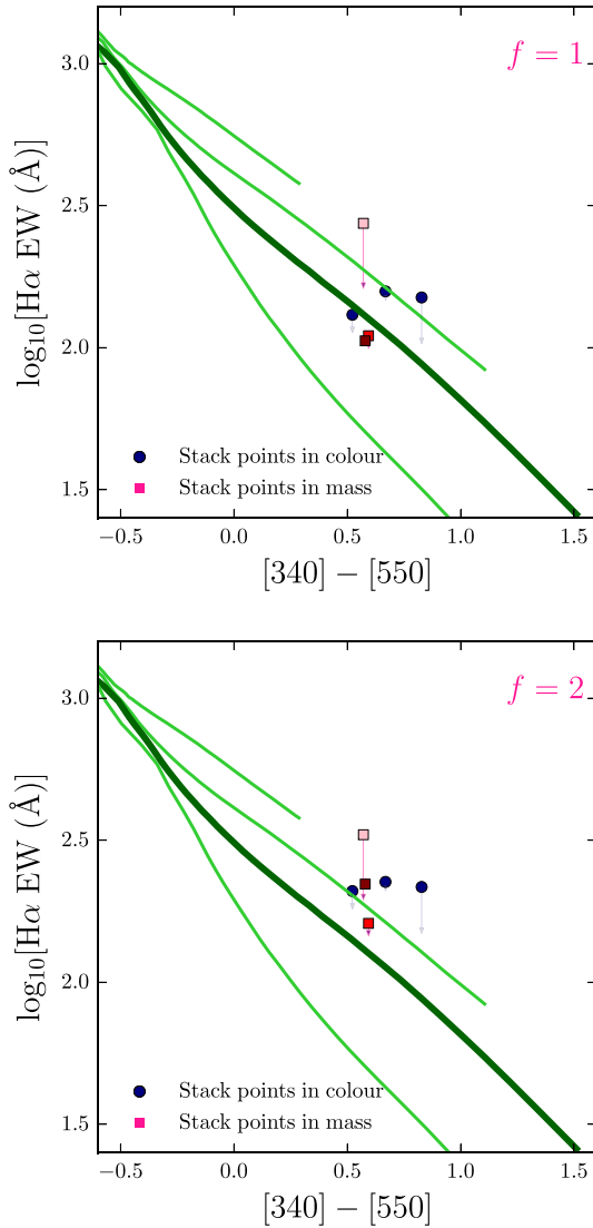
Figure 16. Here, we show the effect of adding the continuum contribution (c2) of galaxies with no H\alpha detections to the ZFIRE-SP sample stacks. Galaxies are stacked in mass and colour bins and the arrows show the change in EW when the contribution from c2 is added to the data. All tracks shown are similar to Fig. 15. Top : dust corrections applied with f = 1 . The errors for the data points are similar to Fig. 15 (centre panel). Bottom : dust corrections applied with f = 2 . The errors for the data points are similar to Fig. 15 (right-hand panel).
