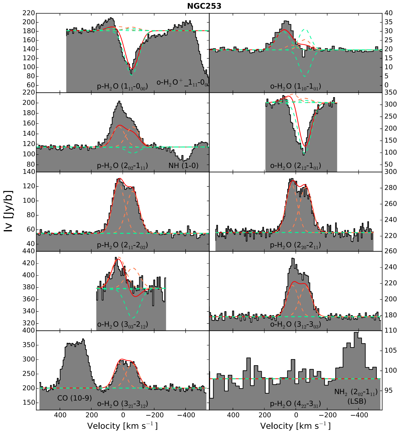
Figure 12. Observed H 2 O spectra (gray histograms) and the modeling results (red solid curve) of NGC 253. For explanation of the symbols used in the plots, see Figure 11.
