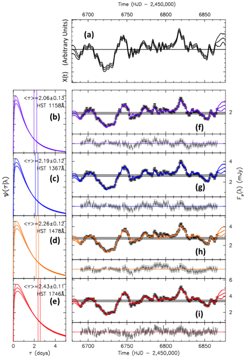
Figure 2. Model 2 fits to the HST light curves. Panels (b)–(e) show the mean response functions and 1\sigma error envelopes from the MCMC samples. Vertical lines in these panels indicate the mean and standard deviation in \langle\tau\rangle . Panels (f)–(h) show the inferred echo light curves with residuals included beneath each light curve. Panel (a) shows the inferred driving light curve.
