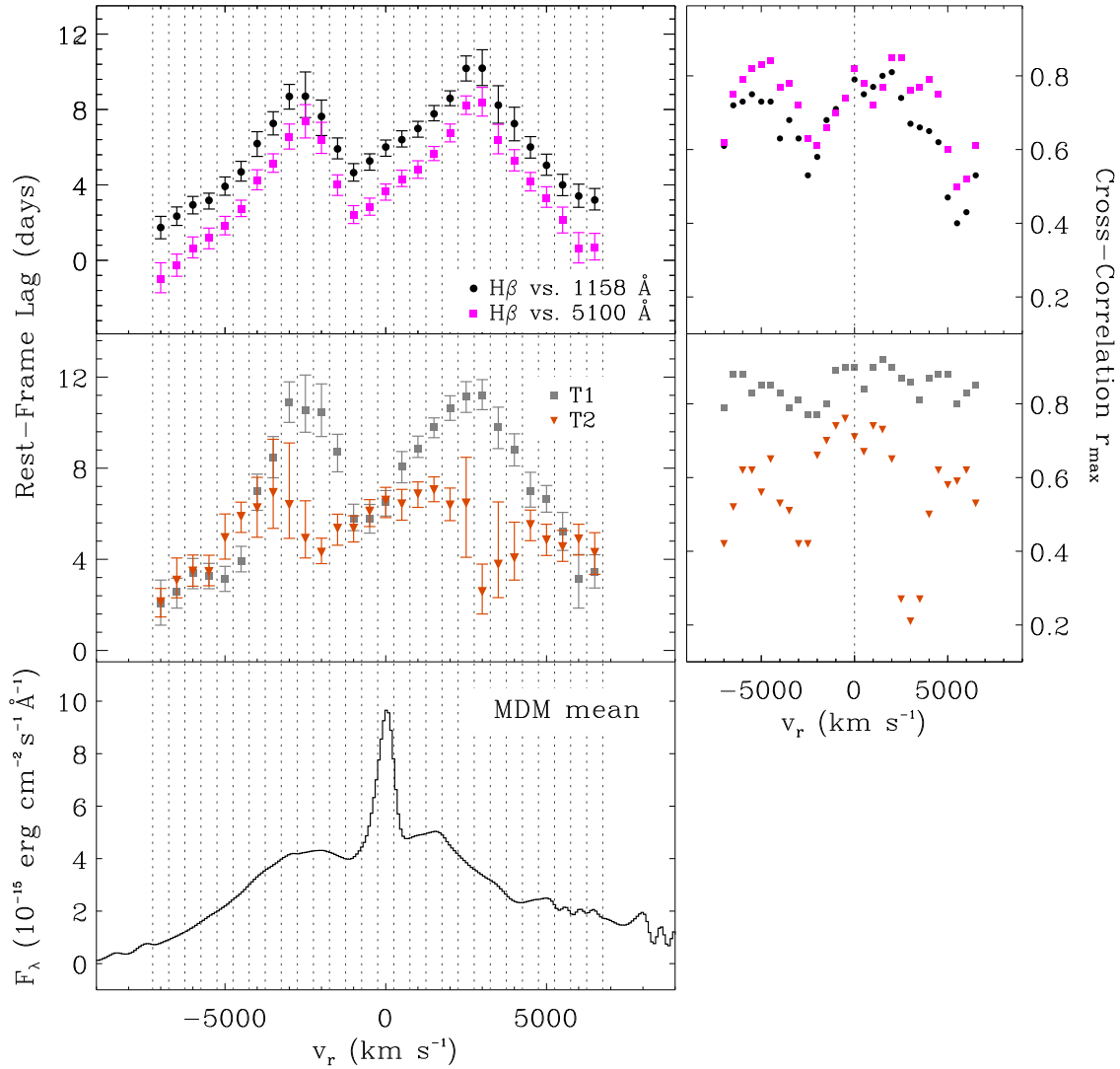
Figure 11. Top left: ICCF H \beta lags ( \tau_{\text{cen}} ) for 500 \text{km s}^{-1} bins measured against the 1158 Å and 5100 Å continua. Middle left: lags for T1 and T2 measured against the 1158 Å continuum. Bottom left: MDM mean spectrum for the full campaign. Right: maximum cross-correlation coefficients ( r_{\text{max}} ) for individual velocity bins.
