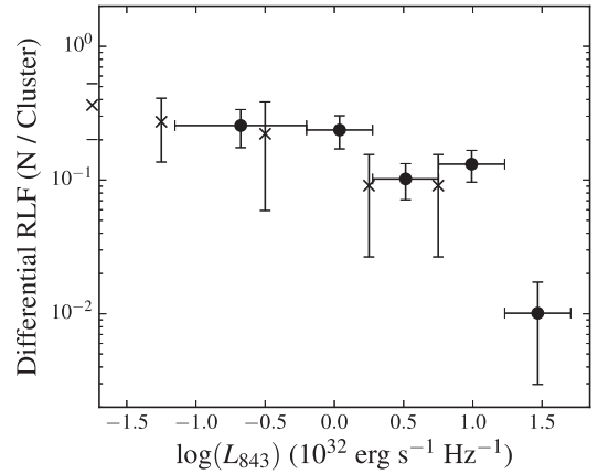
Figure 5. The differential RLF at 843 MHz for our SPT sample (filled circles) and the sample of Branchesi et al. (2006) of 0.3 < z < 0.8 X-ray-selected NEP clusters (crosses), adjusted for our method of calculating the RLF.
