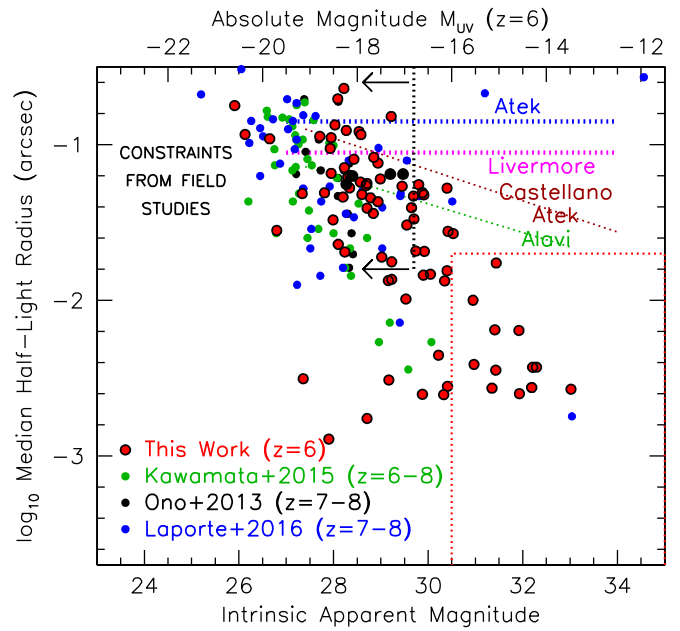
Figure 12. Comparison of various observational constraints on the measured sizes of faint z = 6-8 galaxies from the HUDF (Ono et al. 2013; black circles), the Abell 2744 HFF cluster + parallel field (Kawamata et al. 2015; green circles), the MACS0416 + MACS0717 HFF cluster + parallel field (Laporte et al. 2016; blue circles), as well as the measured and magnification-corrected sizes of sources behind Abell 2744 and MACS0416 (red circles) using GALFIT. The dotted red box shows the constraints we obtain via our indirect arguments. These constraints are shown in relation to the assumptions that have been made in a number of recent studies looking at the z = 2-8 UV LFs (indicated with solid + dotted lines). In particular, Alavi et al. (2016) and Castellano et al. (2016b) had assumed that the faint galaxies had sizes governed by an extrapolation of the Shibuya et al. (2015) and Huang et al. (2013) size-luminosity relation to >29 mag, and Livermore et al. (2017) assumed median sizes of 0.5 kpc (equivalent to an intrinsic half-light radius of \sim 90 mas). Atek et al. (2014, 2015a) assumed an intrinsic half-light radius of \sim 150 mas and that galaxies follow the Huang et al. (2013) size-luminosity scalings. Each of these assumptions was plausible, as each reproduced the sizes of galaxies toward the faint end of the HUDF observations. However, the present observations suggest that faint galaxies have even smaller sizes than what had been assumed in most previous work. Even if the smaller sizes that we find here are a significant fraction of the sample at >29 mag, the corrections rapidly diverge for larger sizes and so any sample at such magnitudes is going to rapidly become uncorrectable for all practical purposes, leading to quite inaccurate volume densities and LFs.
