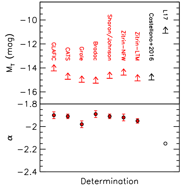
Figure 9. (Upper panel) Brightest luminosity allowed for a potential turn-over in the z \sim 6 UV LF (within our 68% confidence intervals), using faint z \sim 6 galaxies identified behind the first four HFF clusters and assuming different magnification models represent reality. The reported constraints from Castellano et al. (2016b) and L17 are also presented, with the L17 constraints plotted at a \Delta(\text{BIC}) value of two. The substantially fainter allowed turn-over luminosity reported by L17 (significantly discrepant with the other estimates) is likely an artifact of the very large sizes that L17 assume (see Figure 11, Sections 6.1.2, 6.2, and also Bouwens et al. 2017) and a large number of sources close to the detection limit of their selection (Figure 12). (Lower panel) Faint-end slope \alpha determinations using only the HFF cluster search results. See Table 2 for a tabulation of these results.
