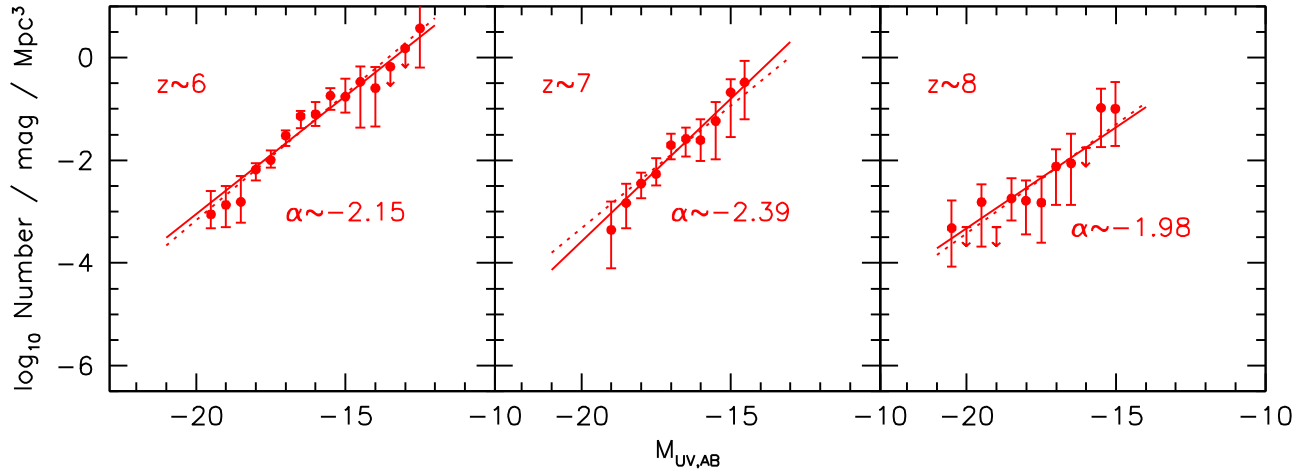
Figure 18. Power-law fits (solid lines) to the binned z \sim 6, 7 , and 8 LF results from L17 in an effort to estimate the faint-end slope estimates from the HFF results alone. Also presented (dotted lines) are fits done to the L17 HFF LF results anchored to the field LF results from the same group (Finkelstein et al. 2015) at M_{UV,AB} = -20 . The motivation for deriving the faint-end slopes \alpha from the HFF results alone is to keep the derived results independent of those derived for the field. This makes it possible to compare the lensed LF results and field LF results in a fair way, as we do in Figure 1.
