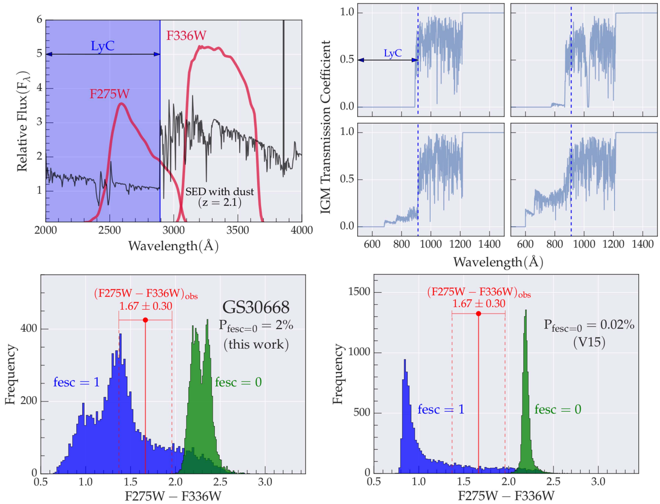
Figure 1. Summary of the selection technique adopted in this paper illustrated with the first LyC candidate GS 30668 ( z = 2.172 ). Top left: at GS 30668’s redshift, >50\% of the F275W band is covered by the LyC (shown as the shaded blue region), and hence LyC leakage may be inferred from the flux observed in that band. The SED shown is a BPASSv2 model SED with \beta_{\text{UV}} and age consistent with GS 30668, and E(B - V) = 0.03 (using the dust extinction curve from Reddy et al. 2016a). Top right: four realizations of the IGM transmission curves toward a z = 2 galaxy from the Inoue et al. (2014) Monte Carlo sampling, with \lambda = 912 \text{ \AA} indicated by blue dotted lines. A total of 10,000 such curves are convolved with a Gaussian distribution of SEDs ( \mu = \beta_{\text{Obs}} , \sigma = \sigma_{\beta_{\text{Obs}}} ) in our method to compute the expected color distribution generated in the bottom left panel. Bottom left: the observed F275W–F336W color (red dot with error bars) lies almost entirely blueward of the color distribution generated under the assumption that f_{\text{esc}} = 0 (shown in green). The probability for f_{\text{esc}} = 0 for GS 30668 is P(f_{\text{esc}} = 0) = 2\% , which makes it an LyC candidate. Further, the actually measured color perfectly lines up with the distribution generated under the assumption that f_{\text{esc}} = 1 (shown in blue), strongly suggesting a high value of f_{\text{esc}} for this galaxy. Bottom right: same color distributions as on the left, but following the original V15 method, in which a single highly ionizing SED is used (selected from our BPASSv2 SED grid that uses the Reddy et al. [2016a] dust curve; see the text), and there is no Monte Carlo treatment of the observed color. This method results in a tighter color distribution, but it also calculates a very low P(f_{\text{esc}} = 0) for GS 30668. All six candidates found using our method of Gaussian SED distributions are also candidates according to the V15 method.
