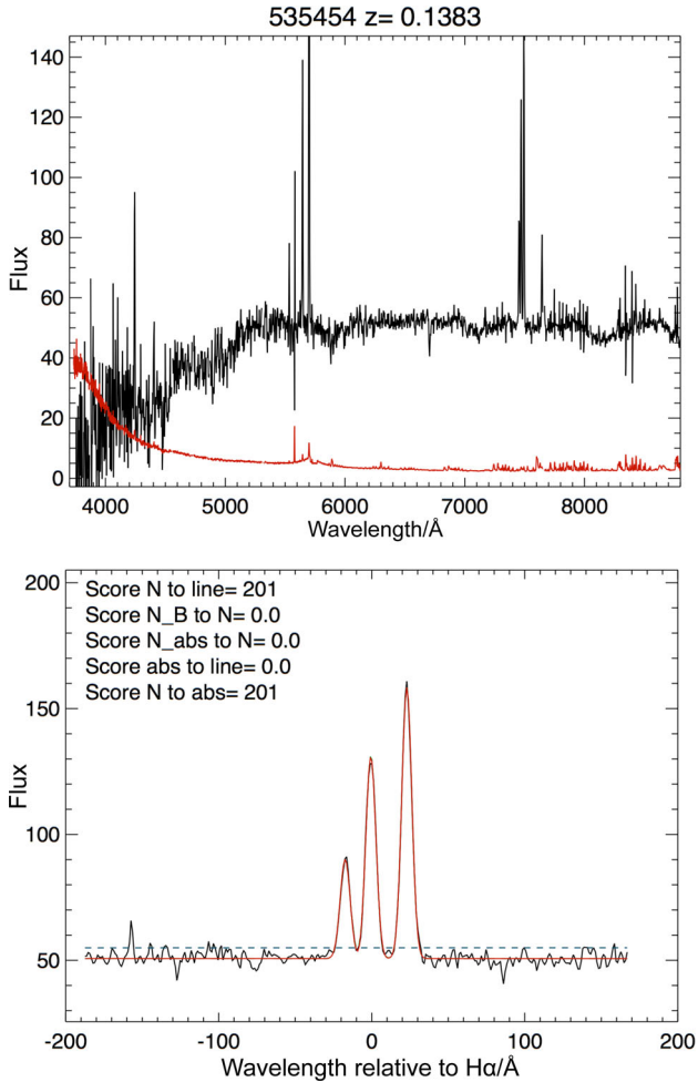
Figure 1. Example of Gaussian fit to a narrow H\alpha emission line. Top: AAOmega spectrum of the galaxy (GAMA CATAID = 535454). Bottom: fitting of the 6398–6710 Å region containing H\alpha and the two [N\text{II}] lines. The scores in the top left of the bottom panel are the model selection scores (see Section 2.3) for the different complexities of fitting model. ‘Line’ is the continuum only model, ‘N’ is the narrow emission model, ‘N_B’ is the narrow + broad emission model, ‘abs’ is the absorption only model, and ‘N_abs’ is the narrow emission + absorption model. The score of 201 involving the narrow model and either just the continuum or absorption ‘N to line’ and ‘N to abs’ of 201 indicates that this is the preferred fit.
