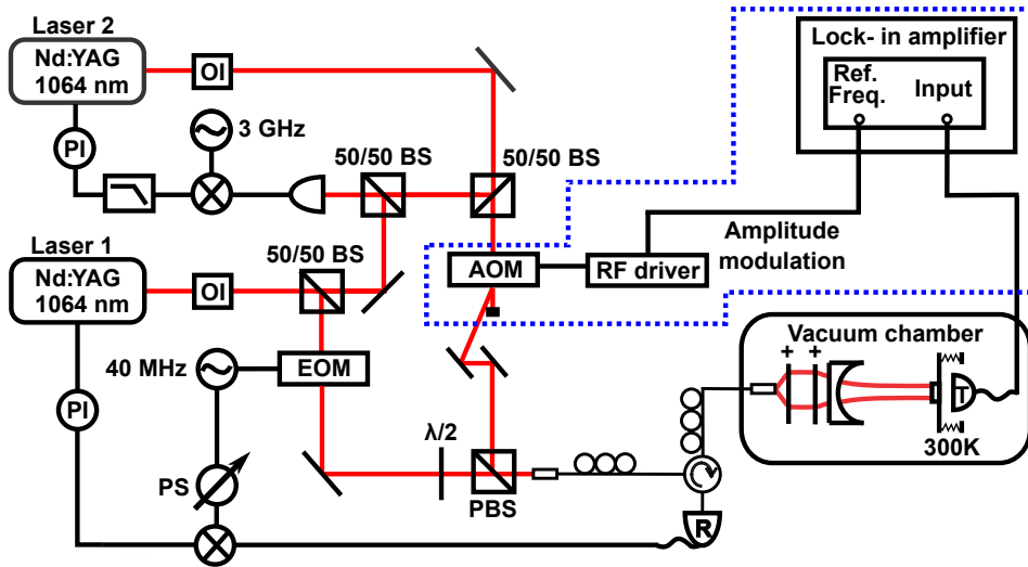
Figure 4.3: Experimental set-up. This is a modified version of the set-up presented by Eerkena et al. [67]. The additional components needed to measure OMIT are highlighted with the dashed blue line. The RF drive signal to the AOM is modulated at the reference frequency of the lock-in amplifier to create a control and two probe beams. The transmitted intensity of the control and probe beams is analyzed using the lock-in amplifier. The components displayed are: LO: local oscillator, BS: beam splitter, PBS: polarizing beam splitter, EOM: electro-optical modulator, OI: optical isolator and PI: proportional-integral feedback controller
