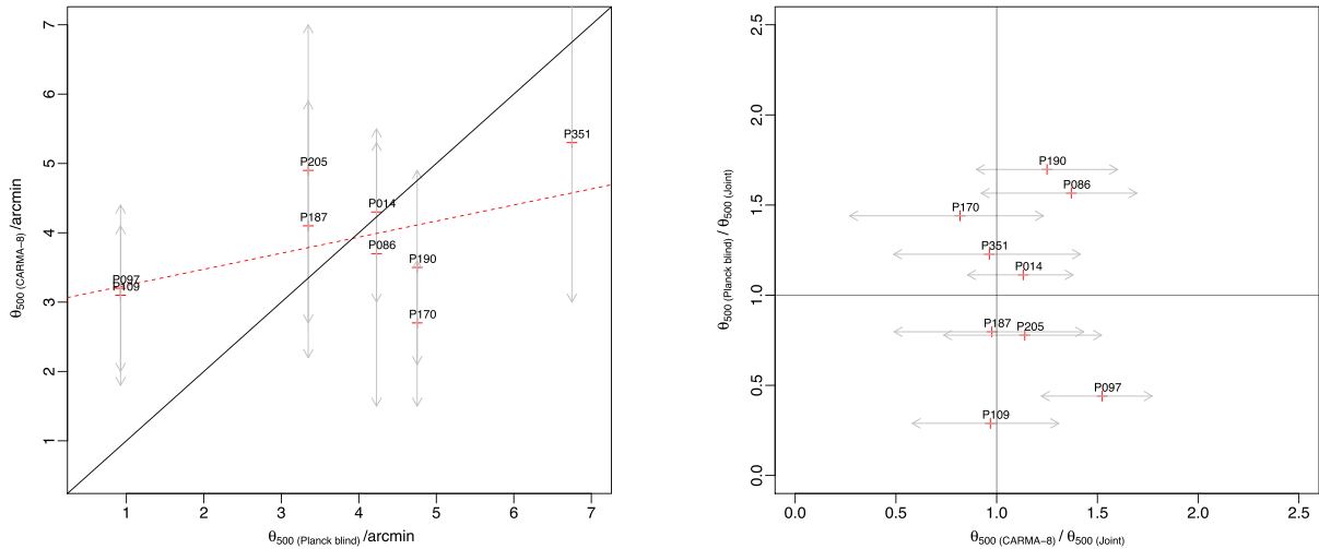
Figure 8. Left: \theta_{500} measured by CARMA-8 against the blind \text{Planck} \theta_{500} . Uncertainties on the \text{Planck} , blind \theta_{500} are not included as they are determined by the large FWHM of the \text{Planck} beam and can range up to 10 arcmin. The best-fitting (red, dotted) and 1:1 (black, solid) lines are included in this plot. Right: ratio of the blind \text{Planck} \theta_{500} and the joint \theta_{500} against the ratio of the CARMA-8 \theta_{500} and the joint \theta_{500} . No strong systematic differences are seen between the different \theta_{500} estimates. The higher resolution of the CARMA-8 data allows \theta_{500} to be constrained much more strongly than using \text{Planck} data alone.
