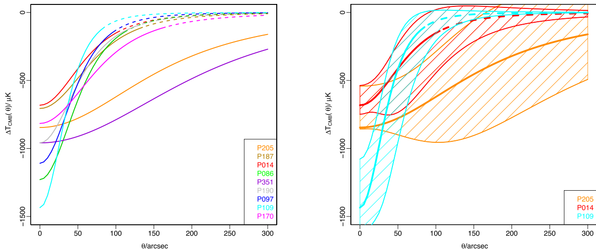
Figure 3. Left: radial brightness temperature profiles derived from equation (11) using the cluster parameter values ( \Delta T_0 , \beta and \theta_c ) from fits of model II to the CARMA-8 data (as provided in Table 9). When the profile has dropped to three times the noise in the SB data, the lines turn from solid to dashed. In the legend, the cluster candidates have been ordered by decreasing Y_{500} (Table 3), although it should be noted that for some clusters, the difference in Y_{500} is small. Shallower profiles with the most negative \Delta T_0 values and largest \theta_{500} values should correspond to the largest Y_{500} from model I. Comparing the volume-integrated brightness temperature profile, \int T(\theta)4\pi\theta^2 d\theta for each cluster from 0 to its \theta_{500} (from model I; Table 3) with Y_{500} (model I), shows reasonable correspondence for most systems, with the exception of P351 and P187. Right: best-fitting radial brightness temperature profiles for three clusters, P205, P014 and P109, which span a range of profile shapes (in thick solid lines, same as the corresponding lines in the left panel). However, here we include the upper and lower 68 per cent-confidence limits of each brightness temperature profile in thin solid lines and highlight the region between these limits with diagonal lines. This shows that according to the parameter fits to CARMA-8 data from model II, the clusters in our sample exhibit a heterogeneous set of profiles, distinguishable despite the uncertainty. Furthermore, high-resolution SZ data or X-ray data may be insensitive to the large signal from the outer parts of the cluster and introduce an additional uncertainty in the derivation of Y_T , an issue which is addressed through a joint analysis with the Planck data.
