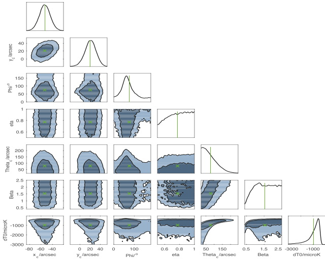
Figure 2. 1D and 2D marginalized distributions for the sampling parameters of our \beta parametrization for P190. The mean is depicted as a green cross and as a line in the 2D and the 1D plots, respectively.
