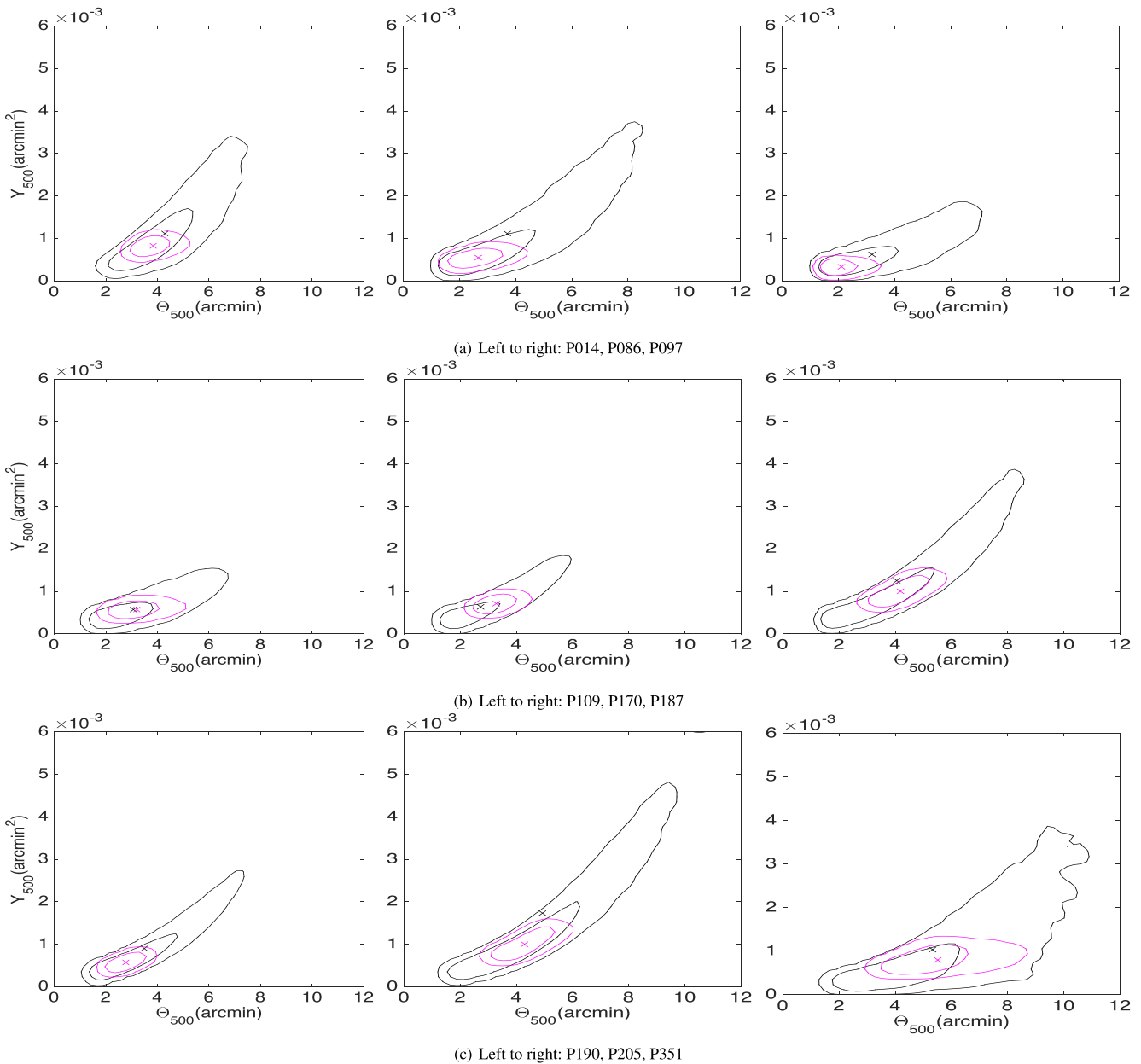
Figure 4. 2D posterior distributions in the Y_{500} – \theta_{500} plane for the CARMA-8 data alone in black contours and for the CARMA-8 data using a Planck prior on Y_{500} (column 4 in Table 11), in magenta contours, to which we refer to as the joint CARMA– Planck constraints. The y-axis is Y_{500} in units of \text{arcmin}^2 and the x-axis is \theta_{500} in units of arcmin. The lower and upper limits of the y-axis are 0 and 0.006 \text{ arcmin}^2 , labelled in steps of 0.001 \text{ arcmin}^2 and for the x-axis, they are 0–12 arcmin, labelled in steps of 2 arcmin. The inner and outer contours in each set indicate the areas enclosing the 68 per cent and 95 per cent of the probability distribution. For all the candidate clusters, there is a dramatic improvement in Y_{500} – \theta_{500} uncertainties when the CARMA and Planck data are jointly analysed to yield cluster parameters.
