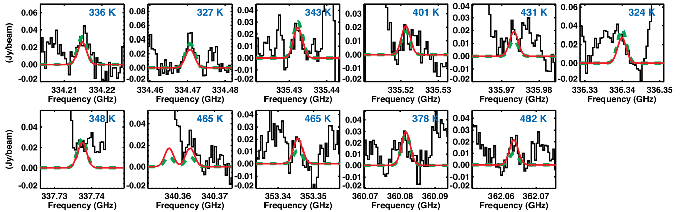
Figure 4. Black: detected unblended lines of CH 3 NCO towards source A. Red solid: best-fitting model for T_{\text{ex}} = 300 K. Green dashed: best-fitting model for T_{\text{ex}} = 100 K. The E_{\text{up}} values of the lines are indicated in blue in the right upper part of each panel.
