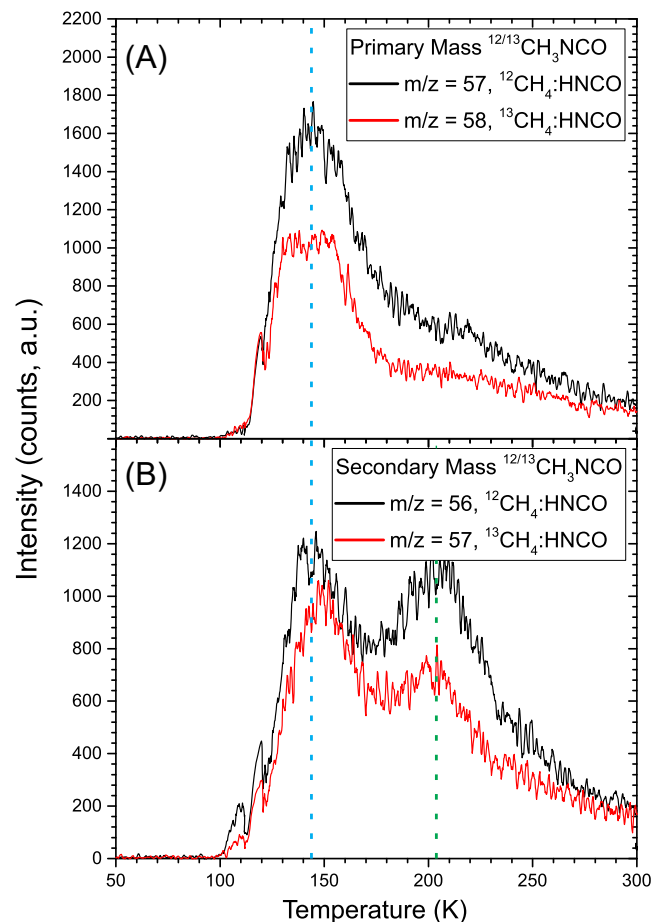
Figure 6. TPD trace of the primary (A) and secondary (B) masses of ^{12/13}\text{CH}_3\text{NCO} . Both the primary and secondary masses are seen being released around 145\text{ K} (blue line). The secondary mass shows another release peak around 205\text{ K} (green), which is suspected to also contribute to first release peak, thus altering respectively the m/z 57/56 and 58/57 ratio.
