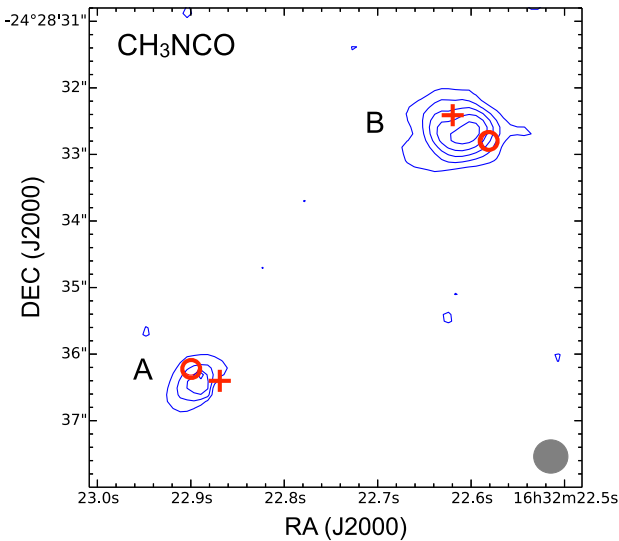
Figure 2. Integrated intensity map of the \text{CH}_3\text{NCO} 39_{0,39,0}-38_{0,38,0} transition at 336 339.9 MHz and E_{\text{up}} = 323.7 K between 1.7 and 3.7 km s ^{-1} . The positions of the continuum of source A (south-east source) and source B (north-west source) are indicated with red crosses, while the positions studied in this paper are indicated with red circles. The contour levels start at 5\sigma with additional steps of 5\sigma . The circular restoring beam of 0.5 arcsec size is indicated in grey in the right-hand lower corner.
