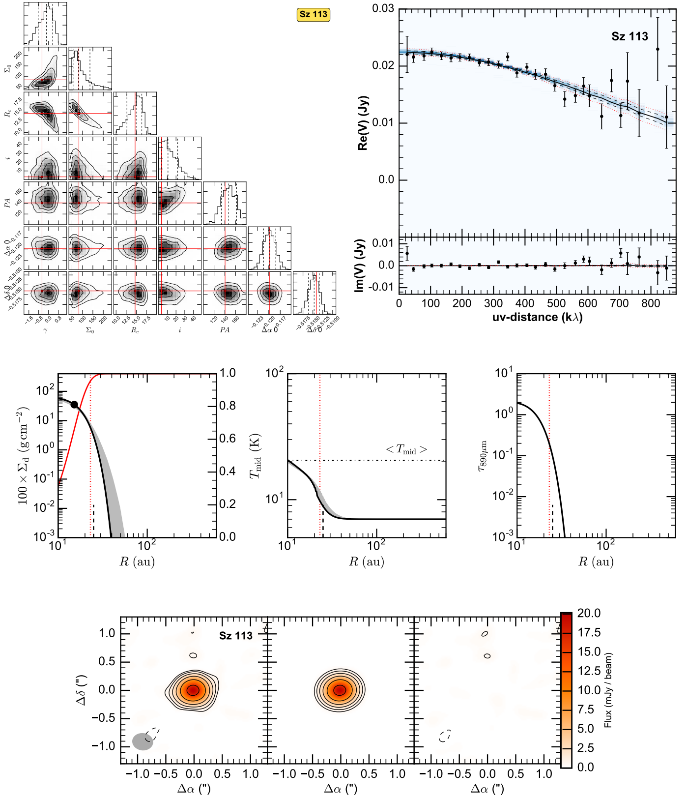
Fig. A.19. Fit results for Sz 113, presented as in Fig. A.1. In the images \sigma = 0.2 mJy/beam.
