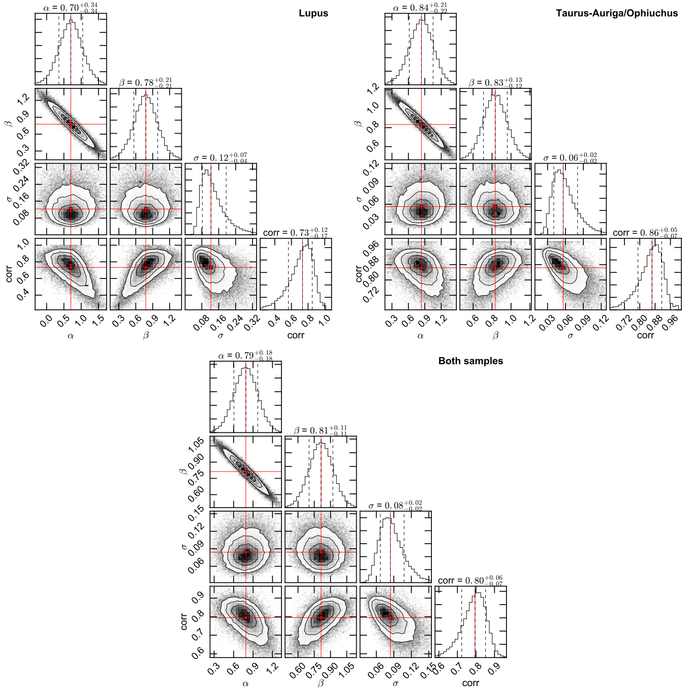
Fig. B.1. Staircase plots showing the posterior PDF resulting from the application of the Bayesian regression method by Kelly (2007) to infer a law \log(F_{890\ \mu\text{m}}) = \beta \log(R_c) + \alpha for the Lupus sample ( top left ), for the Taurus-Auriga and Ophiuchus sample ( top right ) and for both the samples together ( bottom ). Each plot shows the PDF of the intercept ( \alpha ), the slope ( \beta ), the intrinsic scatter of data points ( \sigma ) and the correlation degree ( \text{corr} ). The red lines highlight the posterior peak.
