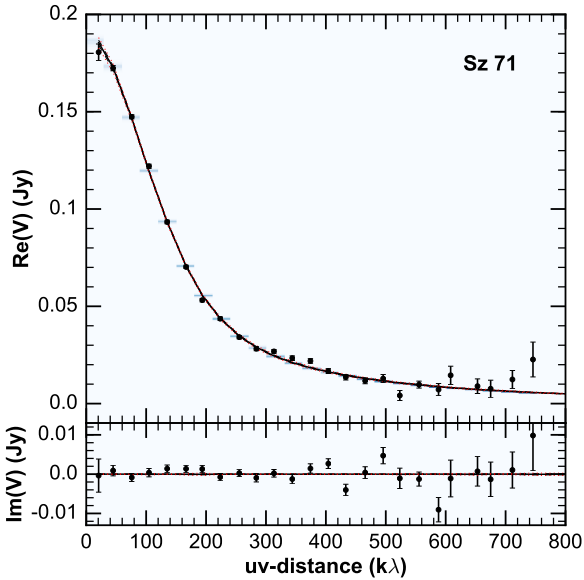
Fig. 5. Comparison between model and observed visibilities of Sz 71 as a function of deprojected baseline length ( uv -distance). The panel above (below) shows the real (imaginary) part of the visibilities. Black dots show the observed visibilities (binned every 30 k \lambda ), the blue density indicators represent the PDF of the model visibilities in each uv -bin. The black solid line corresponds to the median of the model visibilities PDF, the black dashed lines the 16th and 84th percentiles, the red dotted lines the 2.7th and 97.7th percentiles.
