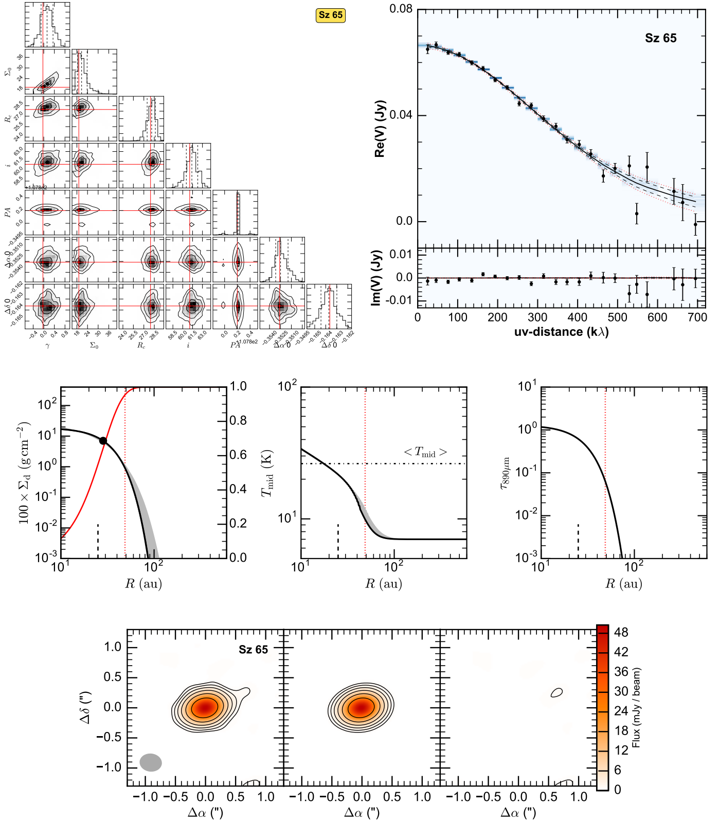
Fig. A.1. Fit results for Sz 65. Top row: on the left, the staircase plot showing the MCMC chains as in Fig. 3; on the right, the comparison of the observations and model deprojected visibilities as a function of uv -distance as in Fig. 5. Middle row: plots showing the physical structure of the disk as in Fig. 4. Bottom row: synthesized images of observations, model and residual visibilities as in Fig. 6. In the images \sigma = 0.27 mJy/beam.
