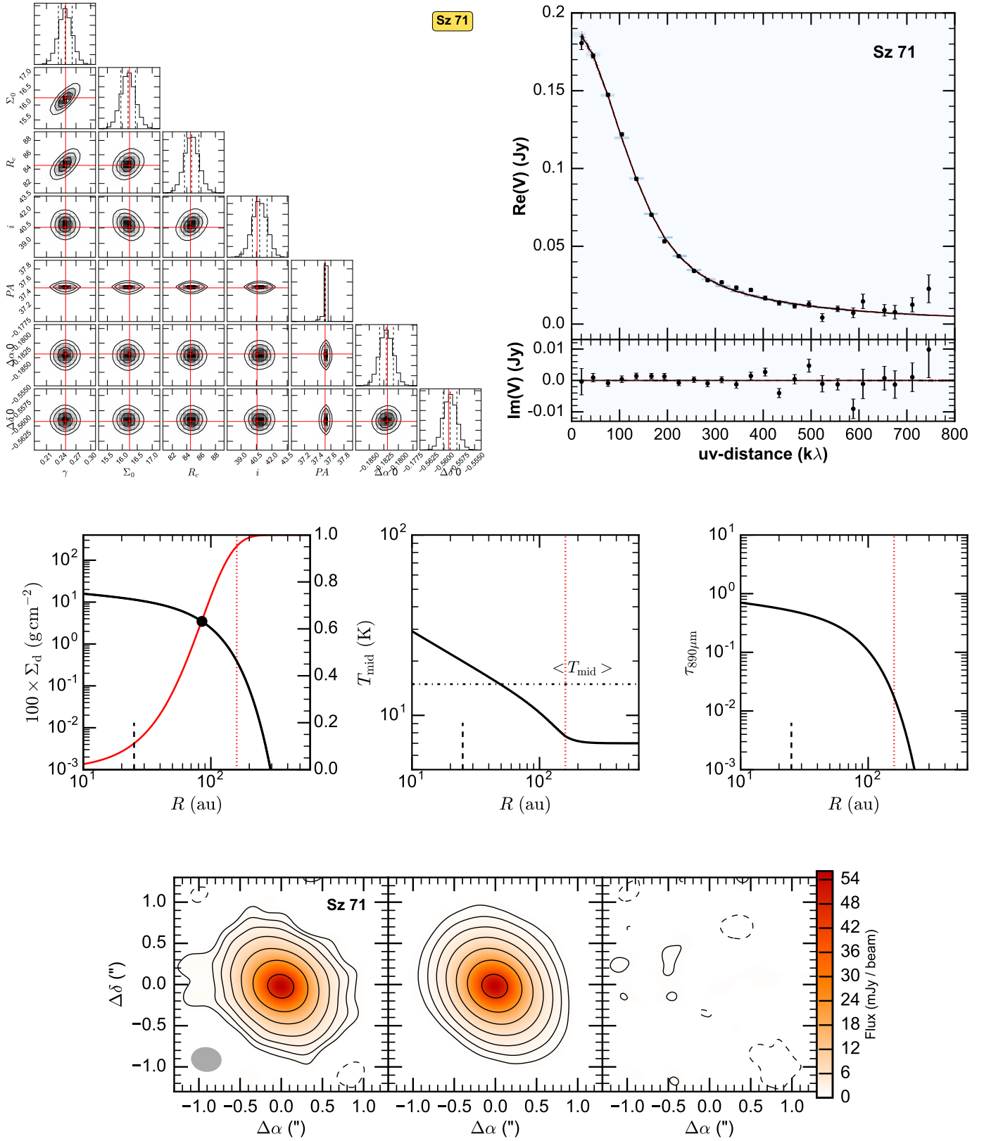
Fig. A.5. Fit results for Sz 71, presented as in Fig. A.1. In the images \sigma = 0.23 mJy/beam.
