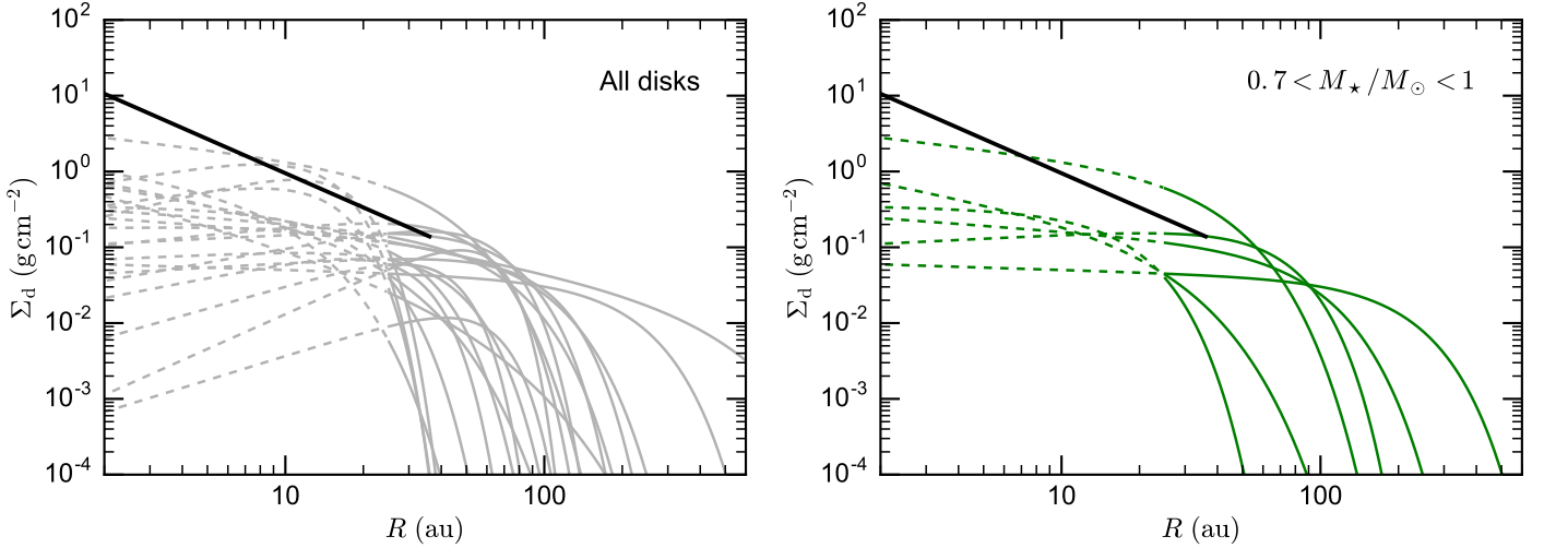
Fig. 13. Left: dust surface density profiles inferred for all the disks in our Lupus sample (gray curves) compared to the Hayashi (1981) dust surface density model for the solar system (black thick line). The inferred surface density profiles are dashed where they are not spatially resolved, that is for R < 25 au. Right: dust surface density profiles for the sources in the 0.7\text{--}1\,M_{\odot} stellar mass bin.
