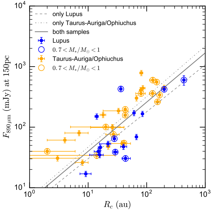
Fig. 11. 890 \mu\text{m} integrated flux (normalized to a common distance of 150 pc) as a function of exponential cut-off radius, constrained by fitting spatially resolved observations with angular resolution better than 0.75'' . For some disks, the 890 \mu\text{m} flux was extrapolated from the measured 1.3 mm flux assuming an average spectral index \alpha = 3.0 . Yellow elements are Taurus-Auriga and Ophiuchus disks from the Andrews (2015) compilation; blue elements are Lupus disks analyzed in this paper. Gray lines represent the correlations found by the Bayesian linear regression for the Taurus-Auriga and Ophiuchus disks (dash-dotted), for the Lupus disks (dashed), and for both the samples taken together (solid).
