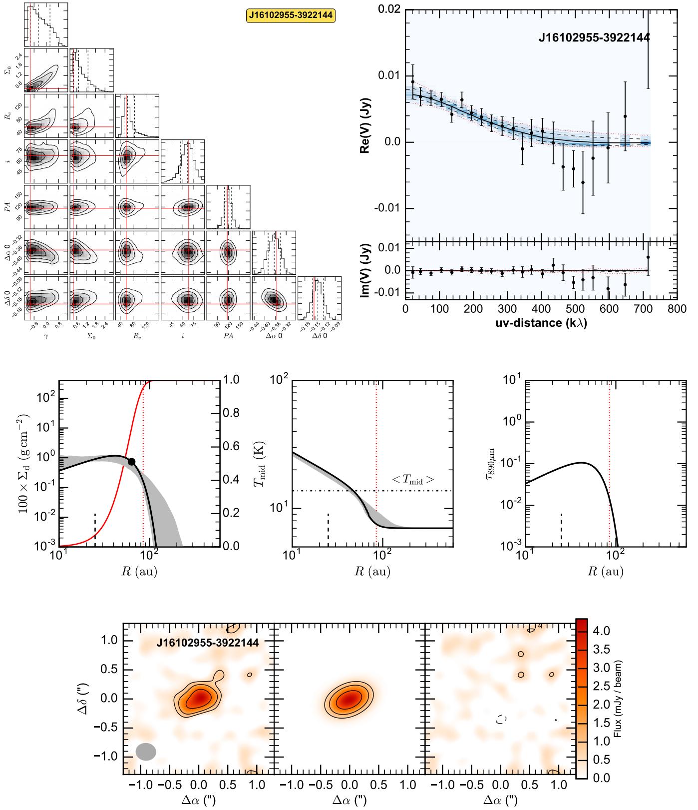
Fig. A.21. Fit results for J16102955-3922144, presented as in Fig. A.1. In the maps, \sigma = 0.25 \text{ mJy/beam} .
