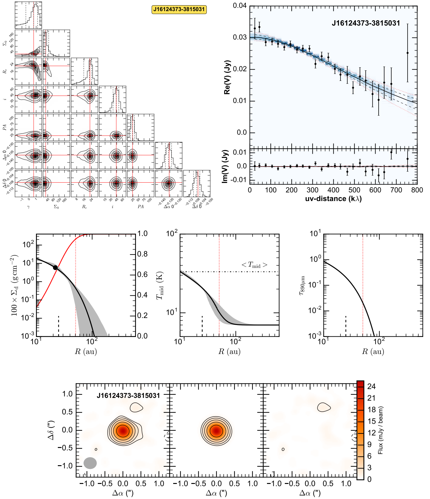
Fig. A.22. Fit results for J16124373-3815031, presented as in Fig. A.1. In the images \sigma = 0.3 mJy/beam.
