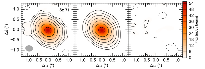
Fig. 6. Comparison between the observed ( left ) and the best-fit model ( middle ) images for Sz 71. Residuals are shown in the right panel. The best-fit model has the following parameters \gamma = 0.25 \pm 0.01 , \Sigma_0 = (16.2 \pm 0.2)\text{g/cm}^2 , R_c = (85 \pm 1)\text{au} . The three images have been produced by applying the CLEAN deconvolution algorithm with natural weighting to the observed, best-fit model and residual visibilities, respectively. Contour levels refer to -3 (dashed), 3, 6, 12, 24, 48, 50, 100, 150, etc. multiple of the rms, which here is \sigma = 0.3 mJy/beam. The FWHM of the synthesized beam is shown as a gray ellipse in the left panel.
