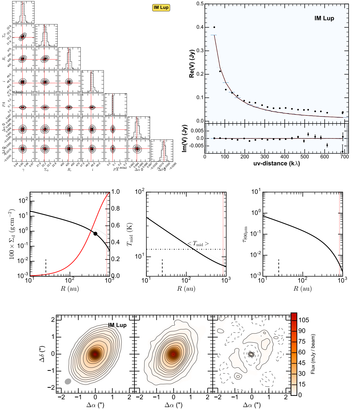
Fig. A.7. Fit results for IM Lup, presented as in Fig. A.1. In the images \sigma = 0.6 mJy/beam.
