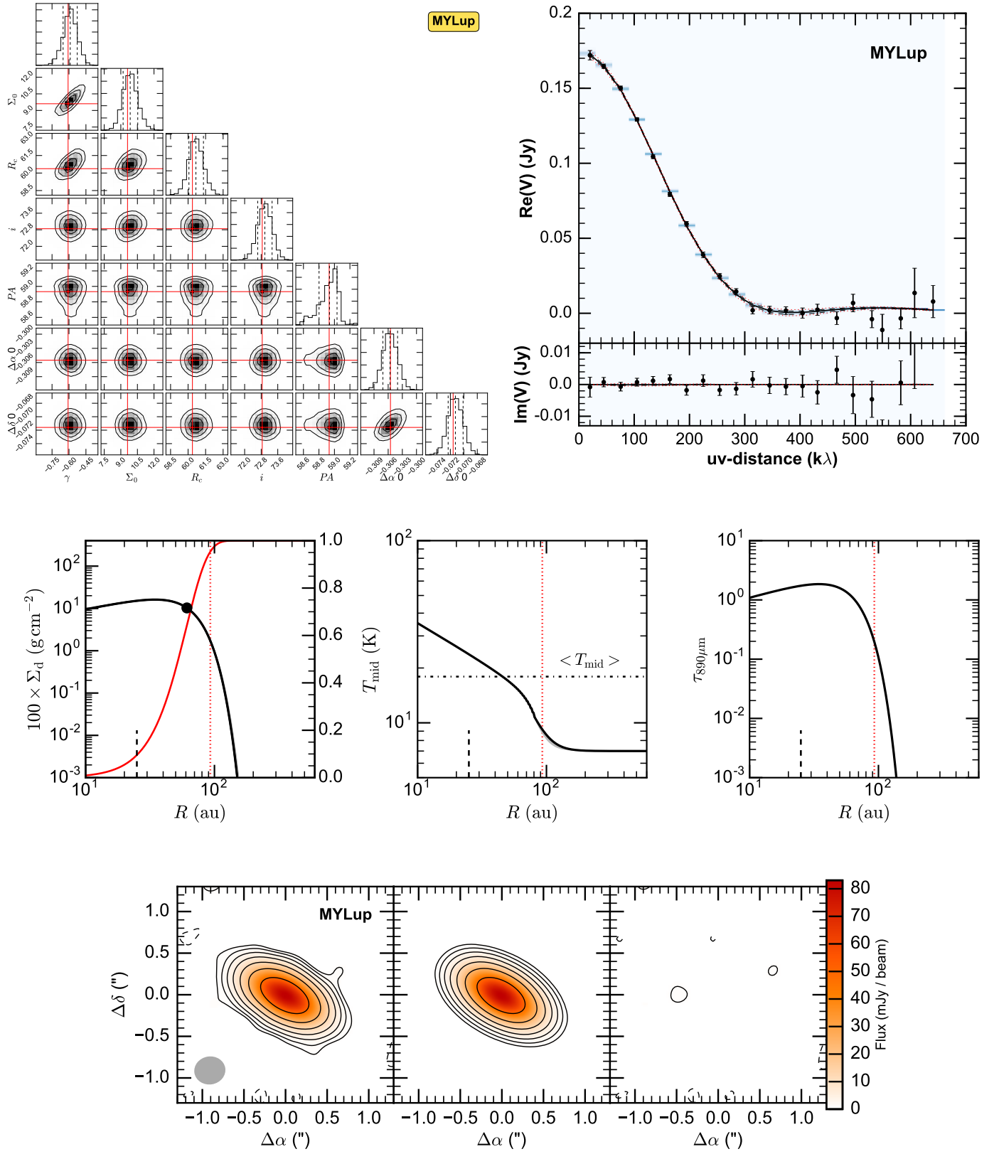
Fig. A.12. Fit results for MY Lup, presented as in Fig. A.1. In the images \sigma = 0.25 mJy/beam.
