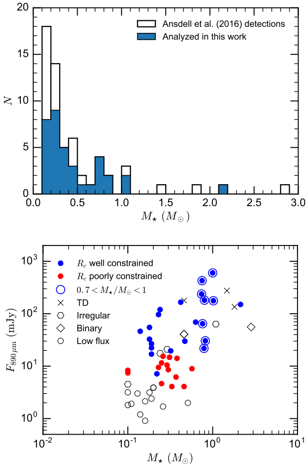
Fig. 1. Top: distribution of stellar masses for the full Lupus sample from Ansdell et al. (2016) (white bars) and for the sub-sample analyzed in this work (blue bars). Bottom: observed integrated continuum flux at 890 \mu\text{m} (Ansdell et al. 2016) as a function of stellar mass. Blue dots represent sources whose analysis is presented in this work. Red dots represent sources that appear unresolved and have been discarded in the rest of the analysis due to low signal-to-noise ratio. In this and subsequent plots, the circled dots highlight sources in the 0.7–1 M_{\odot} mass bin. We also report transition disks (“x” symbols), sources with irregular shape (hexagons), binaries (diamonds), and the sources with integrated flux F_{\text{cont}} < 4 \text{ mJy} that we excluded from our analysis (empty circles).
