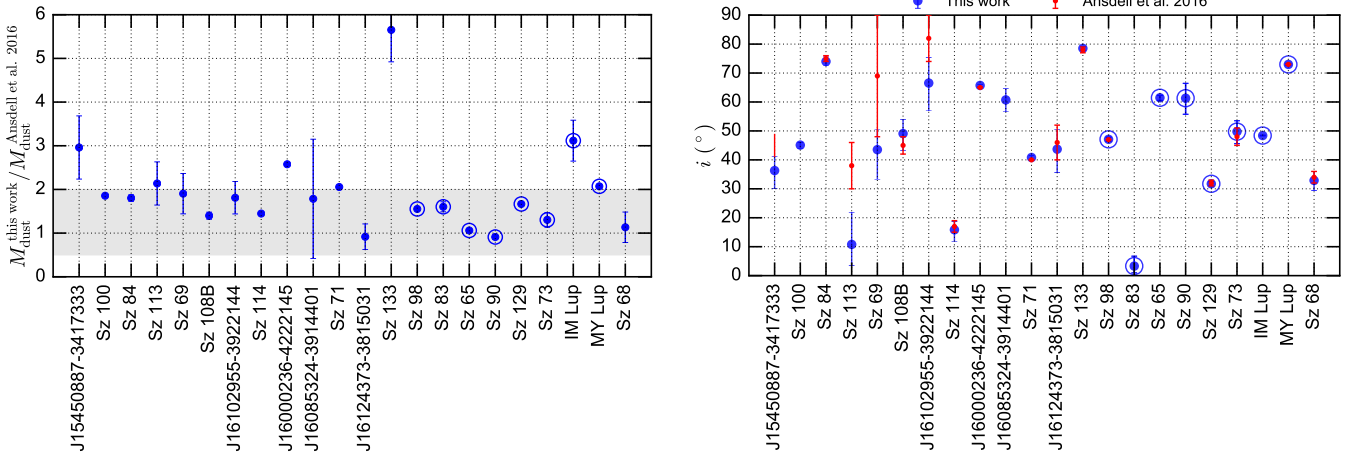
Fig. 7. Left: ratio between the dust masses derived in this work and those derived by Ansdell et al. (2016) . Although derived with very different methods (for a detailed description, see the text), the masses are within a factor of 2 (gray area) for the vast majority of disks. Right: comparison between the disk inclinations i (along the line of sight) obtained in this work and those derived by Ansdell et al. (2016) . In both plots, the disks are sorted from left to right by increasing stellar mass and the circled dots highlight sources with 0.7 \leq M_*/M_\odot \leq 1 .
