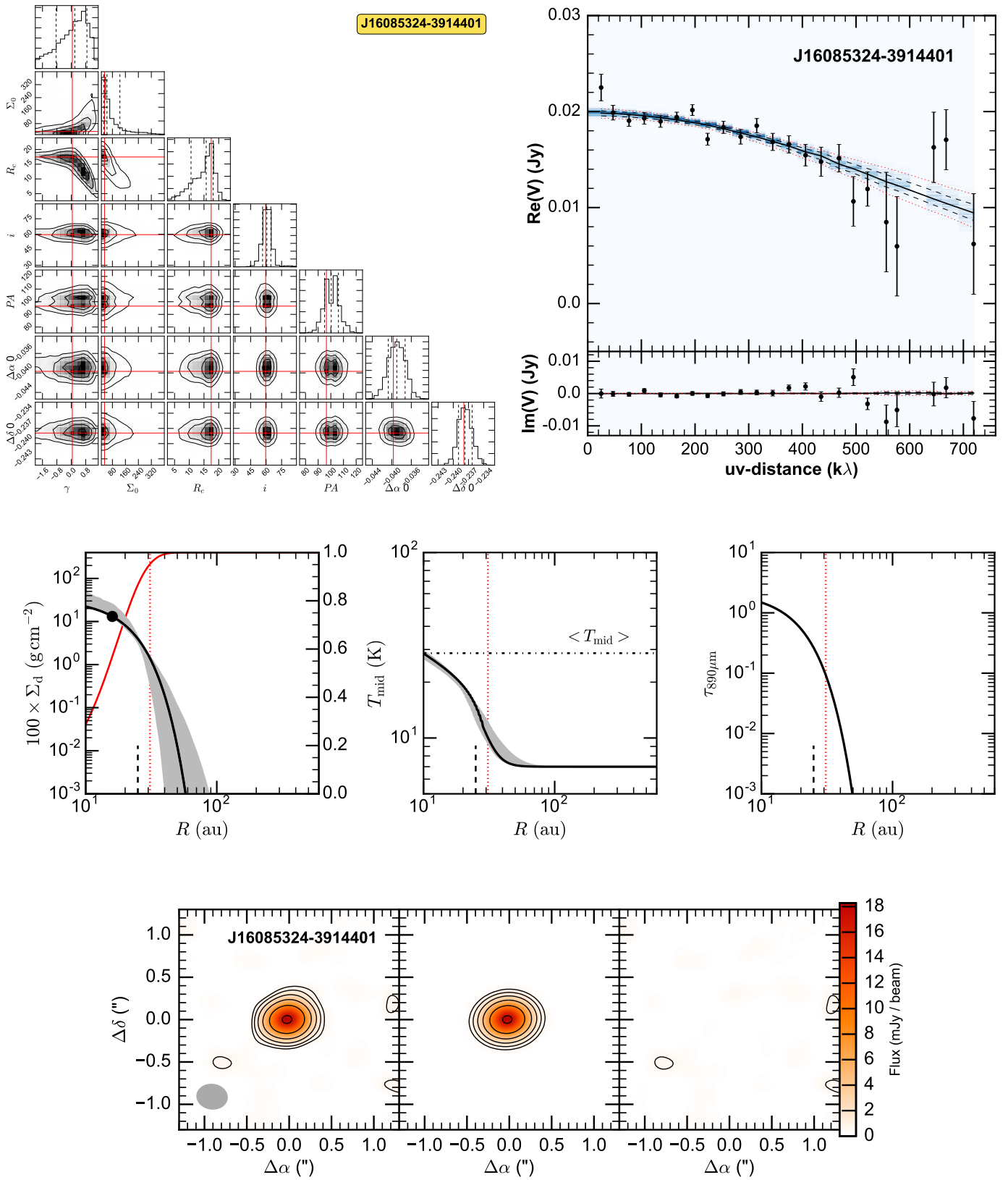
Fig. A.18. Fit results for J16085324-3914401, presented as in Fig. A.1. In the images \sigma = 0.2 mJy/beam.
