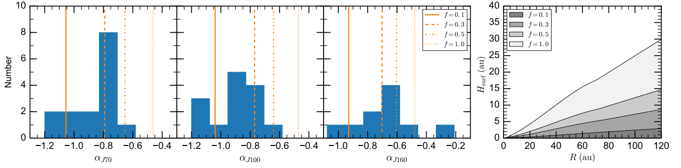
Fig. 2. Left: spectral indices for the sources in our sample measured between J -band (2MASS, 1.235\,\mu\text{m} ) and, respectively, 70\,\mu\text{m} , 100\,\mu\text{m} , 160\,\mu\text{m} (Herschel/PACS) using the definition in Eq. (3). The vertical lines show the spectral indices obtained with our disk model for different values of the flaring reduction parameter f , from a fully-flared model ( f = 1 , dotted line) to less flared models ( f = 0.5, 0.3, 0.1 , respectively dash-dotted, dashed and solid line). Right: scale-height of the disk surface layer computed by the model.
