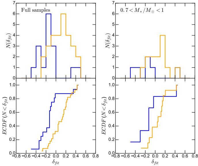
Fig. 12. Top panels: distribution of the parameter \delta_{\text{fit}} (see text) for the Lupus (blue) and Taurus-Auriga and Ophiuchus (yellow) samples. In the left panel we show the full samples, while in the right one we restrict to the range 0.7 \leq M_*/M_\odot \leq 1 . Bottom panels: empirical cumulative distribution functions for the values of \delta_{\text{fit}} for the same samples as in the upper panels.
