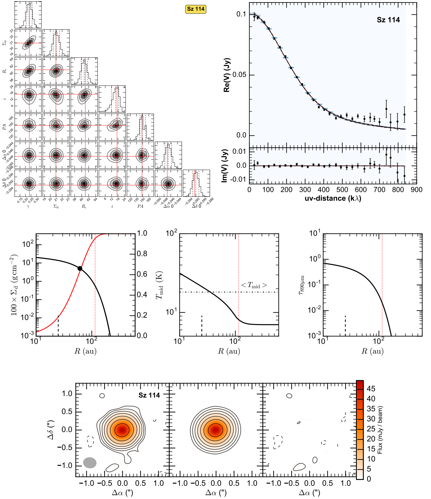
Fig. A.20. Fit results for Sz 114, presented as in Fig. A.1. In the images \sigma = 0.2 mJy/beam.
