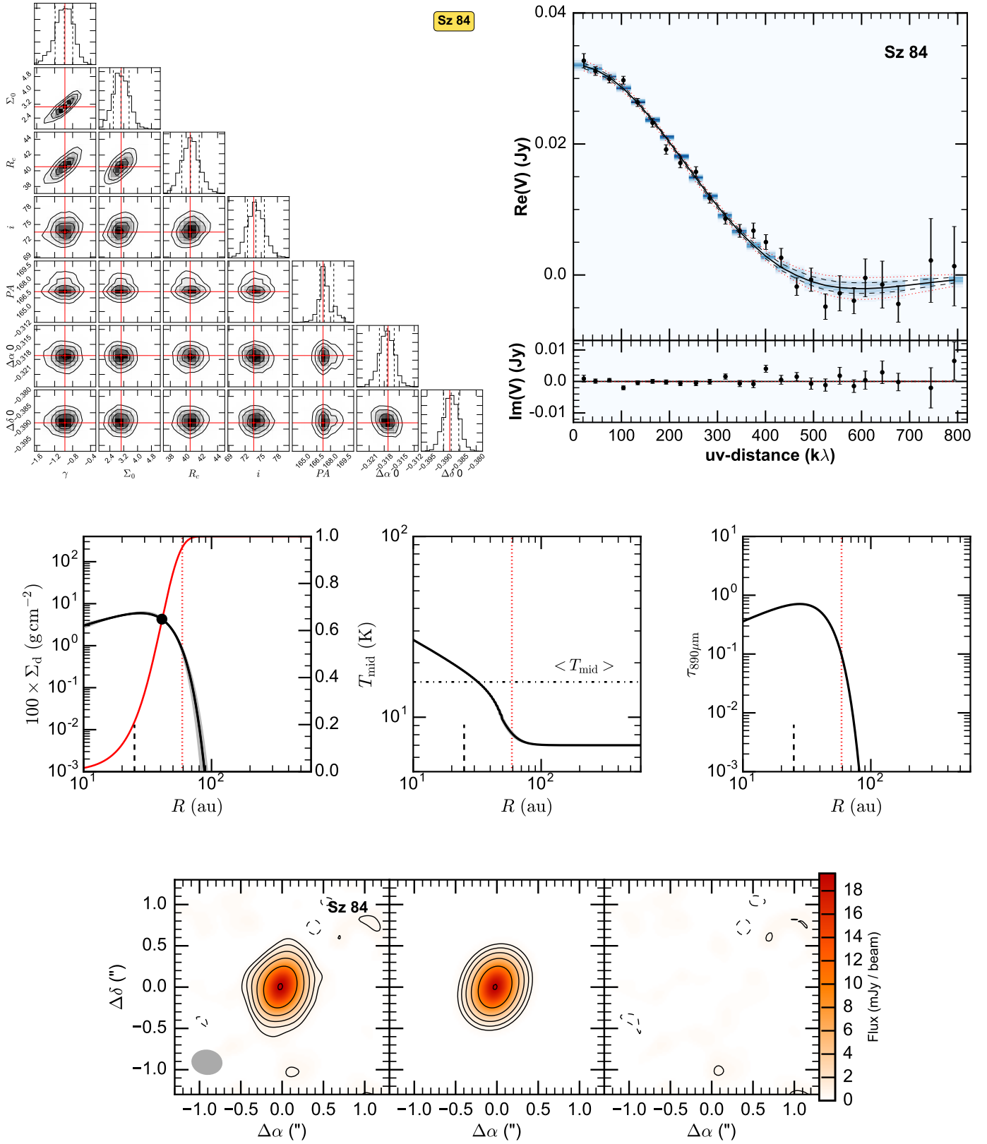
Fig. A.9. Fit results for Sz 84, presented as in Fig. A.1. In the images \sigma = 0.2 mJy/beam.
