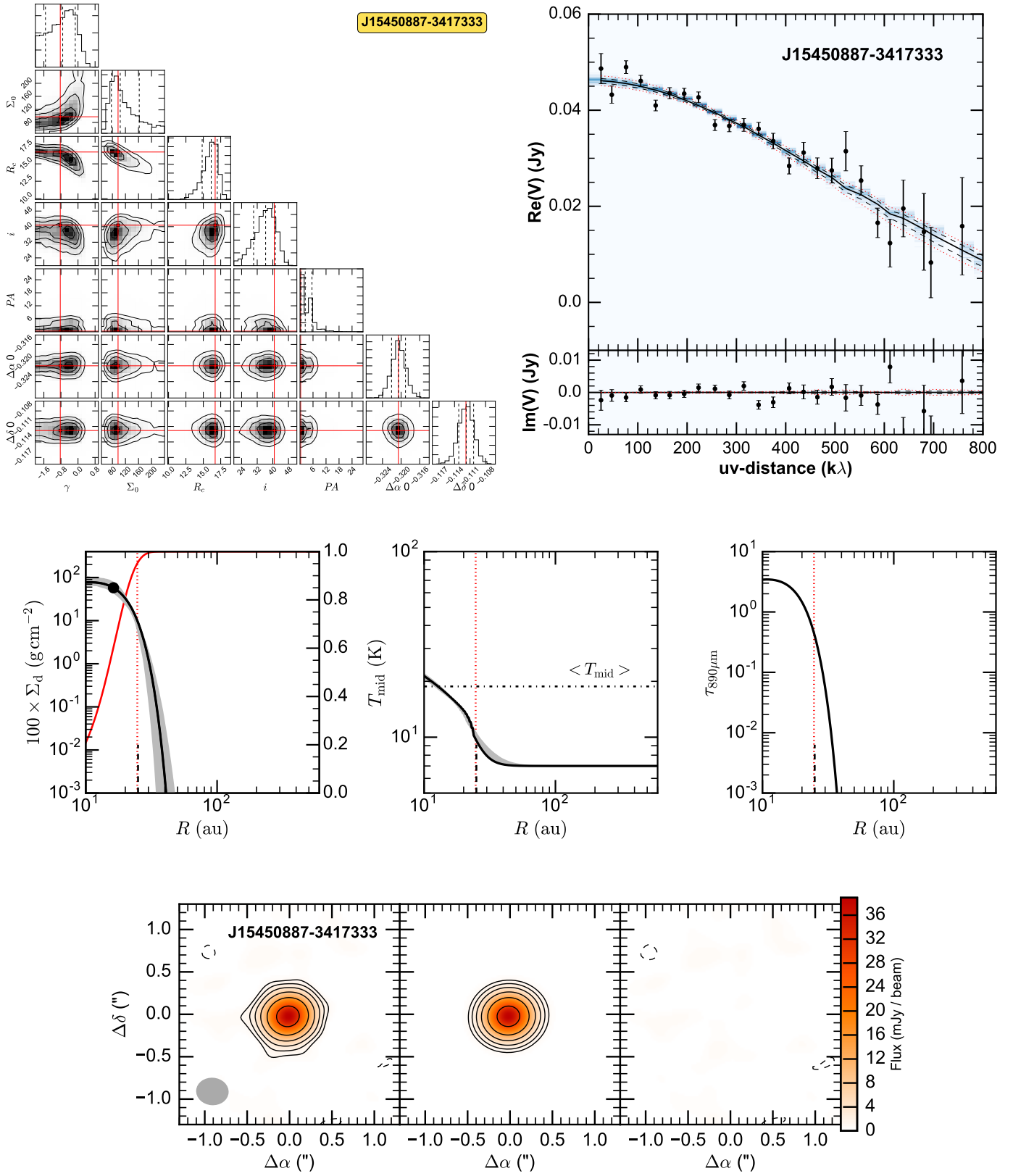
Fig. A.2. Fit results for J15450887-3417333, presented as in Fig. A.1. In the images \sigma = 0.3 mJy/beam.
