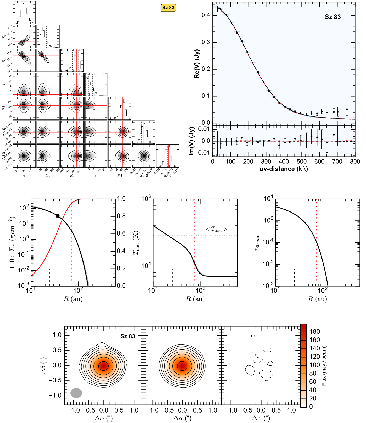
Fig. A.8. Fit results for Sz 83, presented as in Fig. A.1. In the images \sigma = 0.4 mJy/beam.
