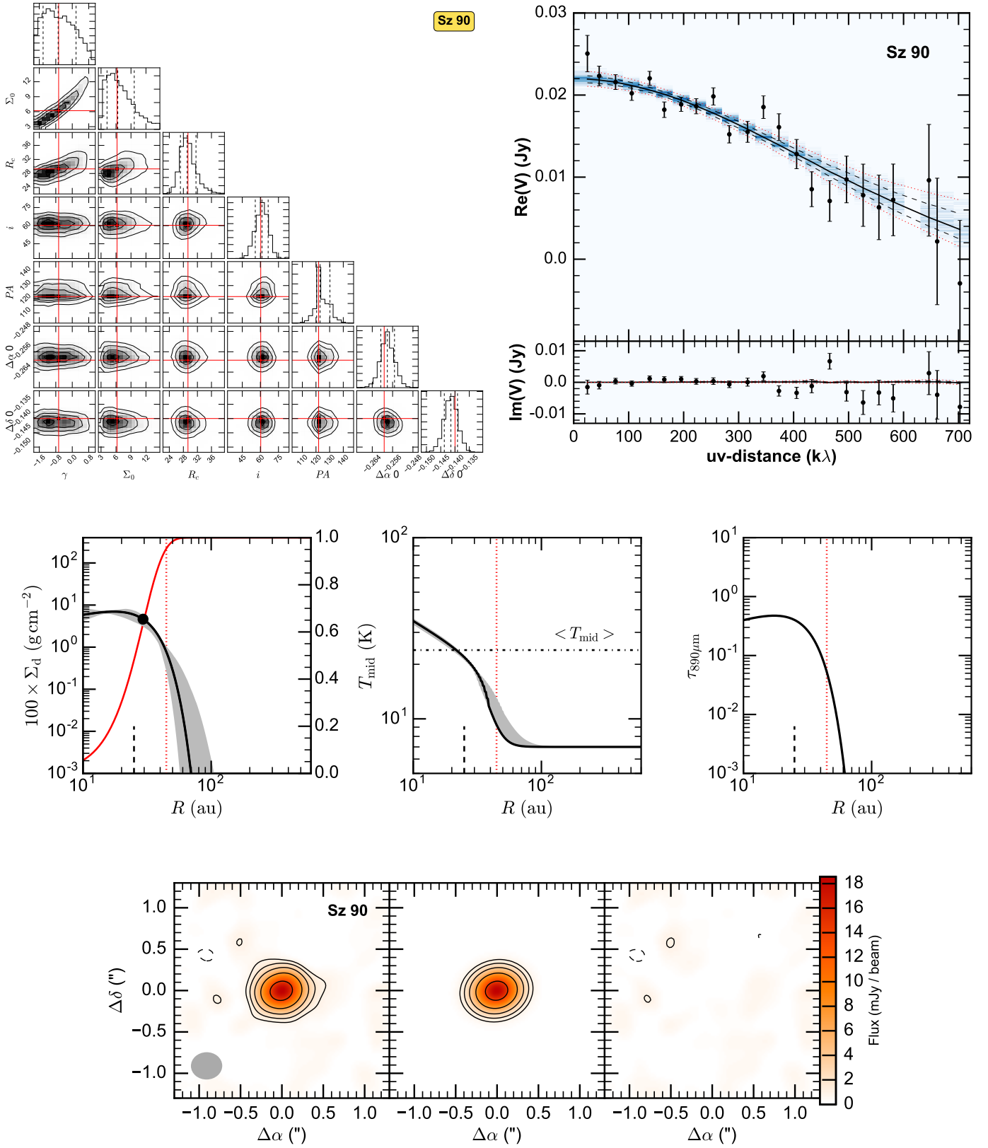
Fig. A.14. Fit results for Sz 90, presented as in Fig. A.1. In the images \sigma = 0.3 mJy/beam.
