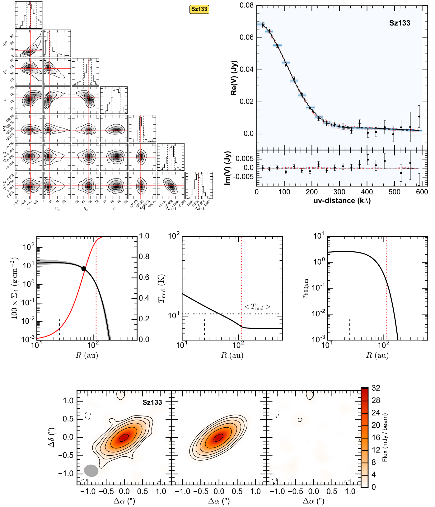
Fig. A.13. Fit results for Sz 133, presented as in Fig. A.1. In the images \sigma = 0.3 mJy/beam.
