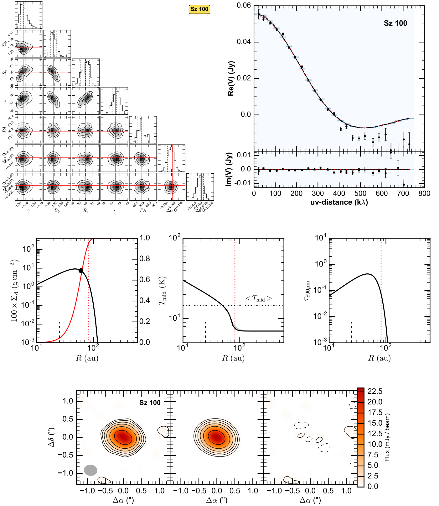
Fig. A.16. Fit results for Sz 100, presented as in Fig. A.1. In the images \sigma = 0.2 mJy/beam.
