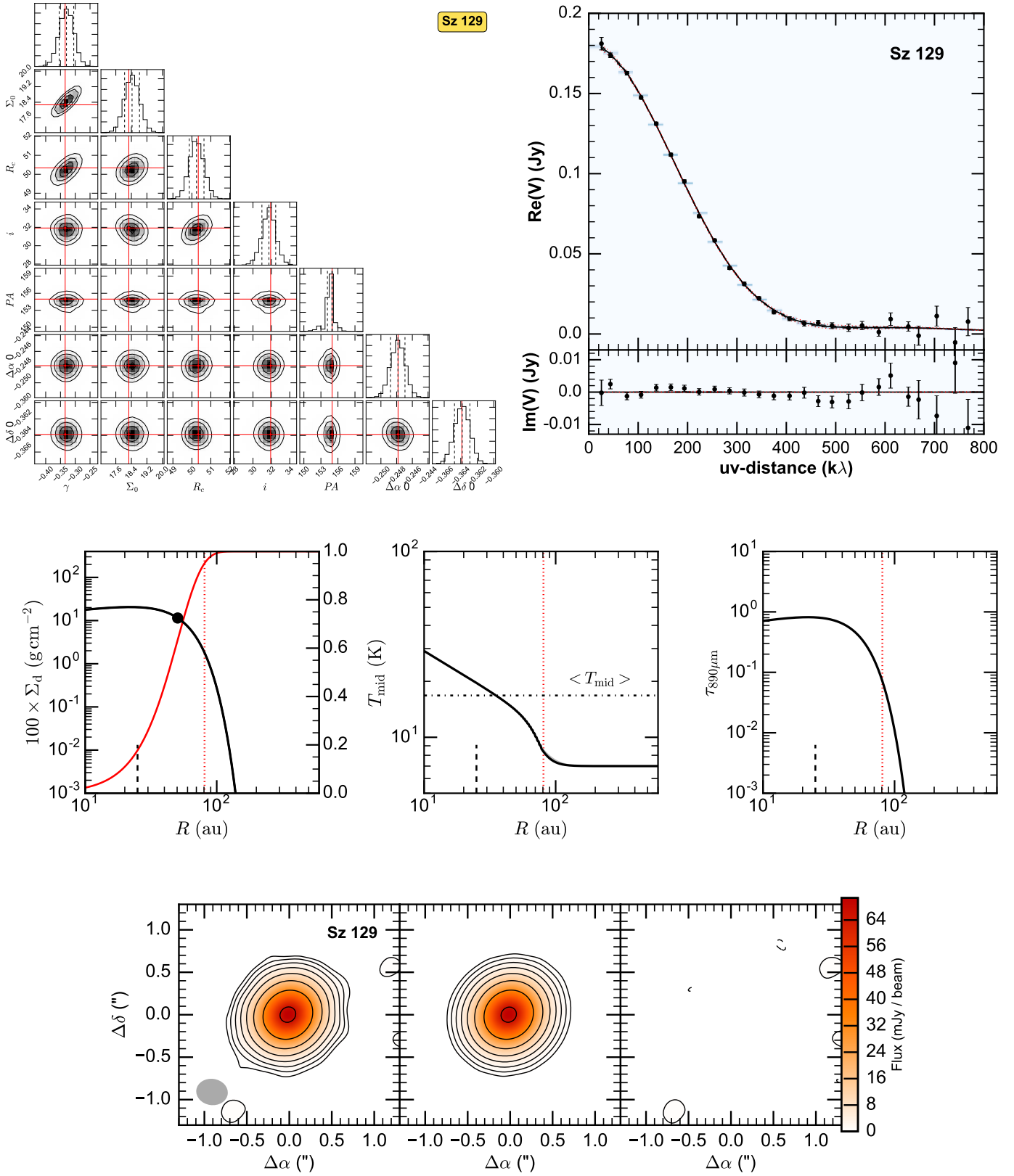
Fig. A.10. Fit results for Sz 129, presented as in Fig. A.1. In the images \sigma = 0.2 mJy/beam.
