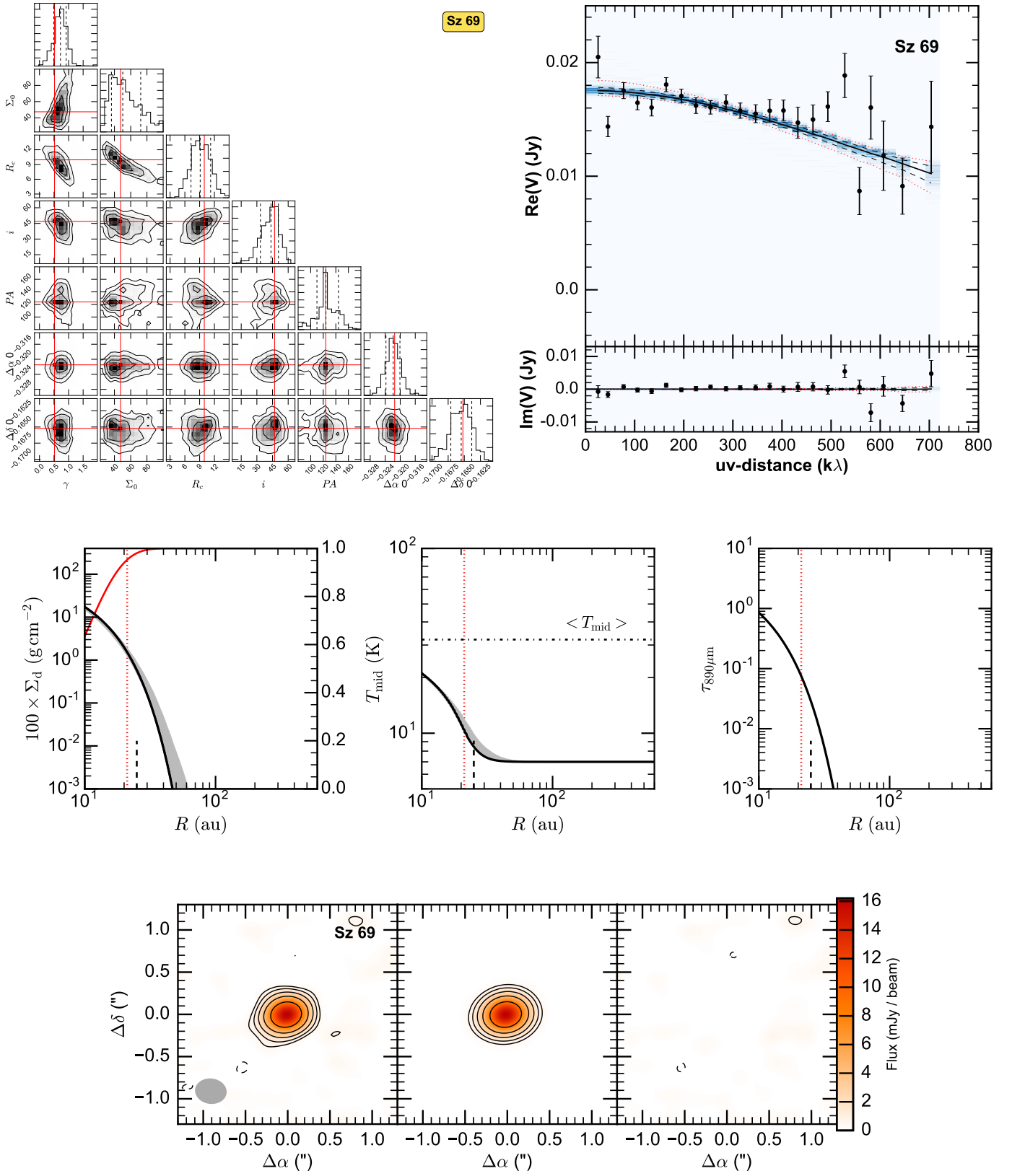
Fig. A.4. Fit results for Sz 69, presented as in Fig. A.1. In the images \sigma = 0.25 mJy/beam.
