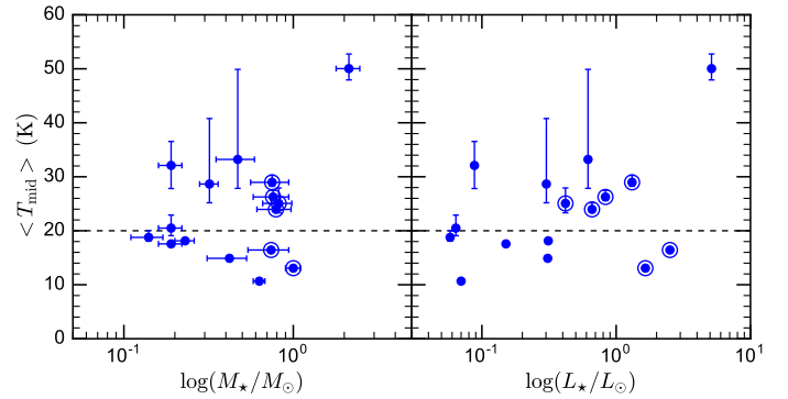
Fig. 8. Mass-averaged midplane temperature as a function of stellar mass ( left ) and luminosity ( right ) for the disks for which we derive a reliable disk structure. Error bars on the y -axis reflect the distribution of models obtained from the fits. In more than half disks we find a disk temperature smaller than T_d = 20 \text{ K} used by Ansdell et al. (2016) .
