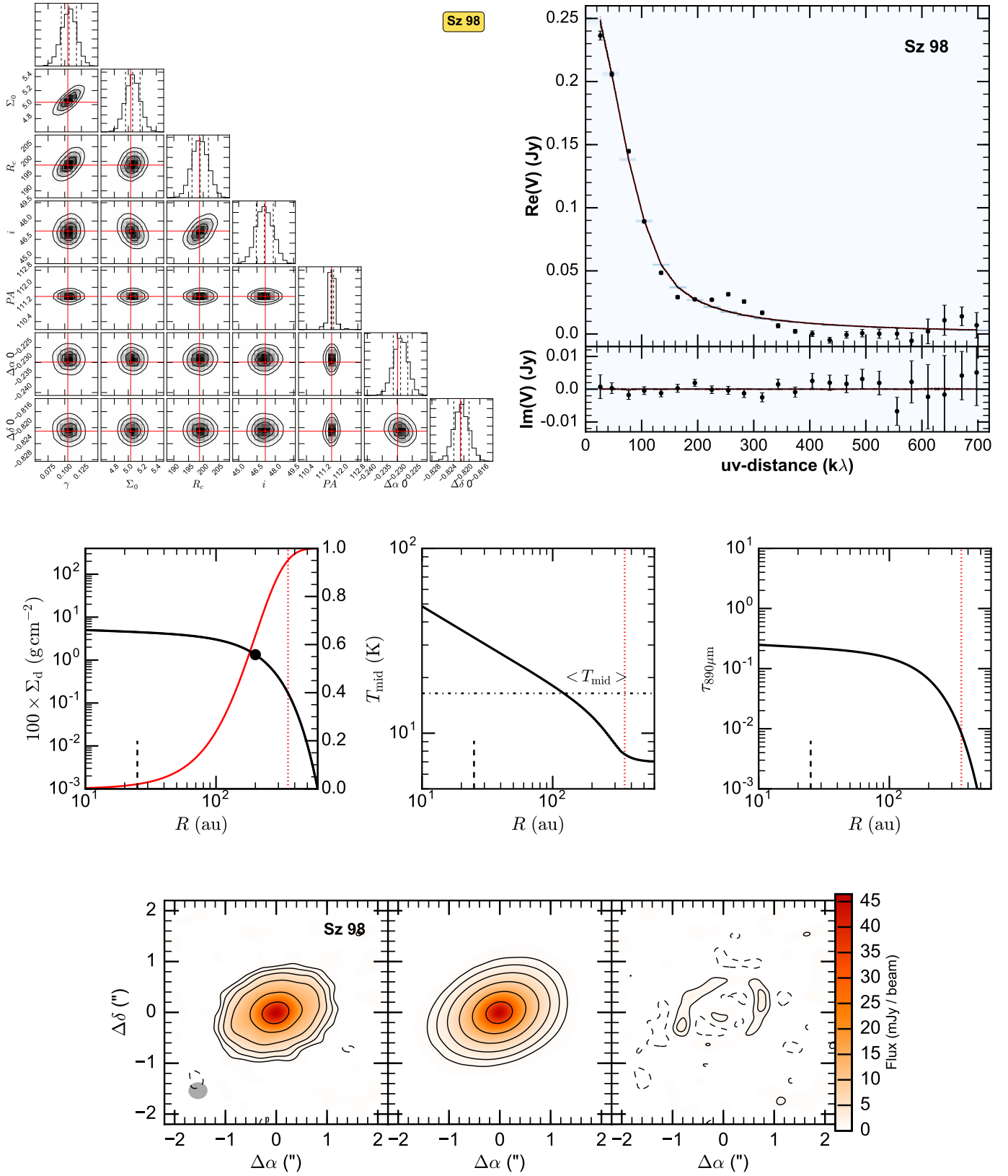
Fig. A.15. Fit results for Sz 98, presented as in Fig. A.1. In the images \sigma = 0.33 mJy/beam.
