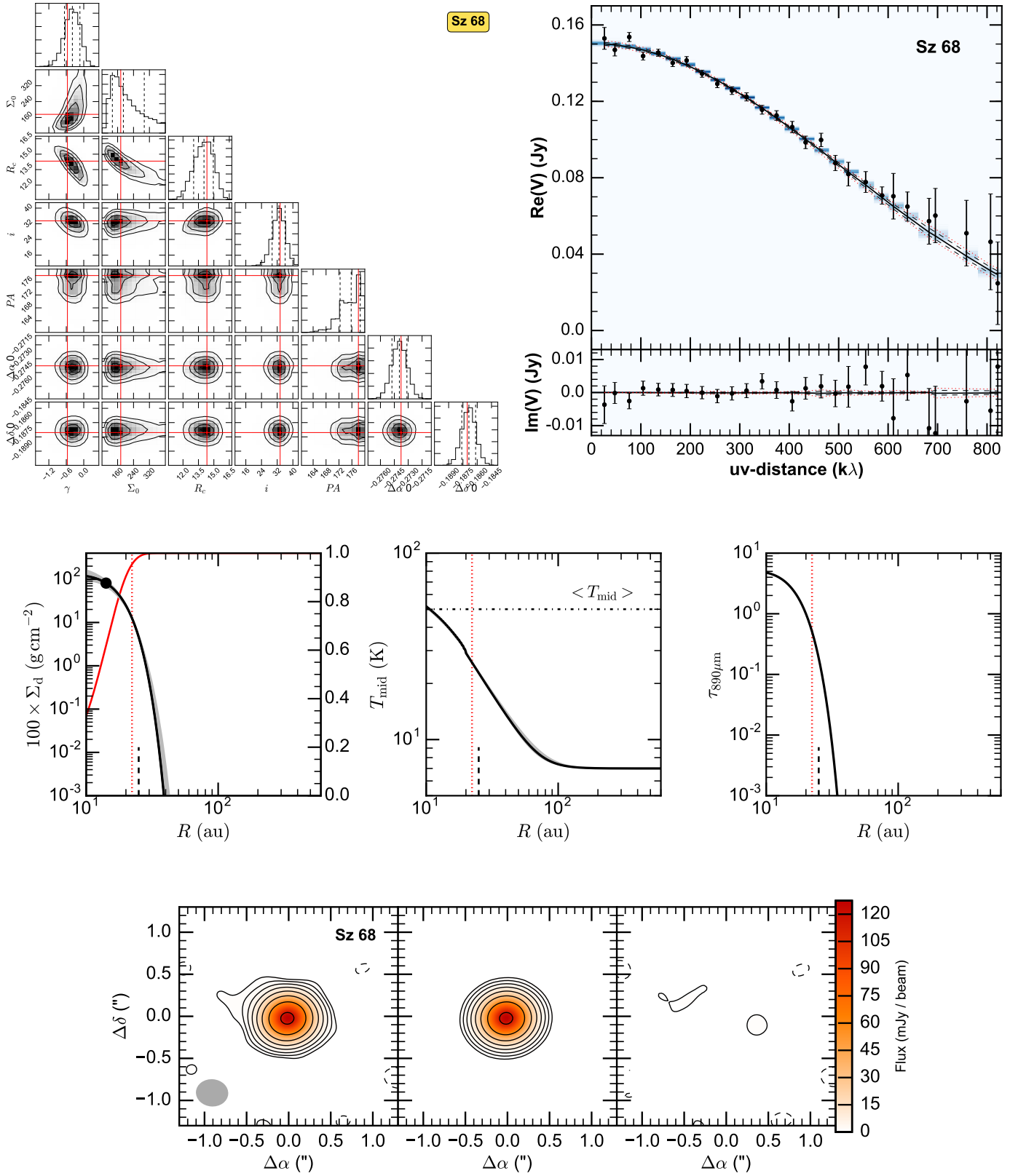
Fig. A.3. Fit results for Sz 68, presented as in Fig. A.1. In the images \sigma = 0.3 mJy/beam.
