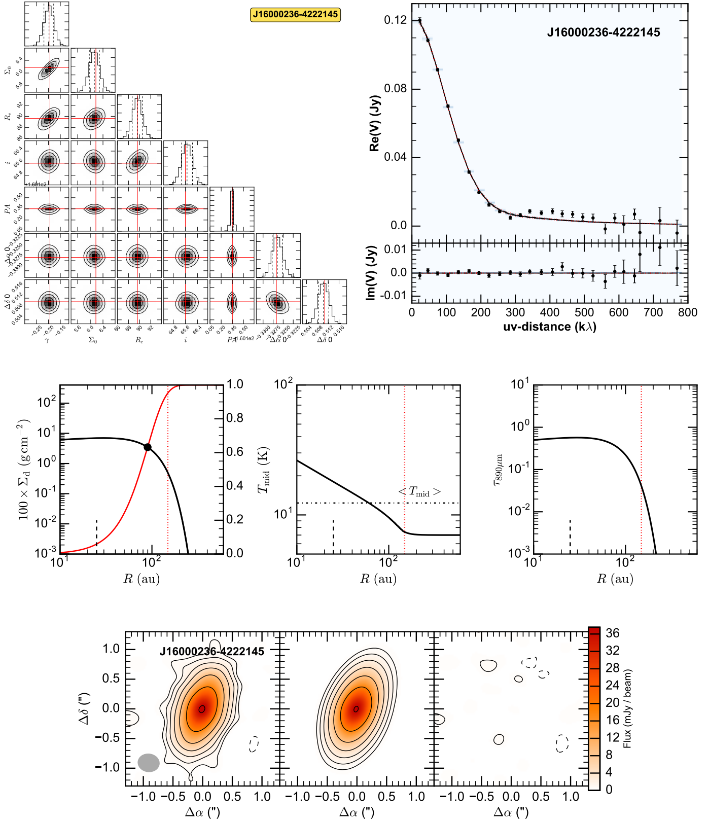
Fig. A.11. Fit results for J16000236-4222145, presented as in Fig. A.1. In the images \sigma = 0.25 mJy/beam.
