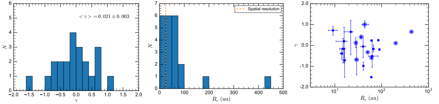
Fig. 9. Distribution of surface density slopes \gamma (left), exponential cut-off radii R_c (center) and the correlation between them (right) derived for the disks in the sample. The vertical dashed line in the top and middle panels gives a visual representation of the spatial resolution of the observations, estimated as half of the synthesized beam size (in our case \sim 25 au at a distance of 150 pc). There is no apparent correlation between \gamma and R_c .
