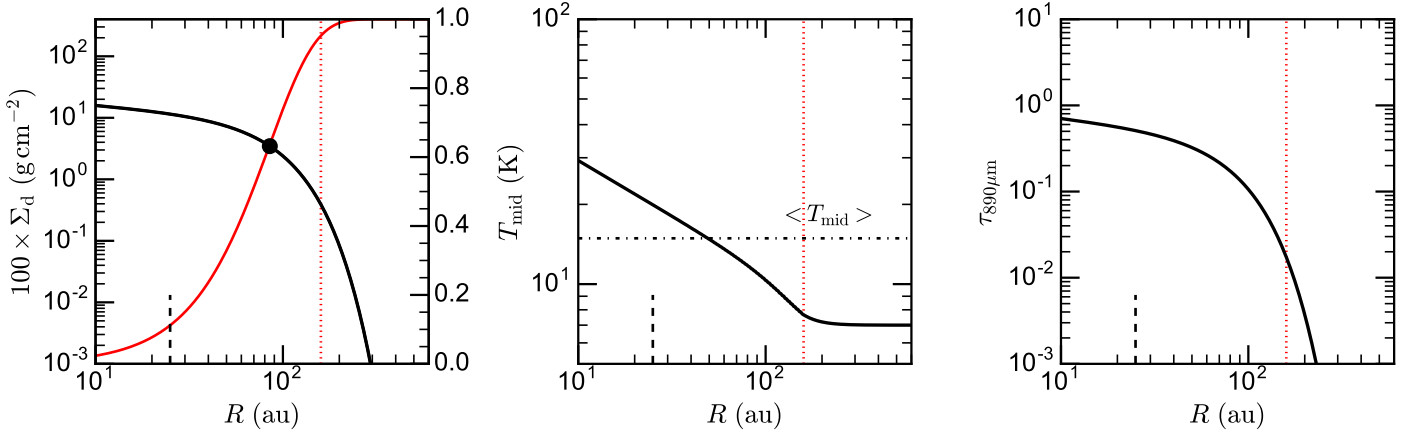
Fig. 4. Physical structure of the best-fit model describing Sz 71. Left: gas surface density profile computed as 100 \times \Sigma_d(R) , where 100 is the gas-to-dust ratio. The solid red line is the cumulative mass (right y axis) and the black filled circle highlights the cut-off radius R_c \approx 85 au. In all three plots, the dotted red line indicates the radius containing 95% of mass and the vertical dashed black line half the synthesized beam size ( \approx 25 ) au. Middle: dust temperature profile T_{\text{mid}}(R) derived self-consistently at each radius from the disk model. The dot-dashed horizontal line represents the mass-averaged dust temperature \langle T_{\text{mid}} \rangle , which for Sz 71 is \approx 14 K. Right: optical depth of the disk midplane at the observing wavelength: the sub-mm continuum emission is expected to be optically thick only within R < 2 au.
