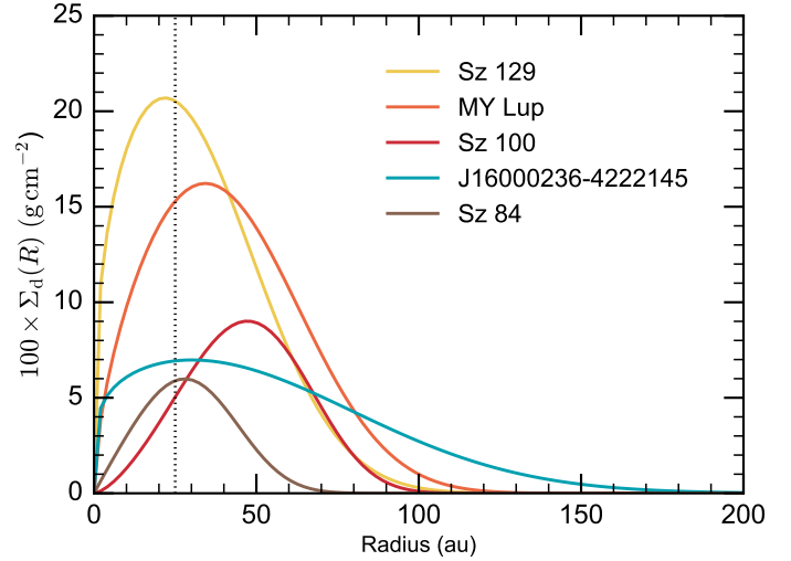
Fig. 10. Surface density profiles of the five disks having \gamma < 0 at a significance level larger than 3\sigma . The vertical dashed line gives a visual representation of half the beam size (25 au at 150 pc).
