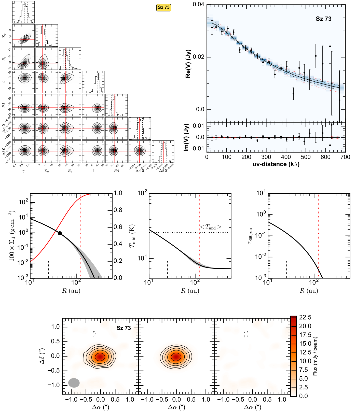
Fig. A.6. Fit results for Sz 73, presented as in Fig. A.1. In the images \sigma = 0.33 mJy/beam.
