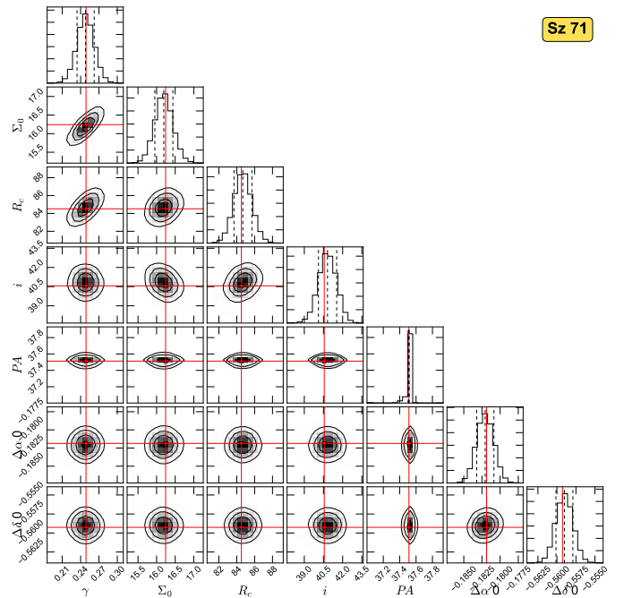
Fig. 3. Staircase plot of the chain resulting from the MCMC fit of Sz 71. The histograms on the main diagonal are the marginalized distributions of each parameter: from left to right, \gamma , \Sigma_0 , R_c , i and PA, \Delta\alpha , \Delta\delta . The vertical dashed lines indicate the 16%, 50% and 84% percentiles. The off-diagonal 2D plots show the correlation between each couple of parameter, with contour lines showing 0.5\sigma increments. The solid red lines highlight the coordinates of the best-fit model.
