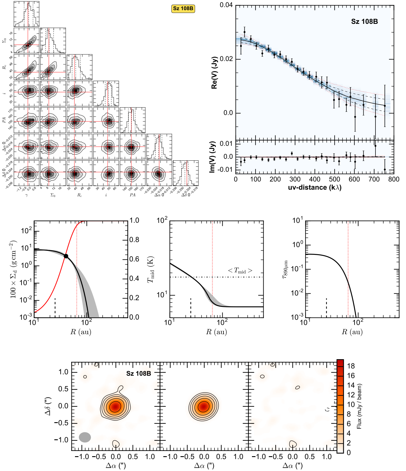
Fig. A.17. Fit results for Sz 108B, presented as in Fig. A.1. In the images \sigma = 0.25 mJy/beam.
