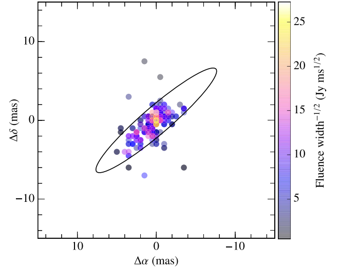
Figure 4. Pulse localizations from the pulsar B0525+21 observed on 2016 February 11 at 1.7 GHz. A total of 406 pulses were imaged. Systematic uncertainties inversely proportional to the detection statistic \xi are observed. We note that only pulses with \xi \gtrsim 5 Jy ms ^{1/2} are robustly localized to within the FWHM, and for pulses with \xi \sim 0.5 – 1 Jy ms ^{1/2} the scatter can be closer to 10 mas.
