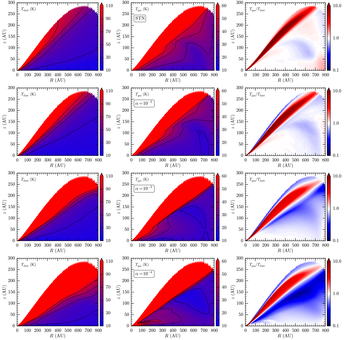
Fig. A.2. From top to bottom: STN, \alpha = 10^{-2} , 10^{-3} , and 10^{-4} models. From left to right: dust temperature T_{\text{dust}} , gas temperature T_{\text{gas}} , and ratio of the two.
