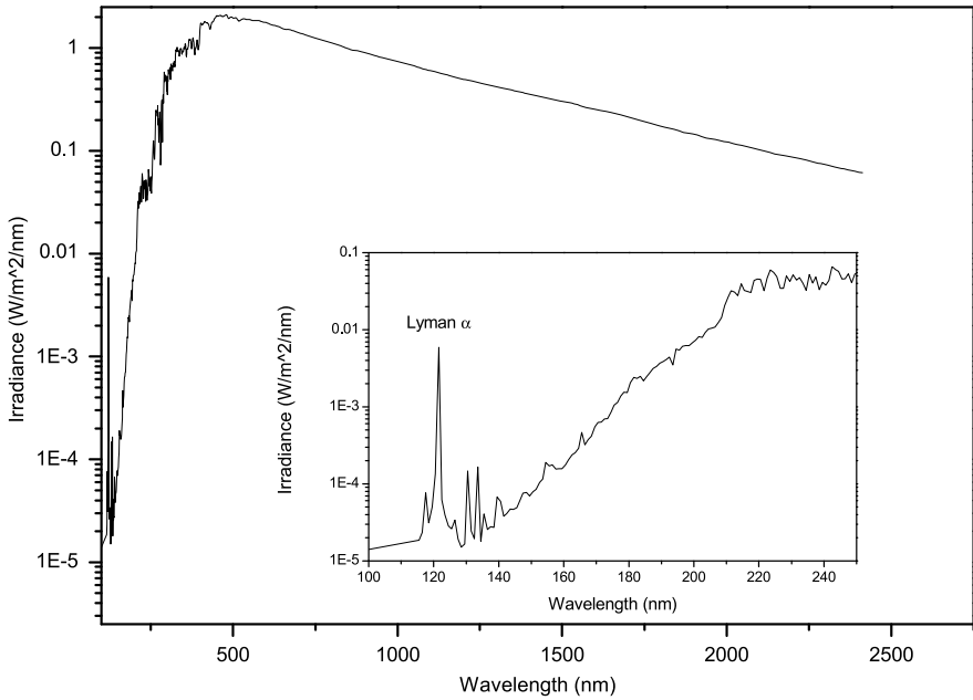
Fig. 2 Irradiance spectrum of the Sun from 100 to 2500 nm. (From the Sorce web database, http://lasp.colorado.edu/lisird/sorce/ )
