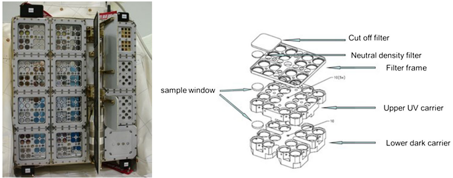
Fig. 40 EXPOSE-E integrated on the EuTEF platform before launch (Credit: ESA). The bottom two compartments and the lower half of next compartments contained the sample carriers (explosion drawing on the right, adapted, credit: Kayser-Threde) with the sample from ADAPT. Left vertical row is tray 1, open to space; middle vertical row is tray 2 with Mars conditions
