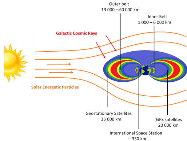
Fig. 5 Earth's particle environment (dominated by galactic cosmic rays and solar particles) and the two main radiation (Van Allen) belts around the Earth
