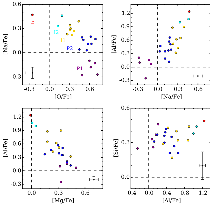
Figure 8. [O/Fe] , [Na/Fe] , [Mg/Fe] , [Al/Fe] , and [Si/Fe] plotted against each other to illustrate the O–Na/Mg–Al anticorrelations and Na–Al/Al–Si correlations present in NGC 5986. The [Na/Fe] vs. [O/Fe] plot in particular suggests that approximately five distinct populations with different light-element chemistries may exist. We have labeled and color-coded the “primordial” ( P1 ; P2 ), “intermediate” ( I1 ; I2 ), and “extreme” ( E ) groups based on the nomenclature used in Carretta (2015) for NGC 2808. The existence of an Al–Si correlation suggests that the gas from which the more Al-rich stars formed was processed at temperatures \gtrsim 65 MK.
