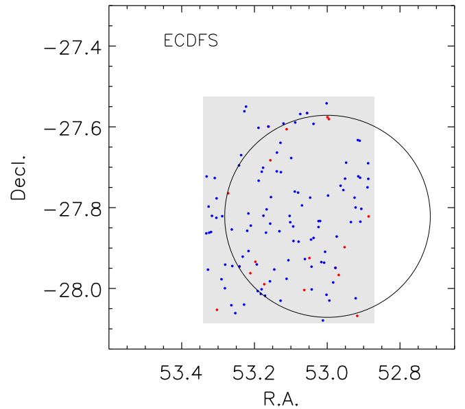
Figure 3. ECDFS field. The field consists of one Suprime-Cam pointing (gray area). The large circle indicates the M2FS pointing. We have to move the pointing center far away from the field center to find a suitable SH star. The red and blue points represent LAE and LBG candidates, respectively.
