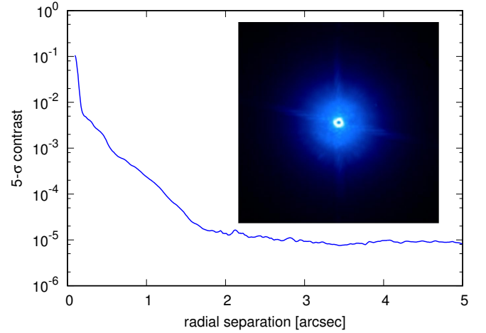
Fig. 3. 5\sigma flux contrast curve as a function of separation from K2-111. The inset displays the combined saturated H -band image of the target acquired with HiCIAO. The field-of-view is 4'' \times 4'' . North is up and east is left.
