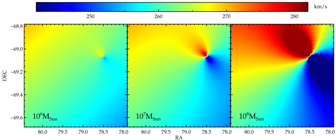
Figure 7. Models of the LMC velocity field with 10^6 M_\odot , 10^7 M_\odot , and 10^8 M_\odot black holes, over the area surrounding the kinematic center implied by previous measurements. In these plots, the black hole was placed at the kinematic center, but its position was varied in our model fits.
