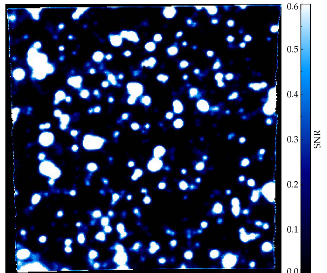
Figure 2. Signal-to-noise map of a typical MUSE field. The area of this field is one arcmin 2 .
