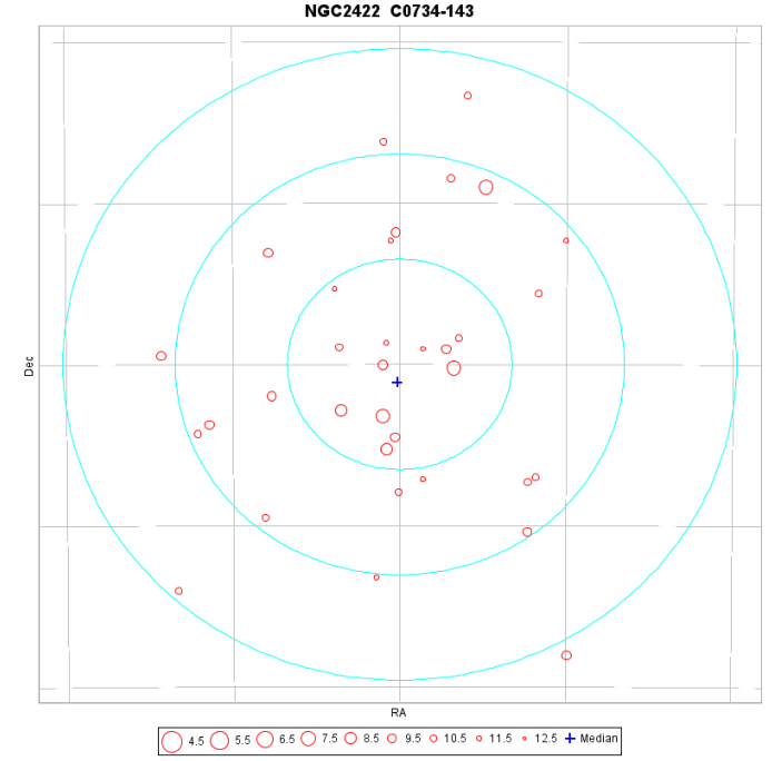
Fig. D.34. A map of members of the cluster NGC 2422 as identified from the TGAS catalogue. The coordinate grid is at 1 degrees intervals, the three concentric circles are at 5, 10 and 15 pc from the cluster centre at the cluster distance.
