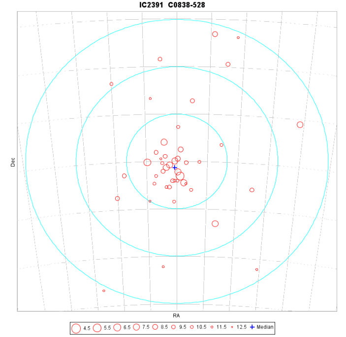
Fig. D.12. A map of members of the cluster IC 2391 as identified from the TGAS catalogue. The coordinate grid is at 2 degrees intervals, the three concentric circles are at 5, 10 and 15 pc from the cluster centre at the cluster distance.
