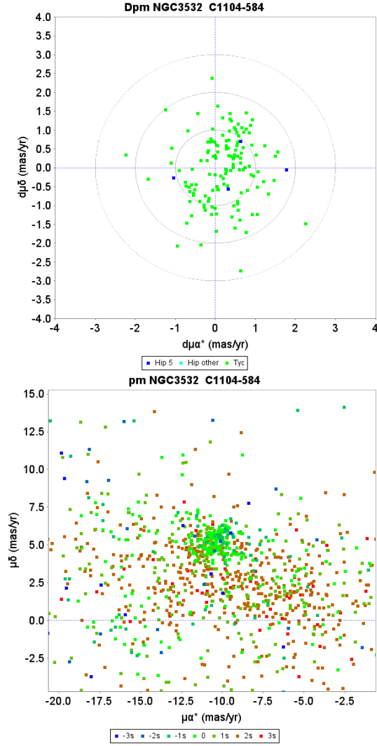
Fig. D.35. Proper motion charts for the cluster NGC 3532. Top : unit weight residual proper motions. Green dots have first epoch Tycho -2 data, the dark blue dots have HIPPARCOS first epoch 5-parameter solutions. The concentric circles represent 1-3\sigma su levels. Bottom : actual proper motion distribution, where the colour indicate the difference from the cluster parallax in su units.
