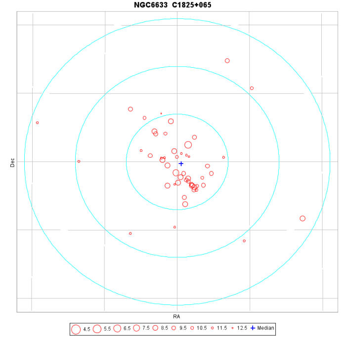
Fig. D.30. A map of members of the cluster NGC 6633 as identified from the TGAS catalogue. The coordinate grid is at 1 degrees intervals, the three concentric circles are at 5, 10 and 15 pc from the cluster centre at the cluster distance.
