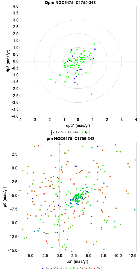
Fig. D.19. Proper motion charts for the cluster NGC 6475. Top : unit weight residual proper motions. Green dots have first epoch Tycho -2 data, the dark blue dots have HIPPARCOS first epoch 5-parameter solutions. The concentric circles represent 1-3\sigma su levels. Bottom : actual proper motion distribution, where the colour indicate the difference from the cluster parallax in su units.
