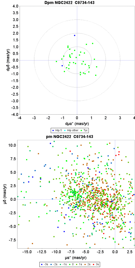
Fig. D.33. Proper motion charts for the cluster NGC 2422. Top : unit weight residual proper motions. Green dots have first epoch Tycho -2 data, the dark blue dots have HIPPARCOS first epoch 5-parameter solutions. The concentric circles represent 1-3\sigma su levels. Bottom : actual proper motion distribution, where the colour indicate the difference from the cluster parallax in su units.
