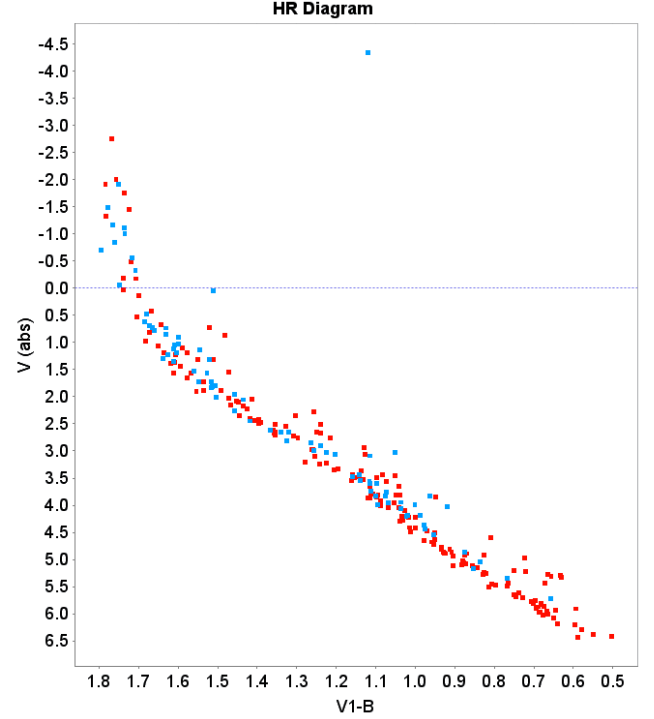
Fig. 27. Geneva photometry HR diagram for the \alpha Per cluster (blue dots) compared with the data on the Pleiades cluster (red dots). Red-densifying corrections were applied for both clusters. Geneva photometry.
