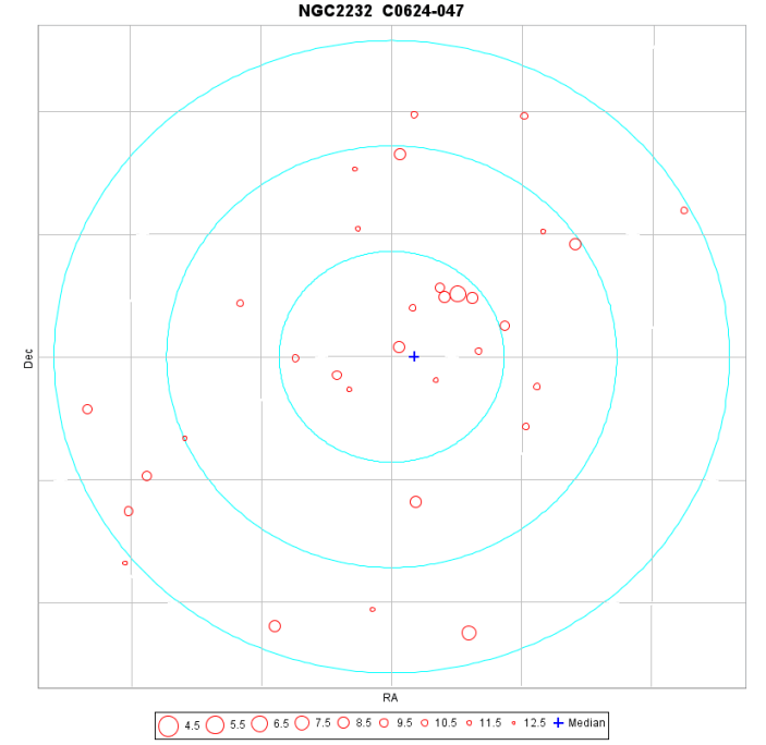
Fig. D.26. A map of members of the cluster NGC 2232 as identified from the TGAS catalogue. The coordinate grid is at 1 degrees intervals, the three concentric circles are at 5, 10 and 15 pc from the cluster centre at the cluster distance.
