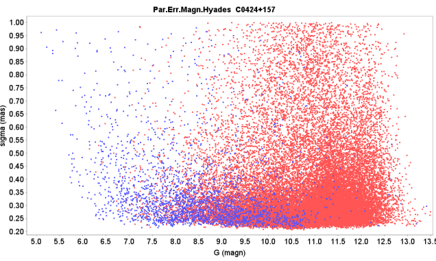
Fig. 7. Standard uncertainties for parallax measurements in TGAS, as a function of the G magnitude, for stars in a field of 18 degrees radius centred on the Hyades cluster. The red and blue points as in Fig. 1.
