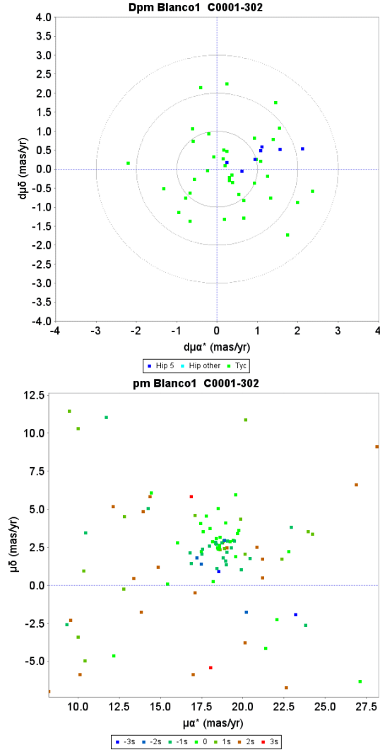
Fig. D.15. Proper motion charts for the cluster Blanco 1. Top : unit weight residual proper motions. Green dots have first epoch Tycho -2 data, the dark blue dots have HIPPARCOS first epoch 5-parameter solutions. The concentric circles represent 1-3\sigma su levels. Bottom : actual proper motion distribution, where the colour indicate the difference from the cluster parallax in su units.
