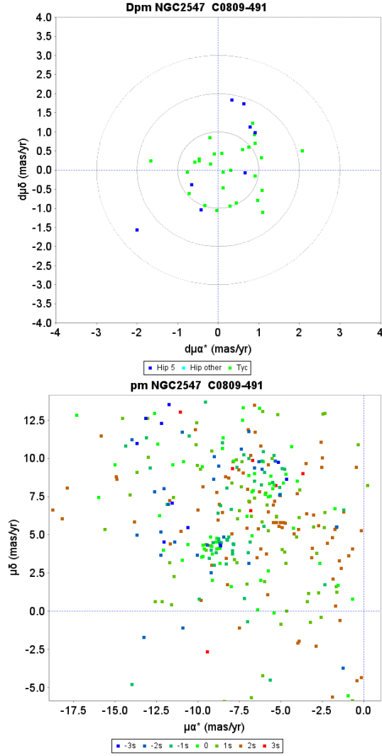
Fig. D.37. Proper motion charts for the cluster NGC 2547. Top : unit weight residual proper motions. Green dots have first epoch Tycho -2 data, the dark blue dots have HIPPARCOS first epoch 5-parameter solutions. The concentric circles represent 1-3\sigma su levels. Bottom : actual proper motion distribution, where the colour indicate the difference from the cluster parallax in su units.
