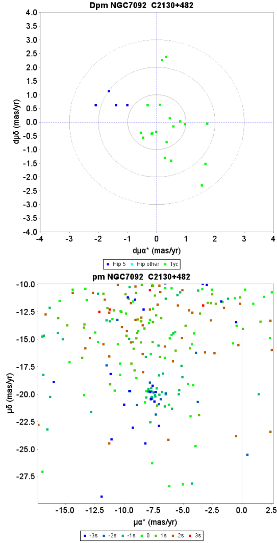
Fig. D.21. Proper motion charts for the cluster NGC 7092. Top : unit weight residual proper motions. Green dots have first epoch Tycho -2 data, the dark blue dots have HIPPARCOS first epoch 5-parameter solutions. The concentric circles represent 1–3 \sigma su levels. Bottom : actual proper motion distribution, where the colour indicate the difference from the cluster parallax in su units.
