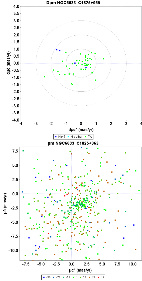
Fig. D.29. Proper motion charts for the cluster NGC 6633. Top : unit weight residual proper motions. Green dots have first epoch Tycho -2 data, the dark blue dots have HIPPARCOS first epoch 5-parameter solutions. The concentric circles represent 1-3\sigma su levels. Bottom : actual proper motion distribution, where the colour indicate the difference from the cluster parallax in su units.
