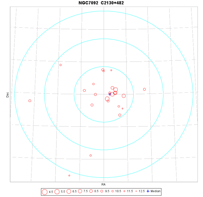
Fig. D.22. A map of members of the cluster NGC 7092 as identified from the TGAS catalogue. The coordinate grid is at 1 degrees intervals, the three concentric circles are at 5, 10 and 15 pc from the cluster centre at the cluster distance.
