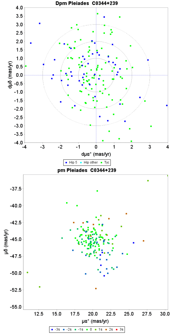
Fig. D.5. Proper motion charts for the Pleiades cluster. Top : unit weight residual proper motions. Green dots have first epoch Tycho-2 data, the dark blue dots have HIPPARCOS first epoch 5-parameter solutions. The concentric circles represent 1-3\sigma su levels. Bottom : actual proper motion distribution, where the colour indicate the difference from the cluster parallax in su units.
