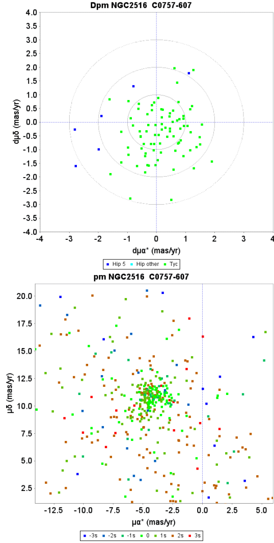
Fig. D.23. Proper motion charts for the cluster NGC 2516. Top : unit weight residual proper motions. Green dots have first epoch Tycho -2 data, the dark blue dots have HIPPARCOS first epoch 5-parameter solutions. The concentric circles represent 1-3\sigma su levels. Bottom : actual proper motion distribution, where the colour indicate the difference from the cluster parallax in su units.
