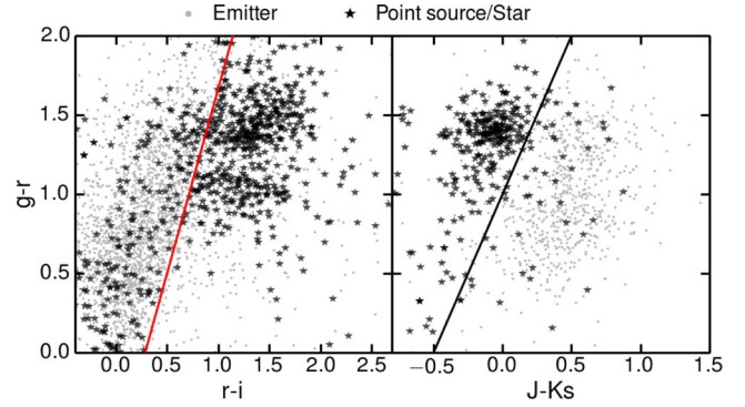
Figure 4. Colour–colour plots for emitters. The left plot displays the g - r colour versus r - i . The right plot represents g - r versus J - Ks . Point-like objects are represented with stars, while emitters are shown in grey dots. The lines show the colour cuts used to select point-like objects, in combination with other criteria as discussed in Section 4.2.
