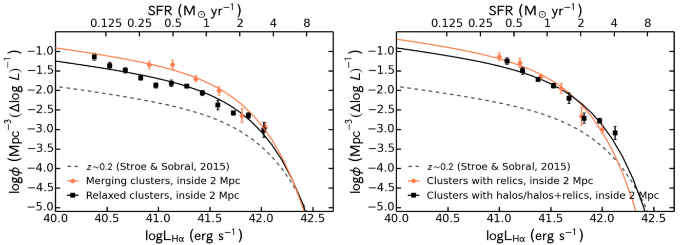
Figure 9. Left-hand panel: the H \alpha LF for merging and relaxed clusters (within 2 Mpc of centre). Note the differences in normalization of the two LFs. Right-hand panel: the H \alpha LF for clusters hosting relics and haloes, respectively (within 2 Mpc of centre). The presence of shocks mildly boosts the number of H \alpha emitters compared to a cluster hosting a halo.
