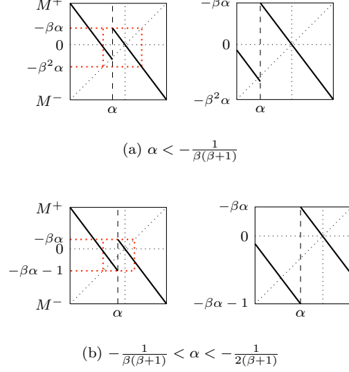
Figure 2: Two choices of \alpha for the same \beta that give different forward invariant sets. For both (a) and (b), the map on the right is the map on the left restricted to this forward invariant set.
