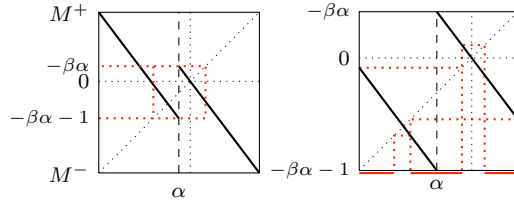
(c) A map from Example 6
