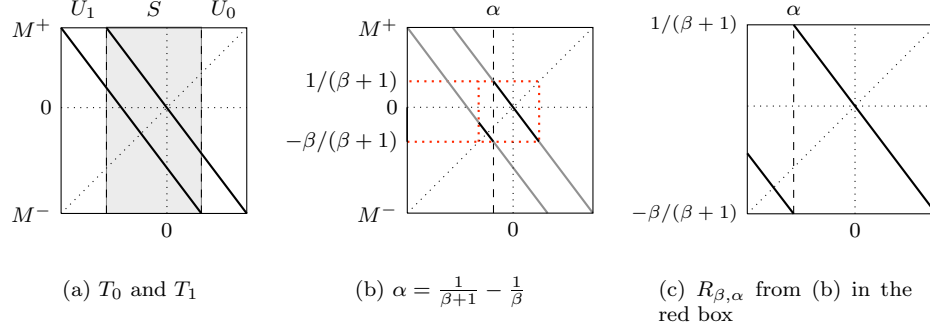
Figure 1: In (a) we see the full maps T_0 and T_1 and in (b) we see the map R_{\beta, \alpha} with \alpha = \frac{1}{\beta+1} - \frac{1}{\beta} , the choice from [7]. In (c) we see this transformation on the interval [-\frac{\beta}{\beta+1}, \frac{1}{\beta+1}] .
