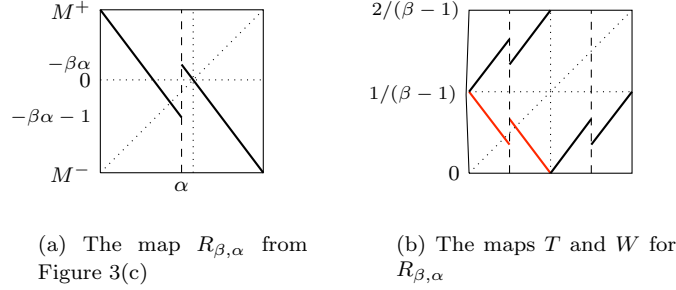
Figure 4: The maps T and W for a map R_{\beta, \alpha} . In (b), the red lines indicate the map T and the black lines the map W .
