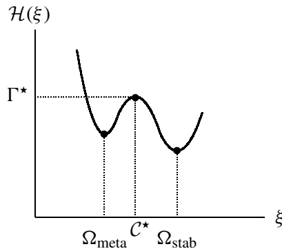
FIG. 2. Schematic picture of \mathcal{H} , \Omega_{\text{meta}} , \Omega_{\text{stab}} and C^* .
