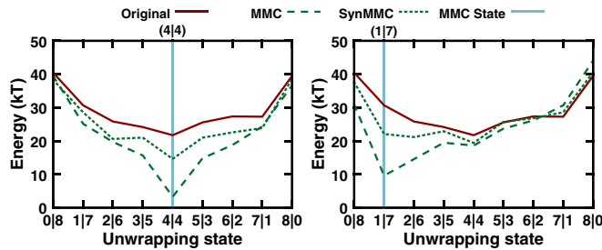
FIG. 2. Energy along the ridge for sequences found using MMC on position 826 of the YAL002W gene of S. cerevisiae , held in unwrapping states (4|4) (left) and (1|7) (right). The solid line represents the original ridge. The dashed line is the ridge after free MMC and the dotted line after SynMMC.
