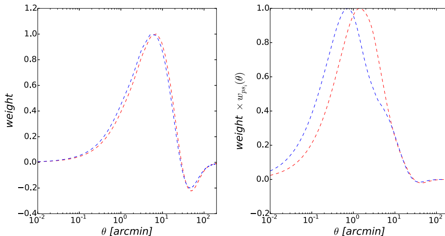
Figure 3. The weights D_i(\theta) defined in Section 5.4 (left-hand panel) and the combination D_i(\theta) \times w_{\text{psi}}(\theta) (right-hand panel) for the mock catalogue tests. The weights and correlation functions are derived for the z = 0.225 (blue) and z = 0.525 (red) redshift bins, for illustration. The combination D_i(\theta) \times w_{\text{psi}}(\theta) represents the angular scales used by the estimator to measure the redshift probability distribution, in accordance with equation (27).
