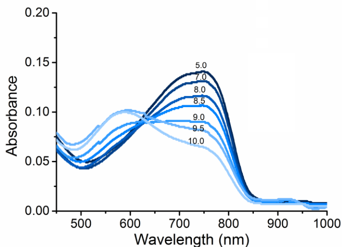
Figure A.6: Absorbance spectra of His-tag purified PR-DNFS:MMAR in DDM solution at pH 5, 7, 8, 8.5, 9, 9.5, 10. pH values are indicated next to the corresponding spectrum in the graph. Spectra represent separate samples, not a titration of a single sample.
