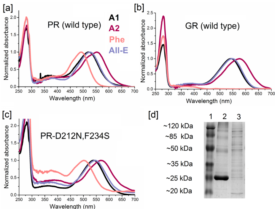
Figure 2.3 Absorbance spectra of purified analog pigments of [a] PR [b] GR and [c] PR-DNFS. No specific peak around 500 nm was obtained for GR with PHE. Spectra are taken at pH 8. Accuracy of the \lambda_{\text{max}} values \pm 2 nm. A1 (black), A2 (magenta), ALL-E (violet) and PHE (pink). [d] Coomassie Blue stained SDS-PAGE gel. The lanes contain (1) protein ladder (2) fraction with purified PR (3) membrane vesicles containing PR. The strong band in lane-2 at ~25 kDa corresponds to the PR monomer.
