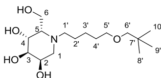
Figure 19: Proton and carbon NMR numbering of iminosugars
