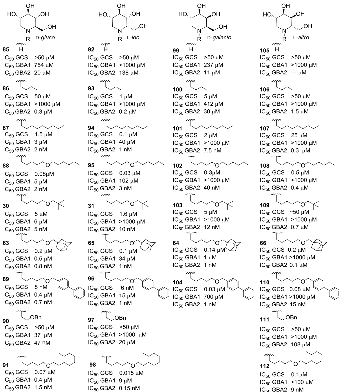
Figure 12: IC_{50} values of DNJ derivatives with 2S, 3R configuration
