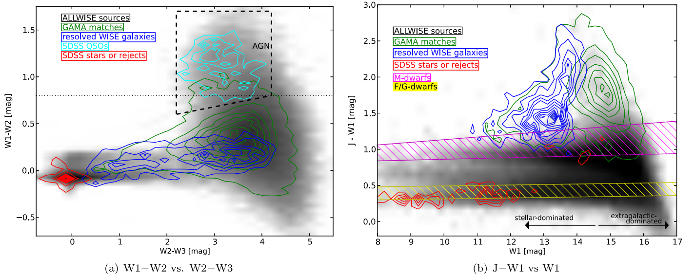
Figure 6. The power of colors: (a) W1-W2 vs. W2-W3 , and (b) near-infrared J-W1 colors. See Figure 5 for a description of the contouring. The AGN box is from Jarrett et al. (2011). Note that the J-W1 color is limited by the 2MASS J-band sensitivity; hence, only the bright W1 sources are shown. The expected track for main-sequence M dwarfs is shown with the magenta shading and the brighter F/G dwarfs with the yellow shading. K dwarfs are located between these two tracks.
