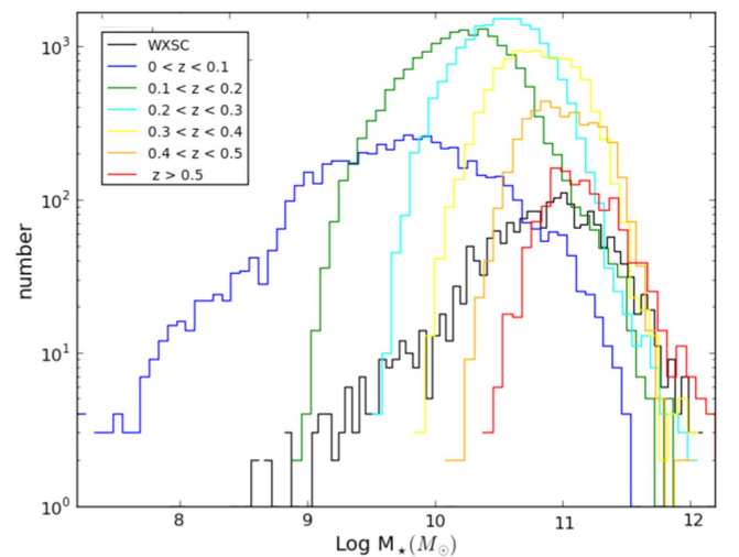
Figure 12. Stellar mass distribution in redshift shells. The lowest mass galaxies detected in GAMA, M_* < 10^9 M_\odot , are only seen at low redshifts ( z < 0.1 ) because of the faint surface brightness, while the highest mass galaxies, > 10^{11} M_\odot , are seen well beyond the local Universe. For the redshift where GAMA is relatively complete, z < 0.3 , the mass distribution peaks around > 10^{10.5} M_\odot .
