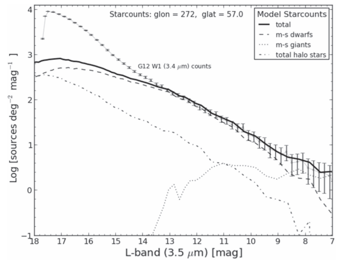
Figure 4. Expected L-band ( 3.5\ \mu\text{m} ) star counts for the direction of the sky that contains the G12 field, which is the polar cap region. For comparison, the ALLWISE W1 ( 3.4\ \mu\text{m} ) counts are indicated (with Poisson error bars) and connected using a faint gray line. Stars dominate the source counts for W1 < 13.5 mag ( 1.2\ \text{mJy} ). We assume a negligible difference between L band ( 3.5\ \mu\text{m} ) and W1 ( 3.4\ \mu\text{m} ).
