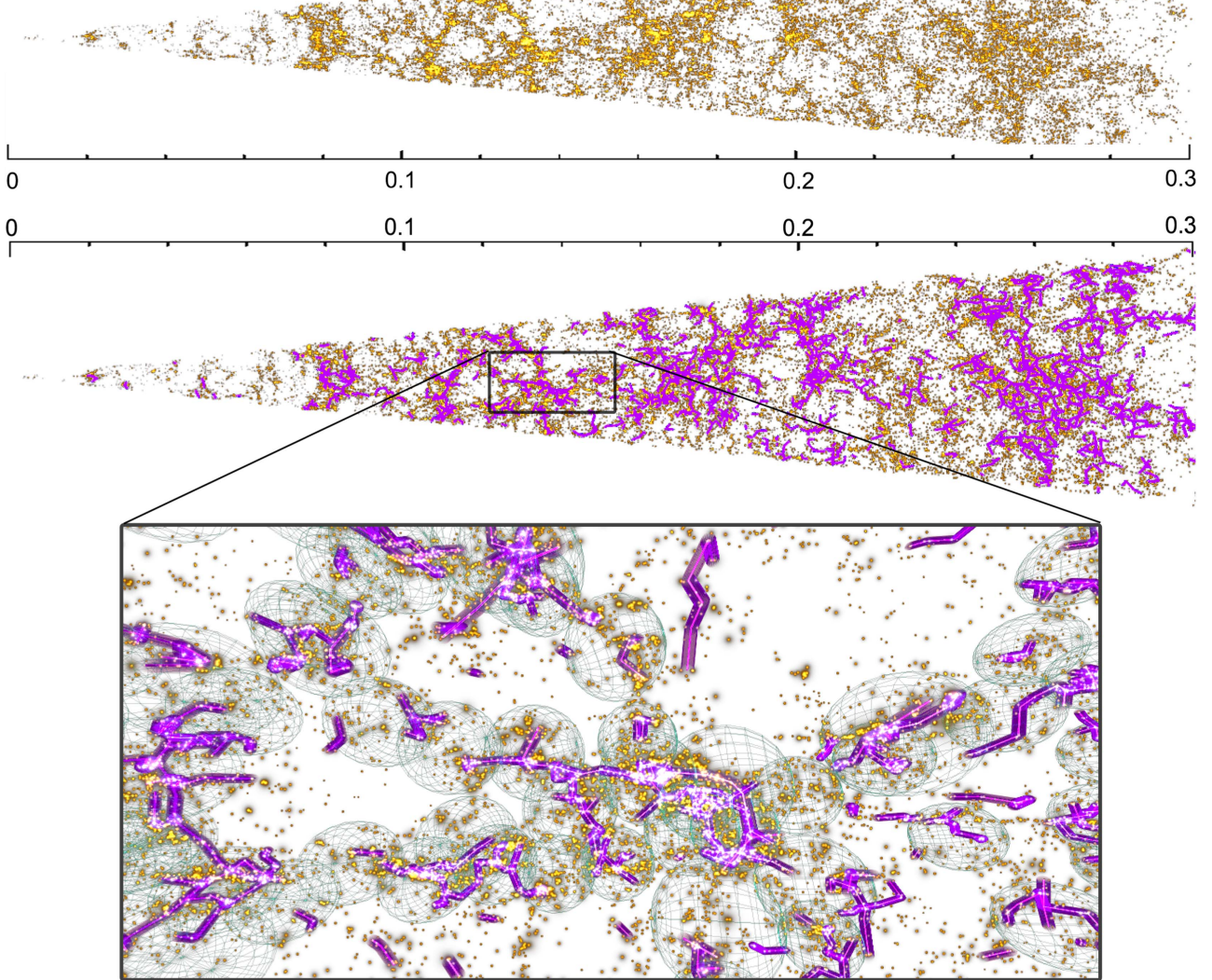
Figure 20. WISE -GAMA galaxies in G12, displayed using a 3D cone that extends to a redshift of 0.3, or a luminosity distance of 1564 Mpc (1200 Mpc in comoving frame), and a total comoving volume of 0.011 \text{ Gpc}^3 . The lower panel shows the same view, but with the GAMA galaxy groups filament catalog (Alpaslan et al. 2015) overlaid in magenta, illustrating the underlying “skeleton” of the web of galaxies. The inset image shows a zoomed view of an overdensity region near z \sim 0.14 to gain a better view of the 3D distribution of filaments and clusters. The green spheres are the overdense regions determined in a 20 Mpc diameter region (see Table 3 and Figure 15). The graphics were made using the Partview visualization system.
