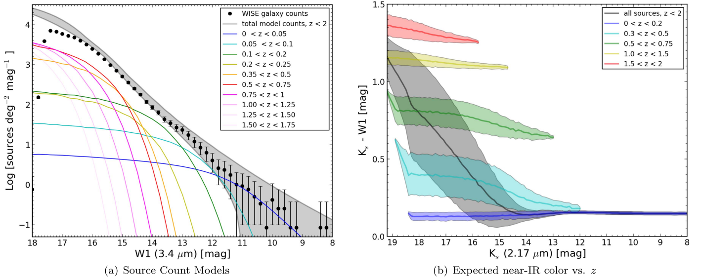
Figure 8. Modeling the extragalactic source counts. (a) Expected extragalactic source counts: differential source counts in comparison to the measured WISE values (solid filled points), highlighting a series of redshift shells. The shaded curve represents the spread in values using a mixture of k -corrections and two different infrared LFs of Dai et al. (2009). (b) The expected near-infrared K -W1 color as a function of the apparent K -band (Vega) magnitude for the extragalactic population; the gray shaded region corresponds to all redshifts (up to 2); the other shadings represent redshift shells and demonstrate the significant band-shifting differences between 2.2\ \mu\text{m} and 3.4\ \mu\text{m} at redshifts >0.2 .
