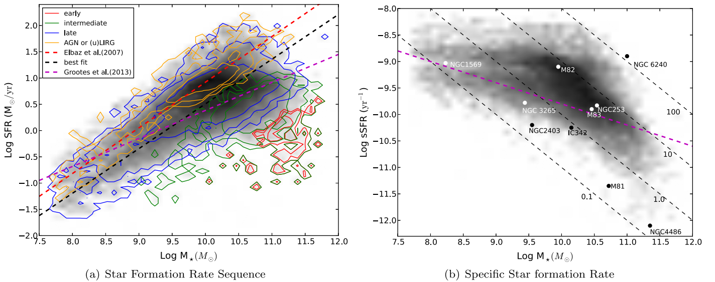
Figure 13. Star formation rate (SFR) relative to the host stellar mass, M_{*} ( M_{\odot} ). The gray scale represents all sources with z < 0.3 , including photometric redshifts. The left panel (a) shows how the rate changes with mass, delineated by WISE color: early, intermediate, late and AGN and infrared-luminous types. The black dashed line represents the average “sequence” for the sample, the red dashed line plots the relation at high redshift (Elbaz et al. 2007), and the dashed magenta line is for a nearby GALEX-GAMA sample (Grootes et al. 2013). The right panel (b) shows the equivalent sSFR distribution, with dashed lines representing lines of constant SFR (0.1, 1, 10, and 100 M_{\odot} \text{ yr}^{-1} ), and the magenta dashed line shows the relation from GALEX-GAMA . For comparison, a few nearby galaxies values are indicated, from massive spheroidal (NGC4486; M87) to star-forming (NGC 253) spirals and starbursts (M82), and to dwarfs (NGC1569).
