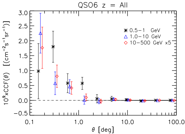
Figure 9. Same as the left panel of Figure 7 but for the cross-correlation of the full SDSS DR6 QSO sample with Fermi -LAT P8 data.
