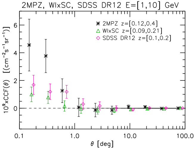
Figure 17. CCF of Fermi -LAT data in the energy range 1–10 GeV with 2MPZ galaxies for z \in [0.12, 0.4] , W1xSC galaxies for z \in [0.09, 0.21] , and SDSS DR12 galaxies for z \in [0.1, 0.2] . Note that, due to the decreasing redshift tail of 2MPZ, the range z \in [0.12, 0.2] contains basically almost all of the galaxies of z \in [0.12, 0.4] .
